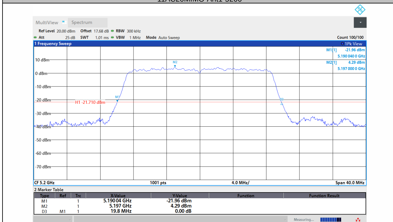
11AC20MIMO-Ant2-5200
