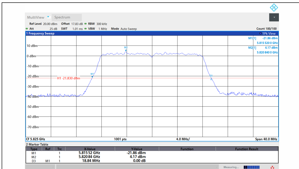
11A-Ant1-5825
