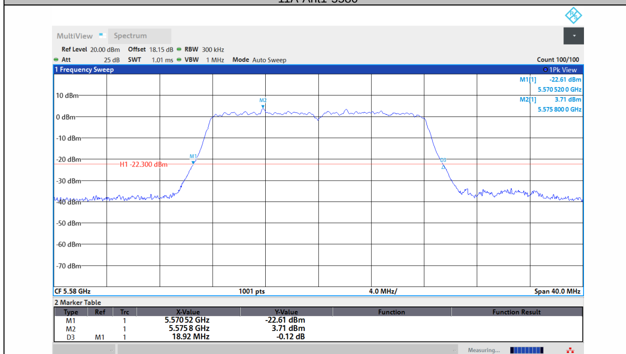
11A-Ant2-5580
