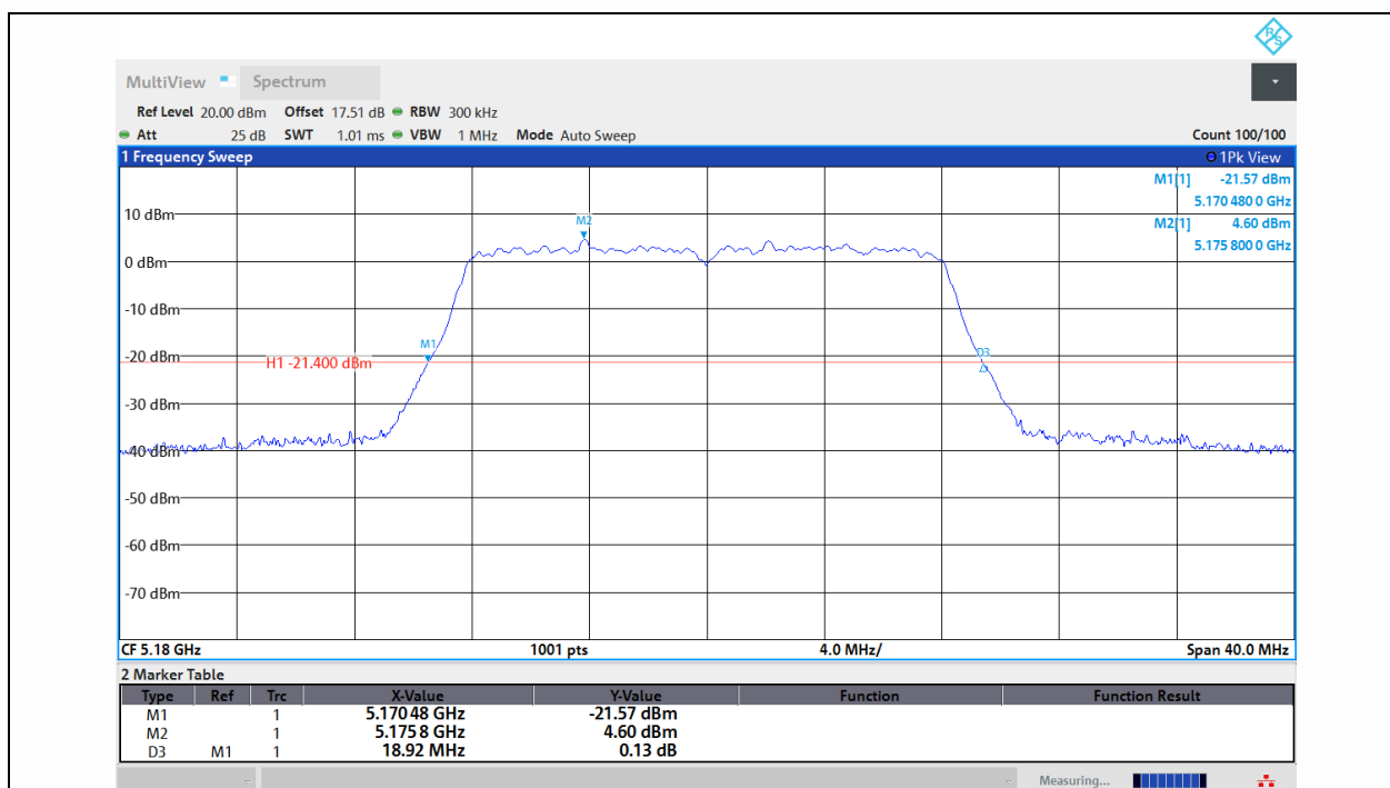
11A-Ant1-5180
