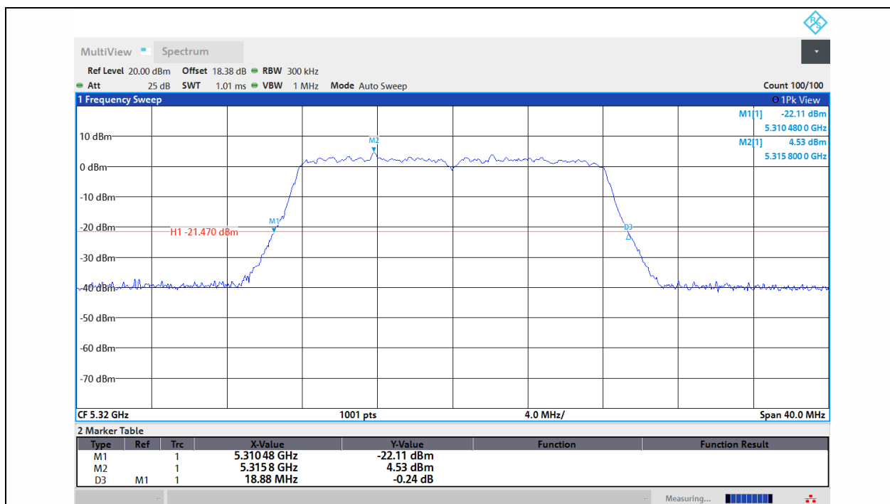
11A-Ant1-5320
