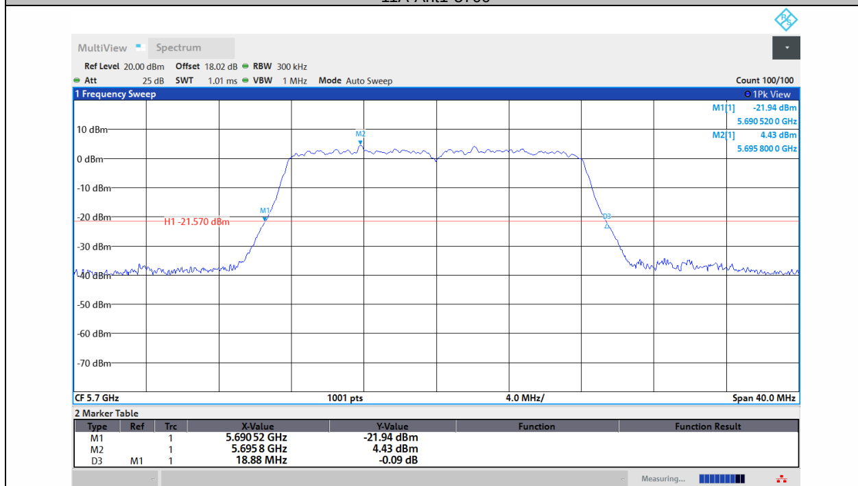
11A-Ant2-5700
