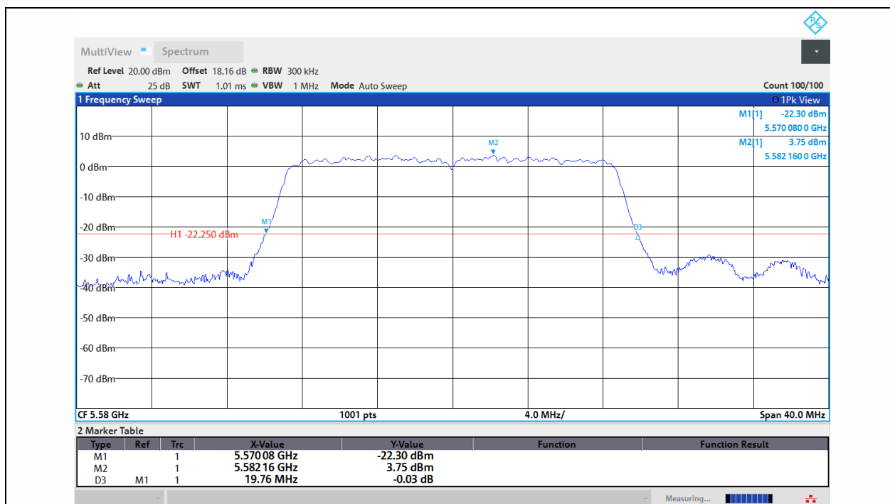
11AC20MIMO-Ant1-5580
