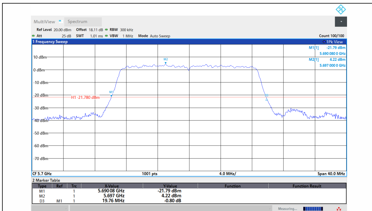
11AC20MIMO-Ant1-5700
