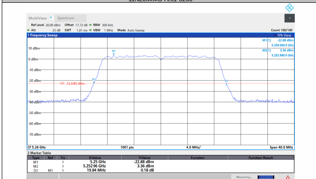
11N20MIMO-Ant2-5260
