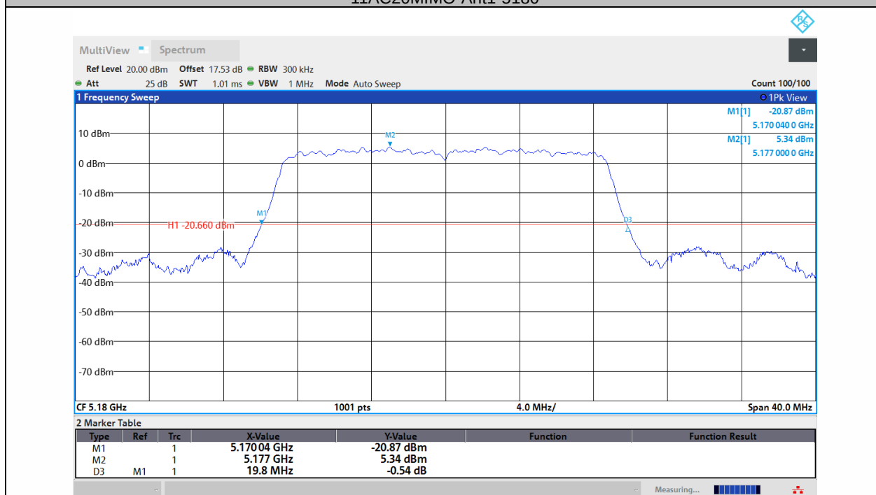
11AC20MIMO-Ant2-5180
