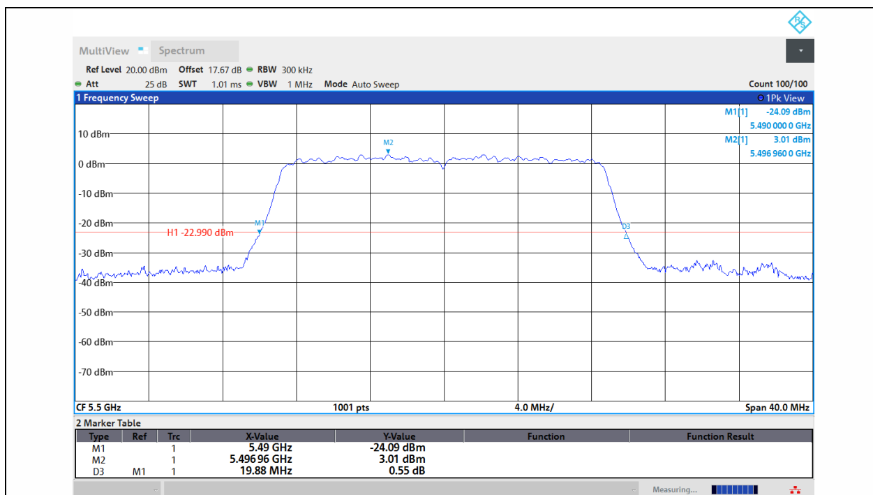
11AC20MIMO-Ant1-5500
