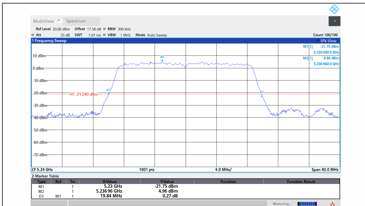
11AC20MIMO-Ant1-5240
