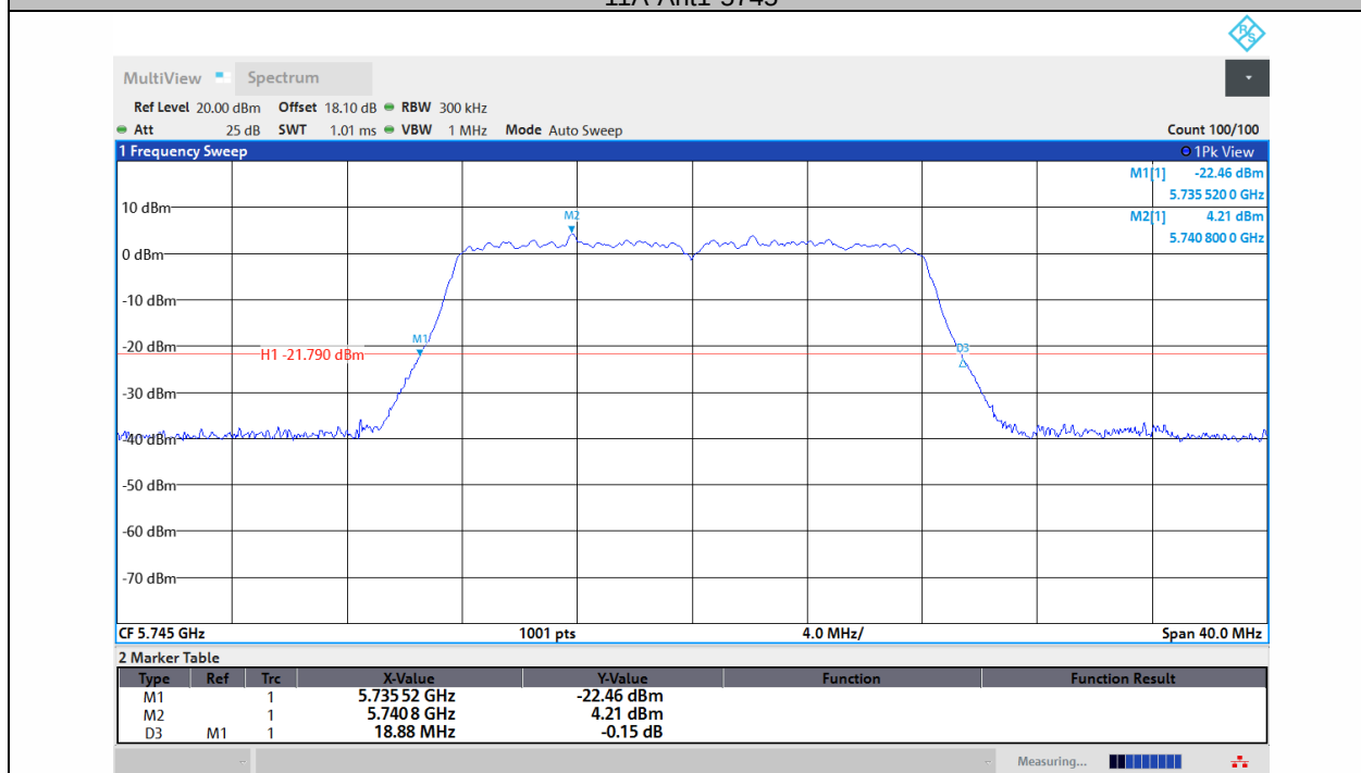
11A-Ant2-5745
