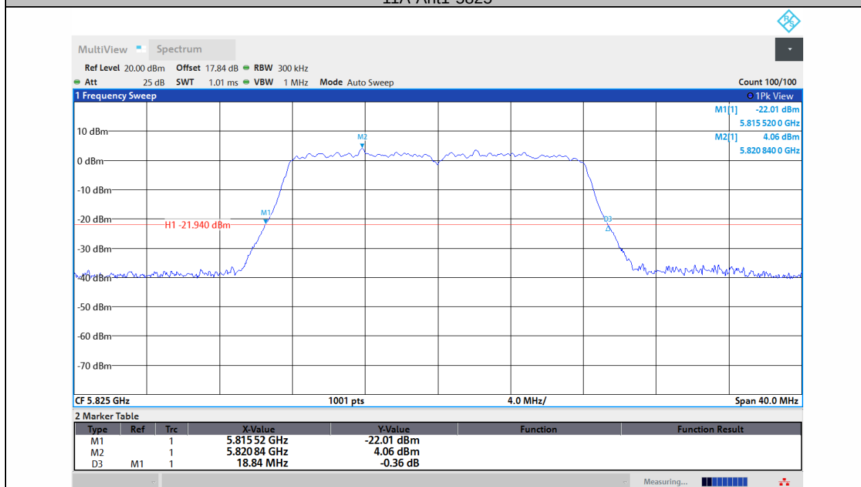
11A-Ant2-5825
