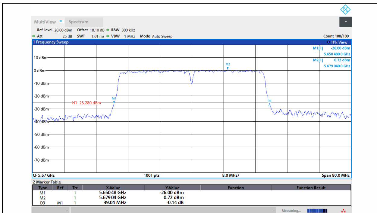
11N40MIMO-Ant1-5670
