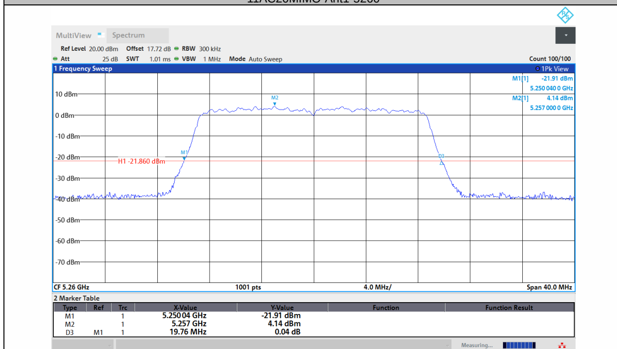
11AC20MIMO-Ant2-5260
