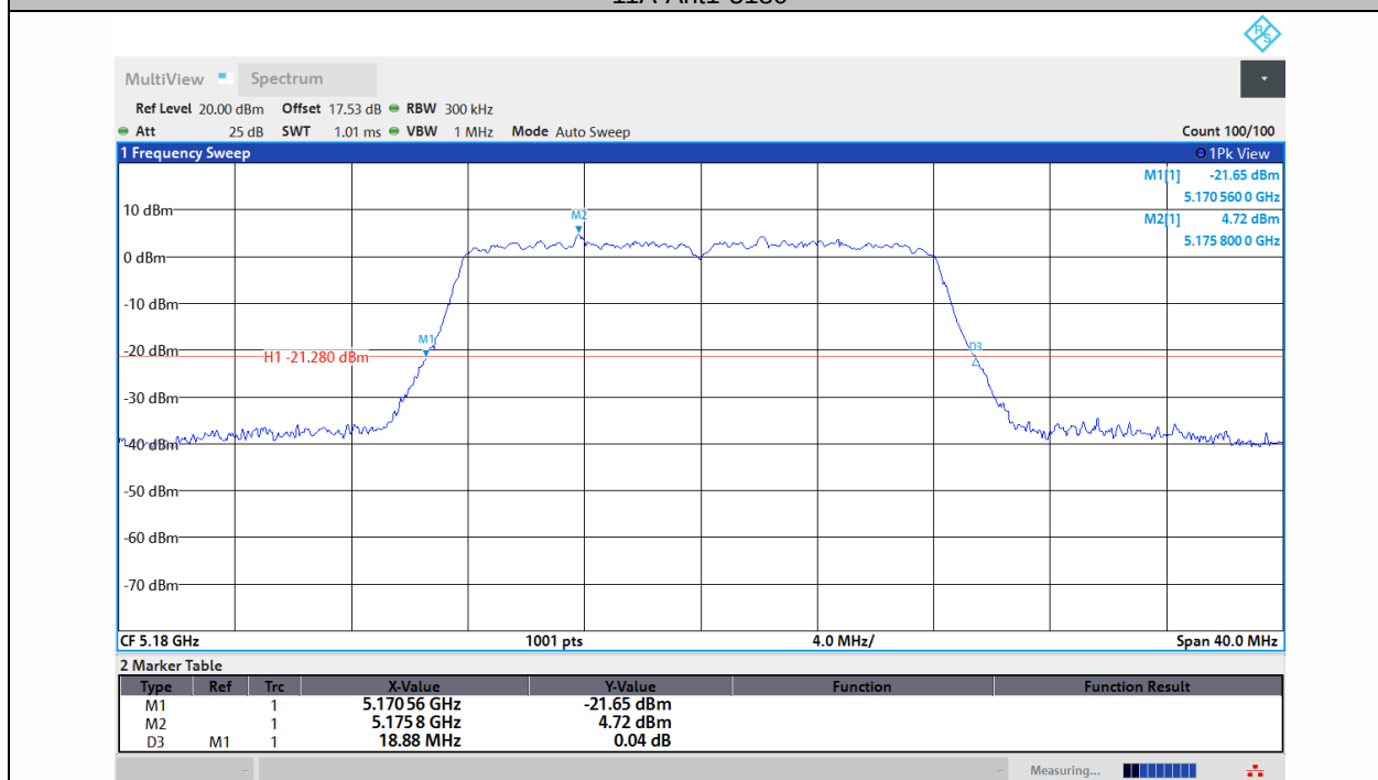
11A-Ant2-5180
