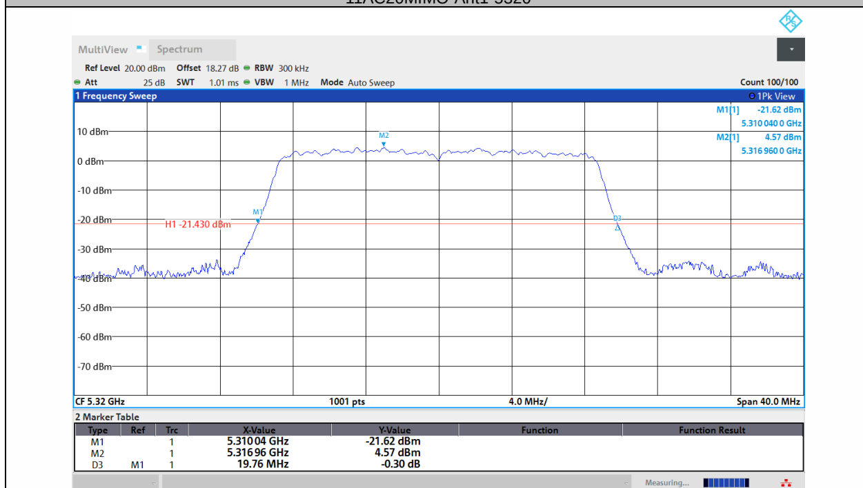
11AC20MIMO-Ant2-5320
