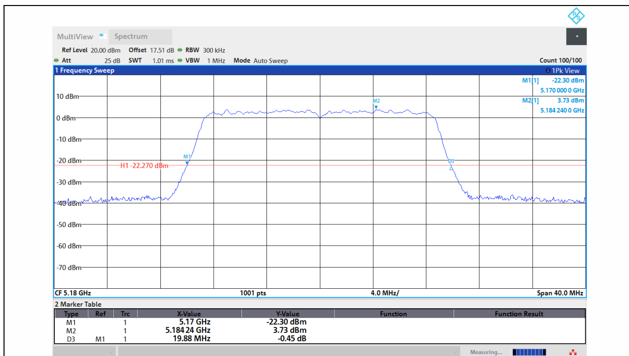
11N20MIMO-Ant1-5180
