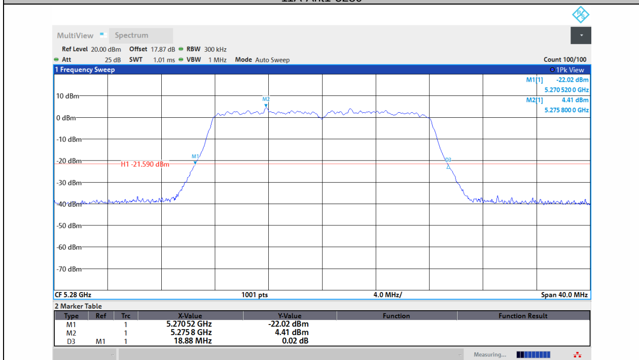
11A-Ant2-5280
