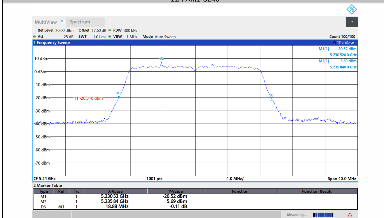
11A-Ant2-5240
