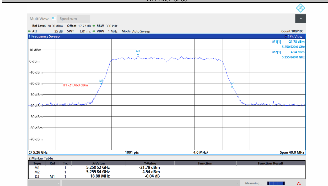
11A-Ant2-5260
