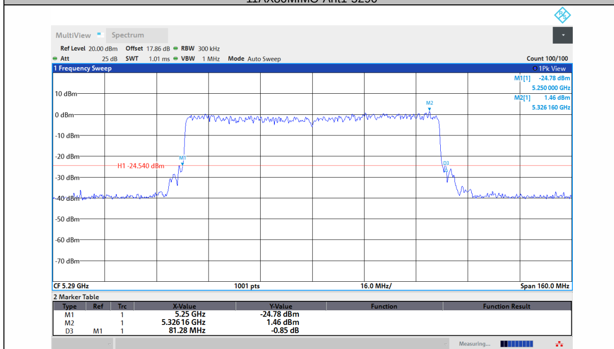
11AX80MIMO-Ant2-5290
