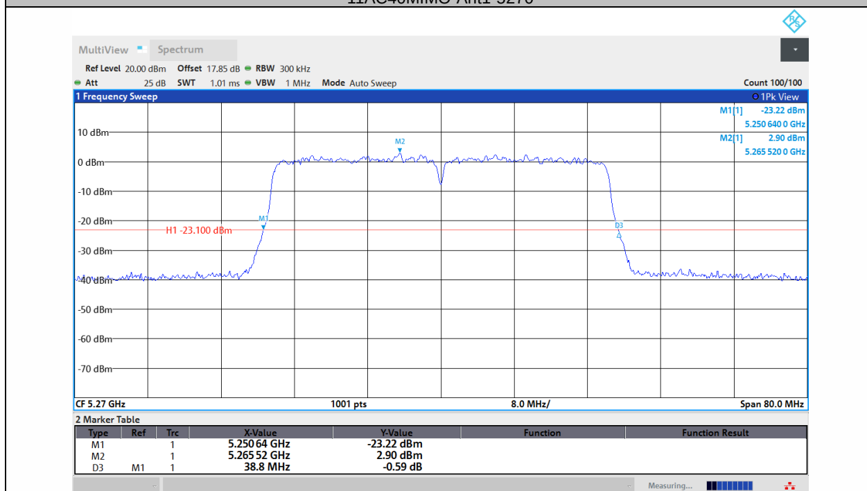
11AC40MIMO-Ant2-5270
