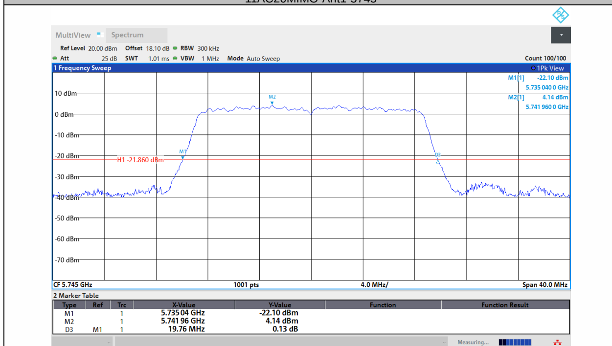
11AC20MIMO-Ant2-5745
