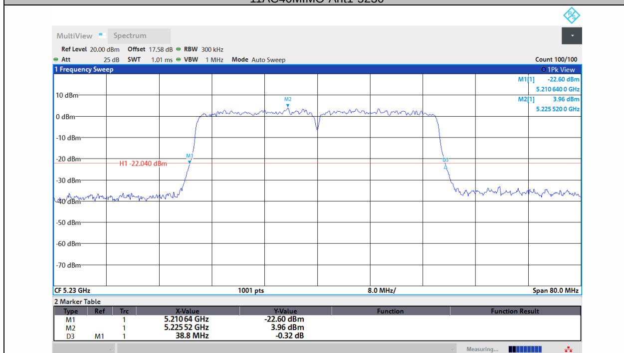
11AC40MIMO-Ant2-5230
