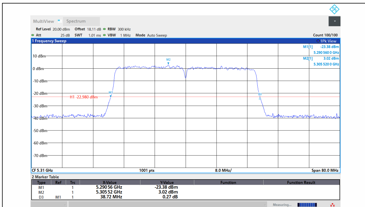
11AC40MIMO-Ant1-5310
