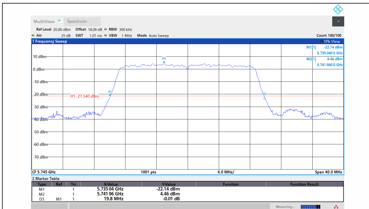
11AC20MIMO-Ant1-5745
