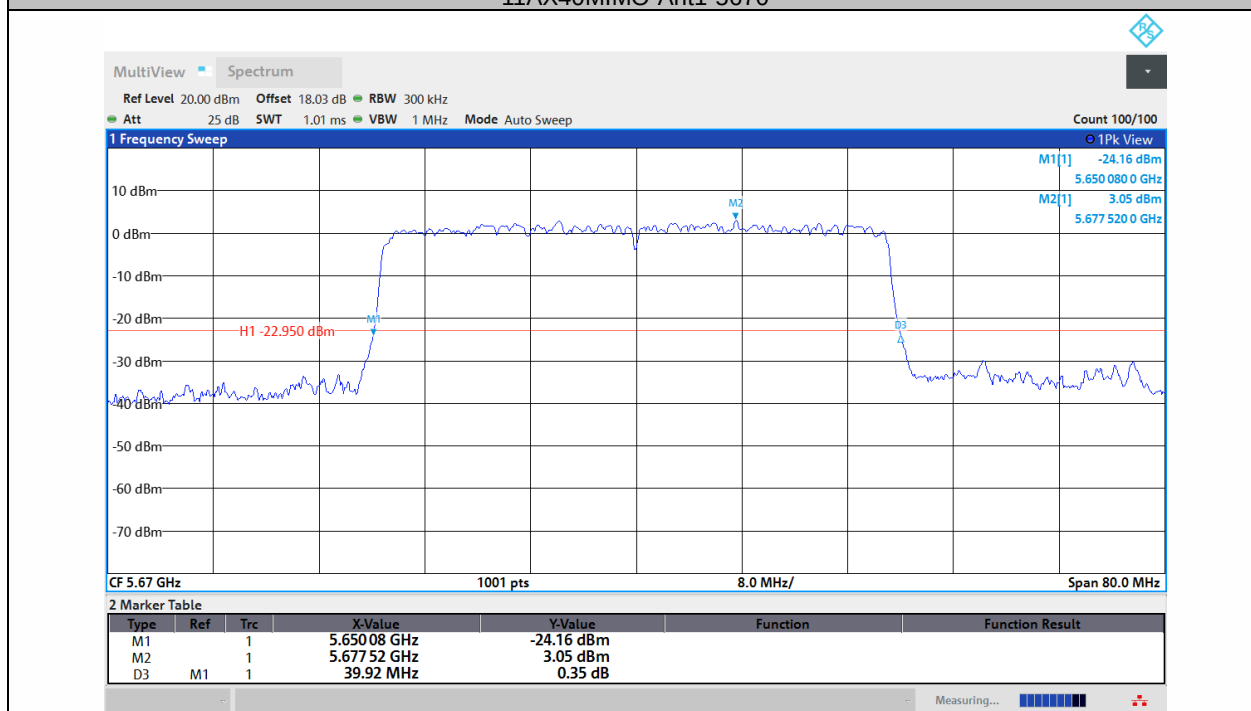
11AX40MIMO-Ant2-5670
