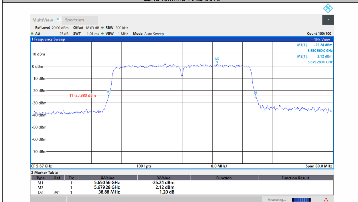
11AC40MIMO-Ant2-5670
