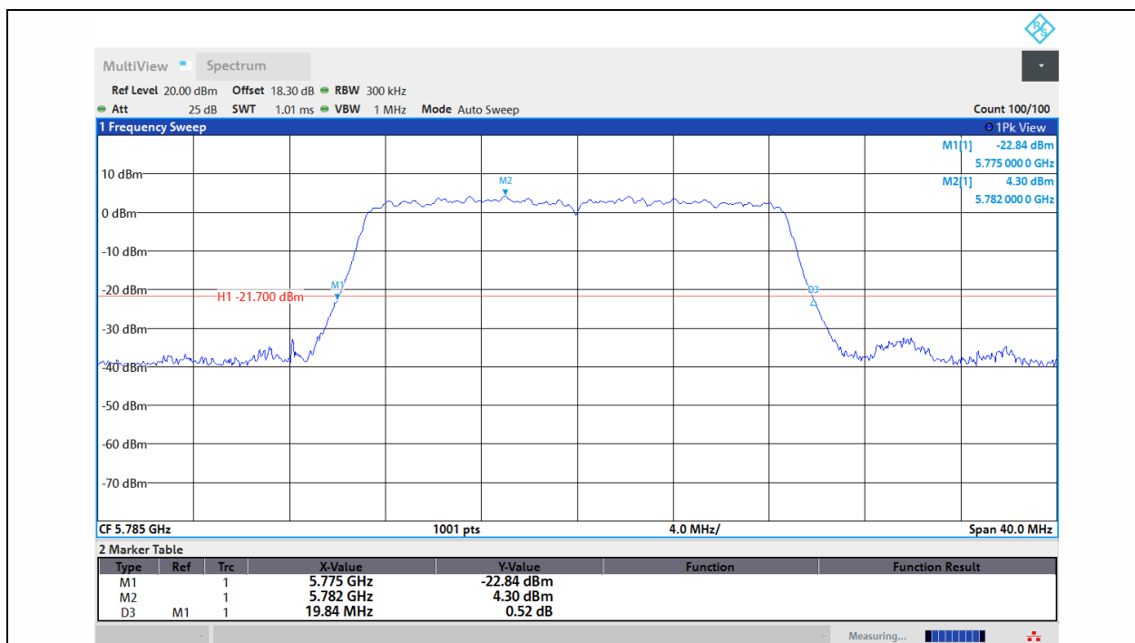
11AC20MIMO-Ant1-5785
