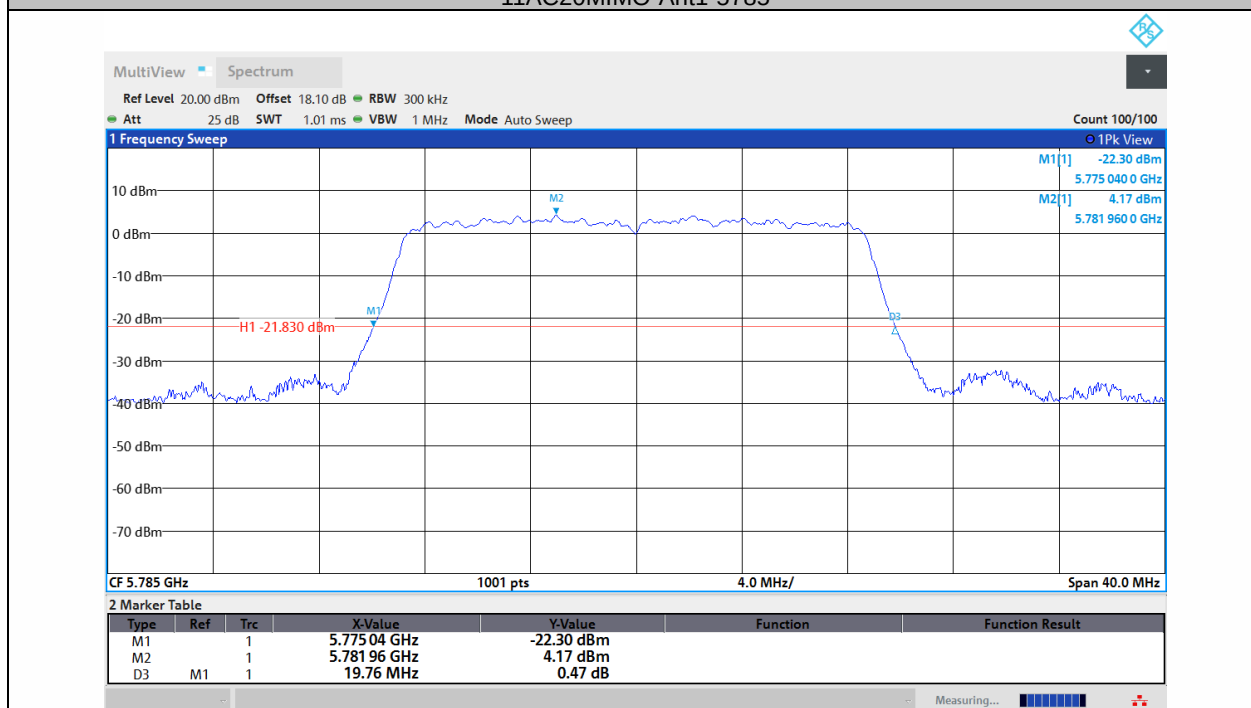
11AC20MIMO-Ant2-5785
