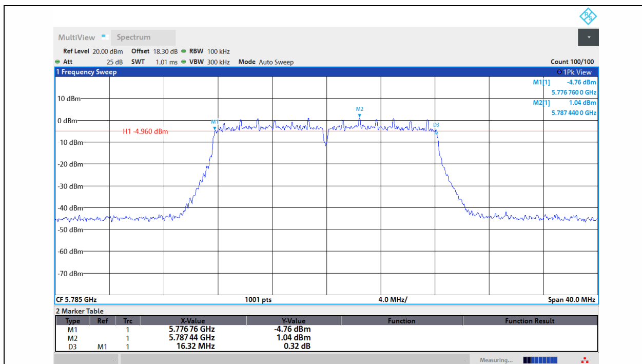
11A-Ant1-5785-PASS
