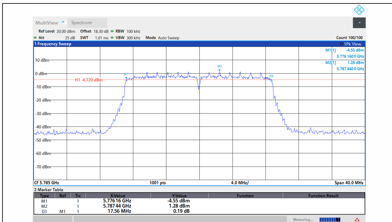
11AC20MIMO-Ant1-5785-PASS
