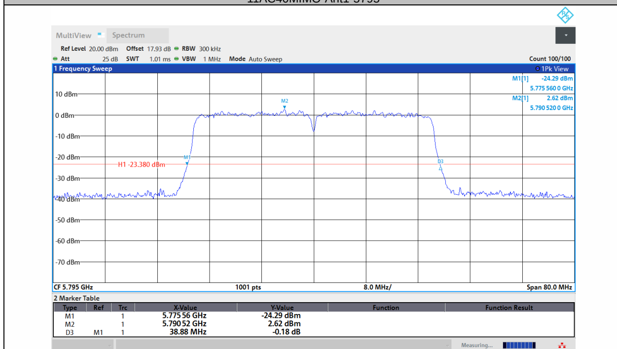
11AC40MIMO-Ant2-5795
