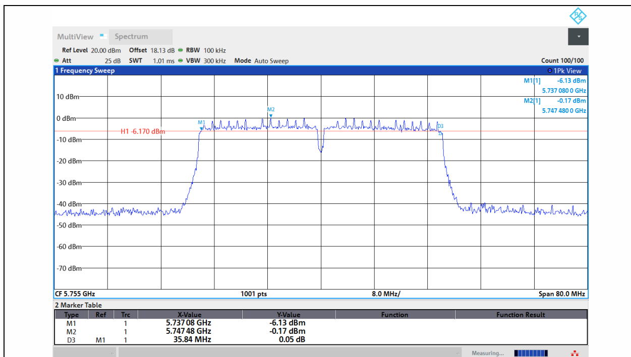
11AC40MIMO-Ant1-5755-PASS
