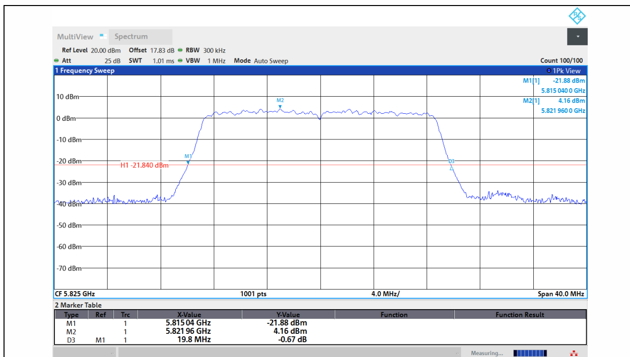
11AC20MIMO-Ant1-5825
