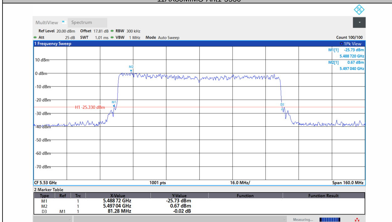
11AX80MIMO-Ant2-5530
