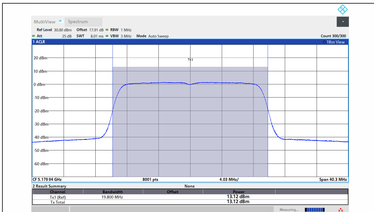
11AC20MIMO-Ant1-5180-PASS
