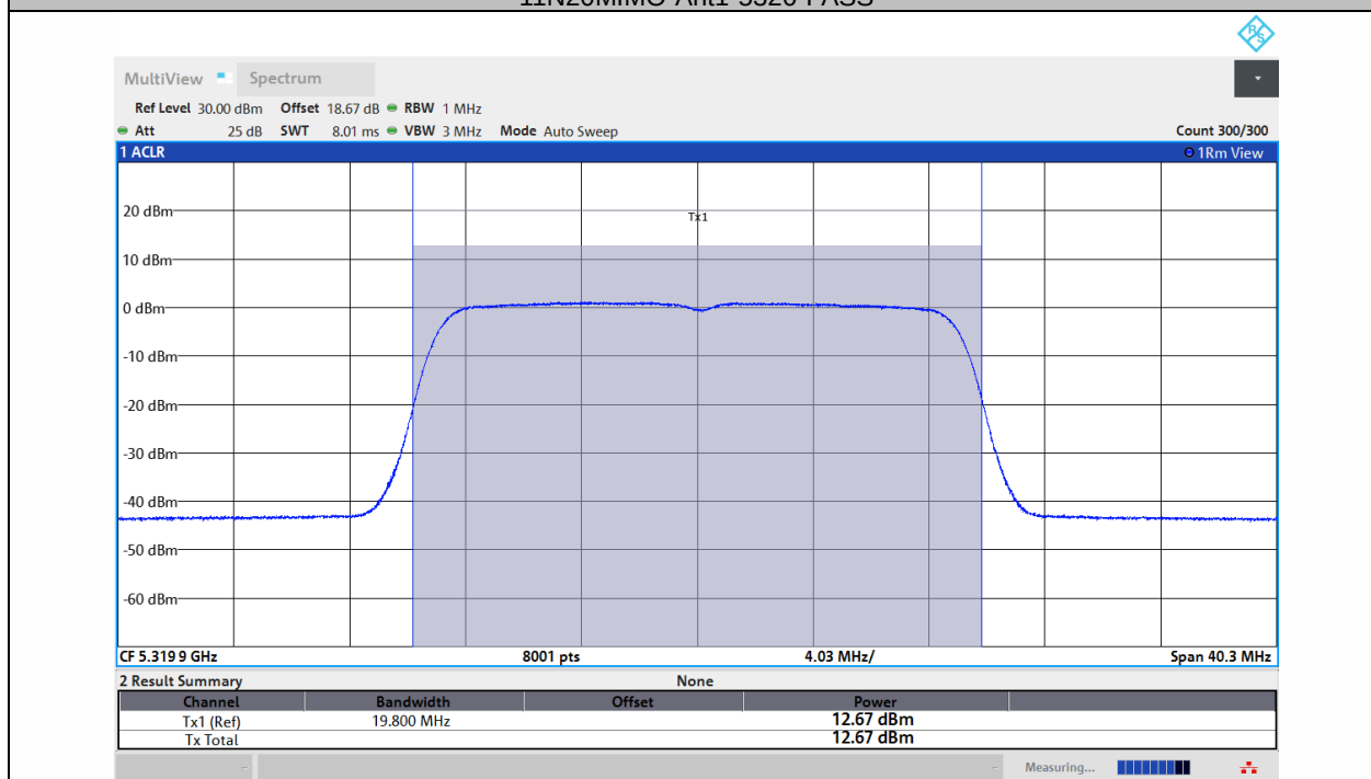
11N20MIMO-Ant2-5320-PASS
