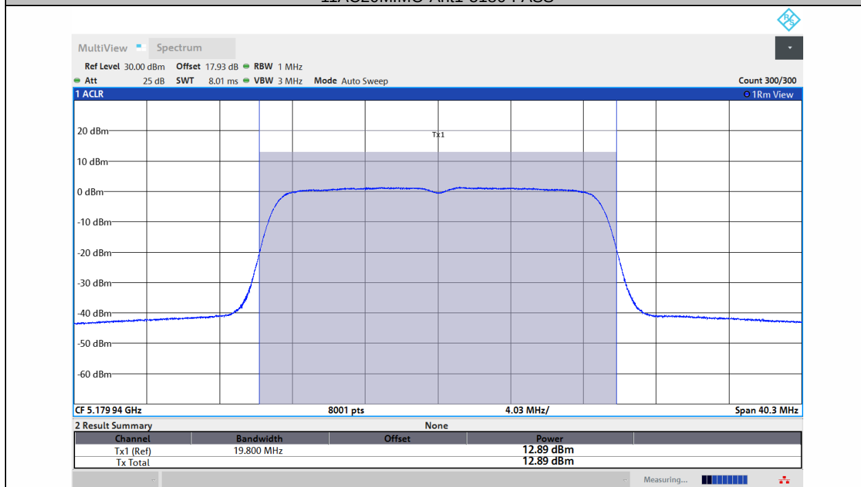
11AC20MIMO-Ant2-5180-PASS
