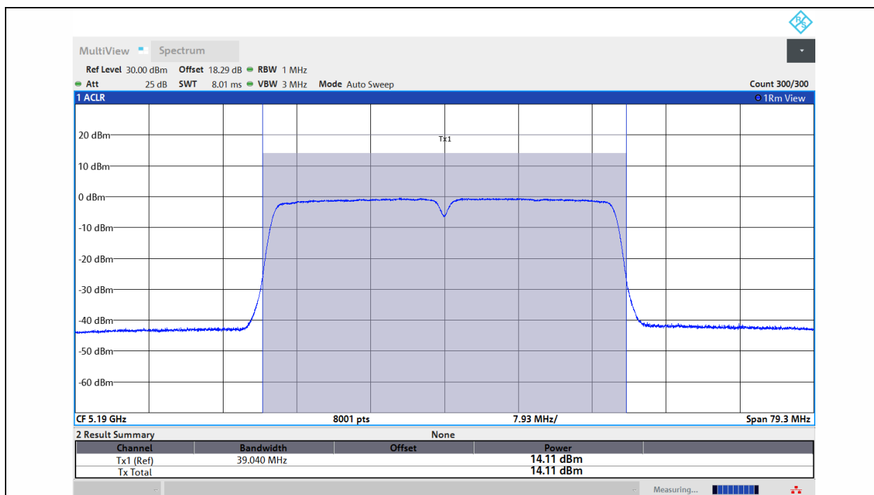
11N40MIMO-Ant1-5190-PASS
