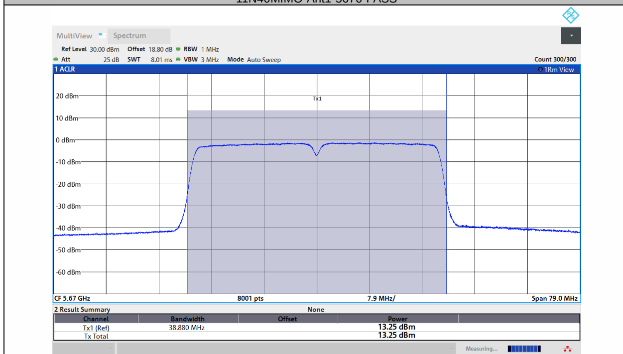
11N40MIMO-Ant2-5670-PASS
