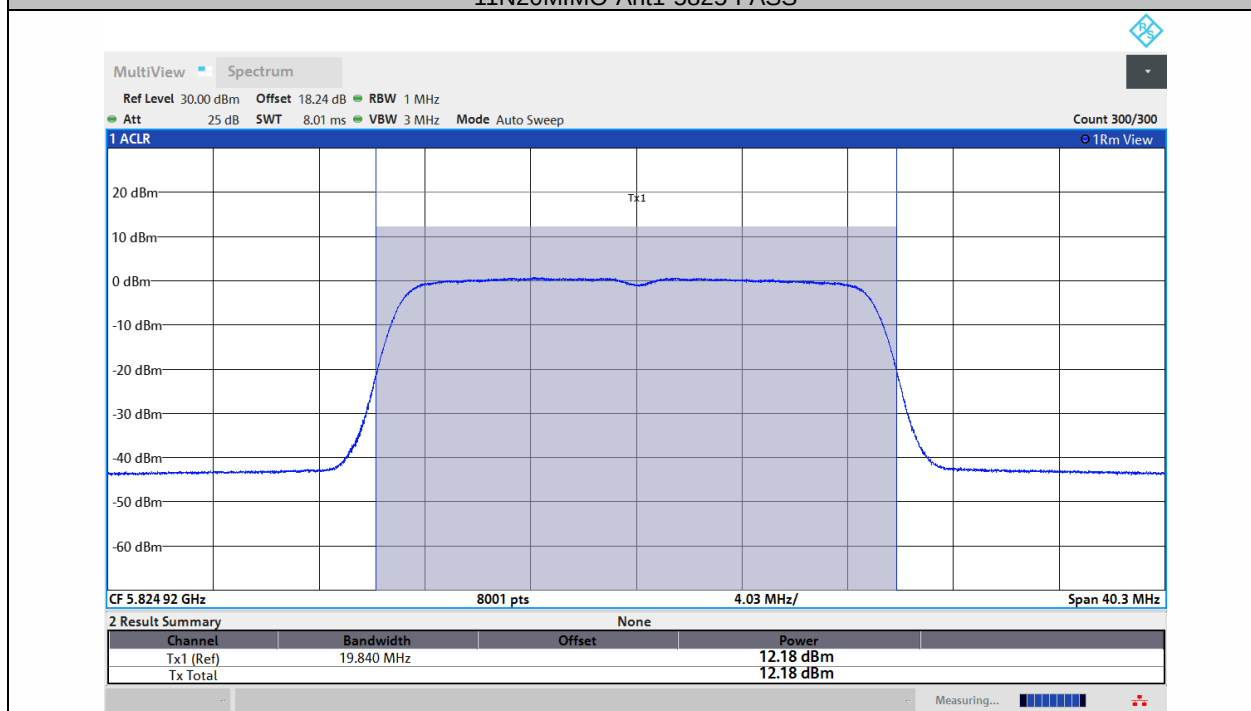
11N20MIMO-Ant2-5825-PASS
