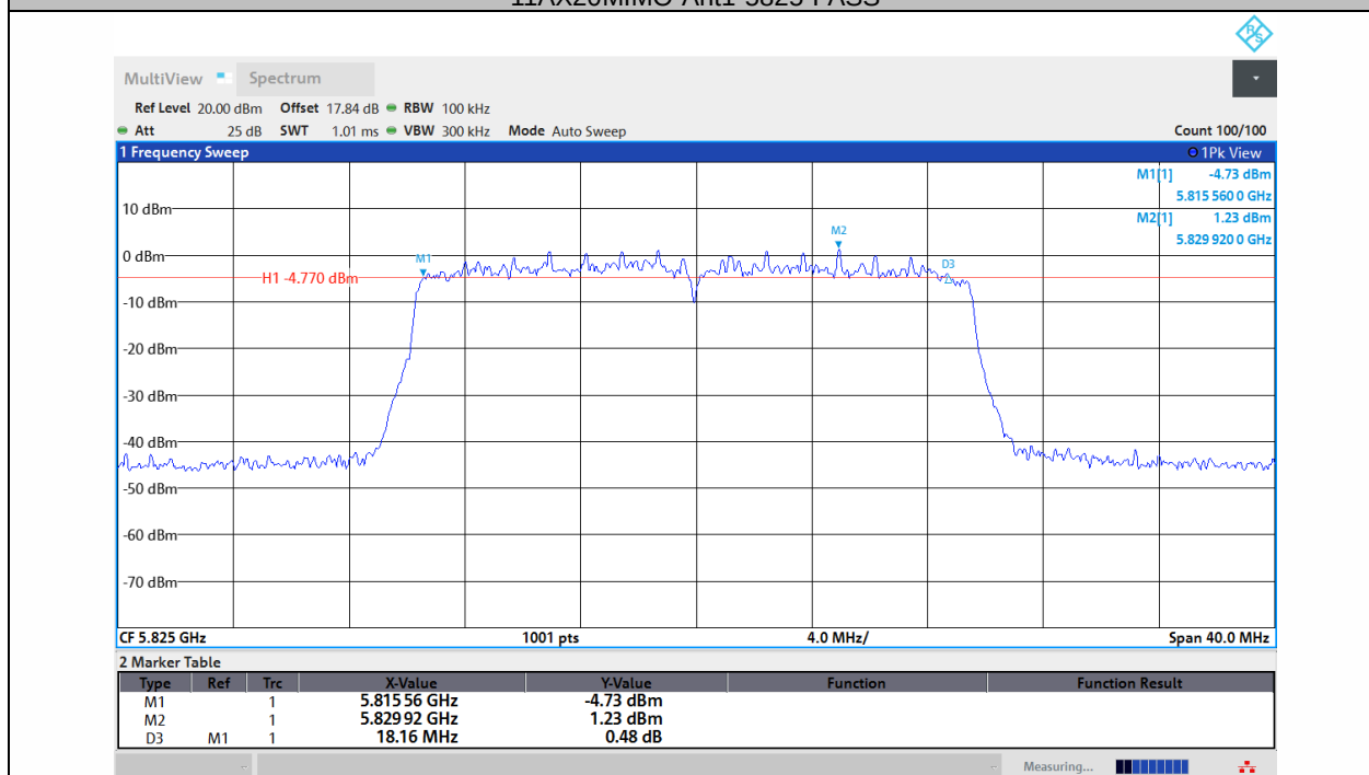
11AX20MIMO-Ant2-5825-PASS
