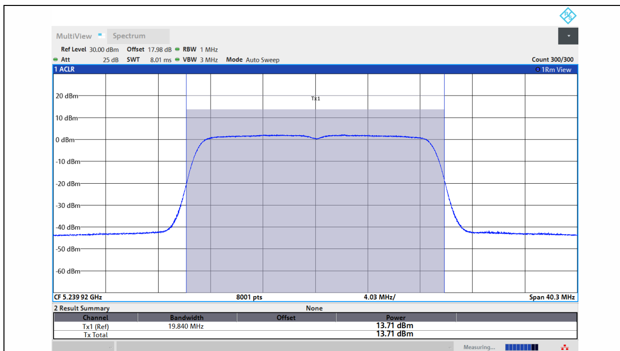
11AC20MIMO-Ant1-5240-PASS
