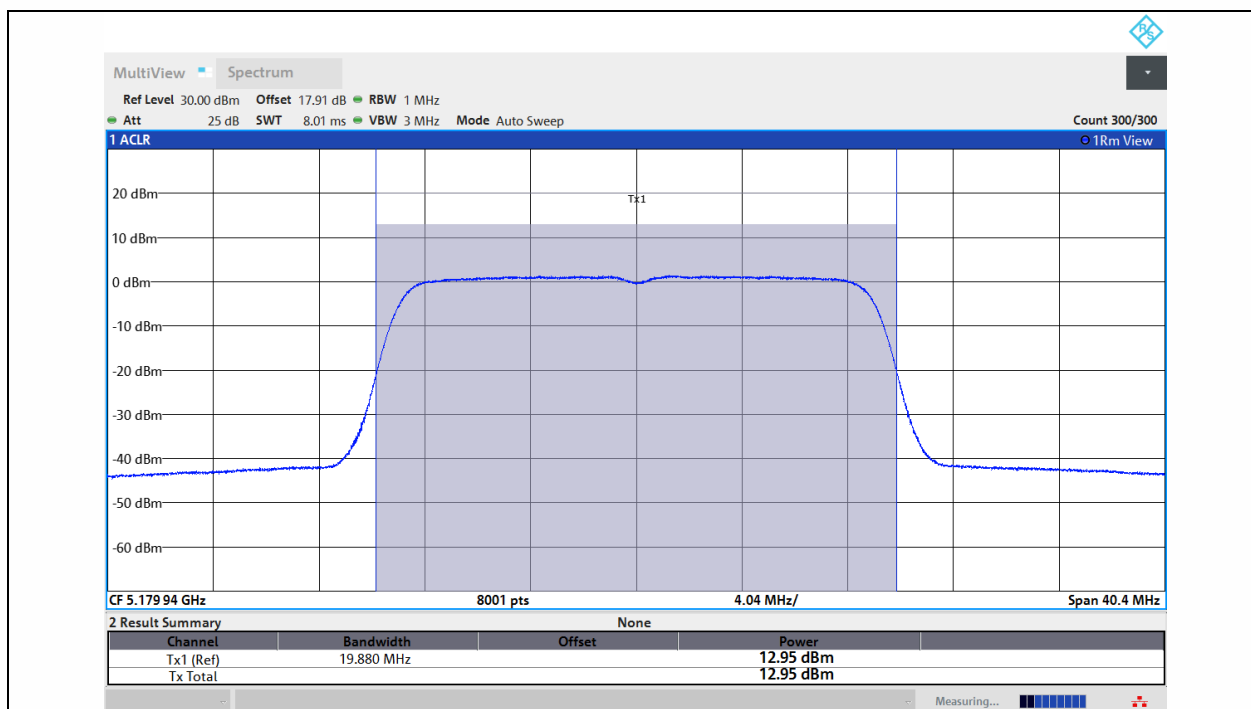
11N20MIMO-Ant1-5180-PASS
