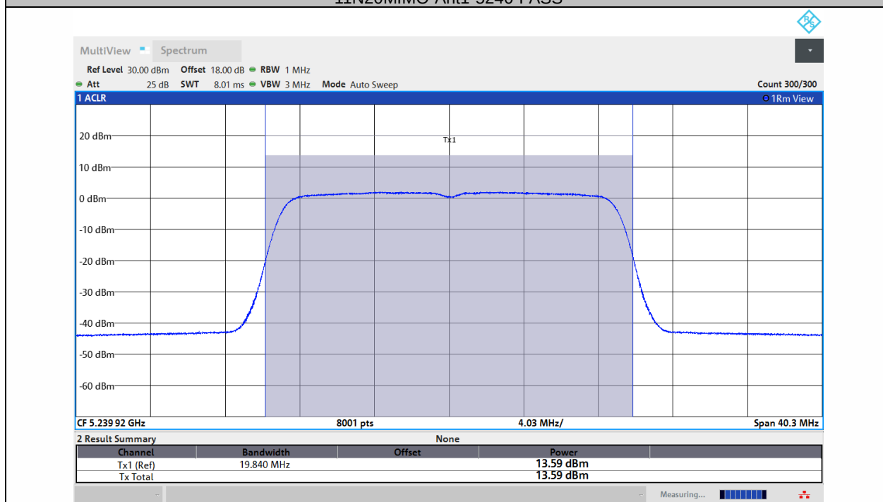
11N20MIMO-Ant2-5240-PASS
