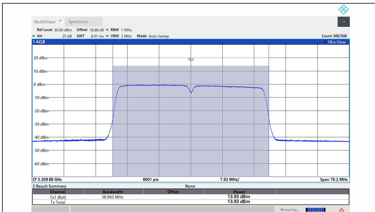
11N40MIMO-Ant1-5310-PASS
