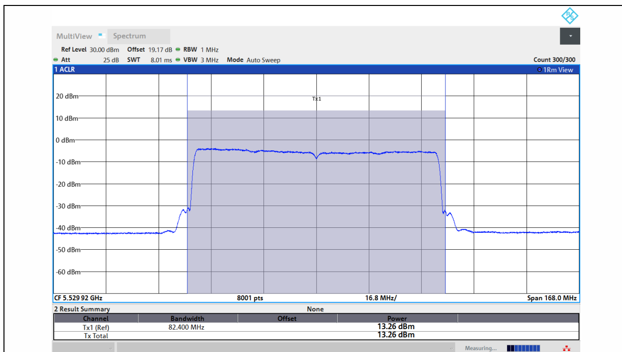
11AX80MIMO-Ant1-5530-PASS
