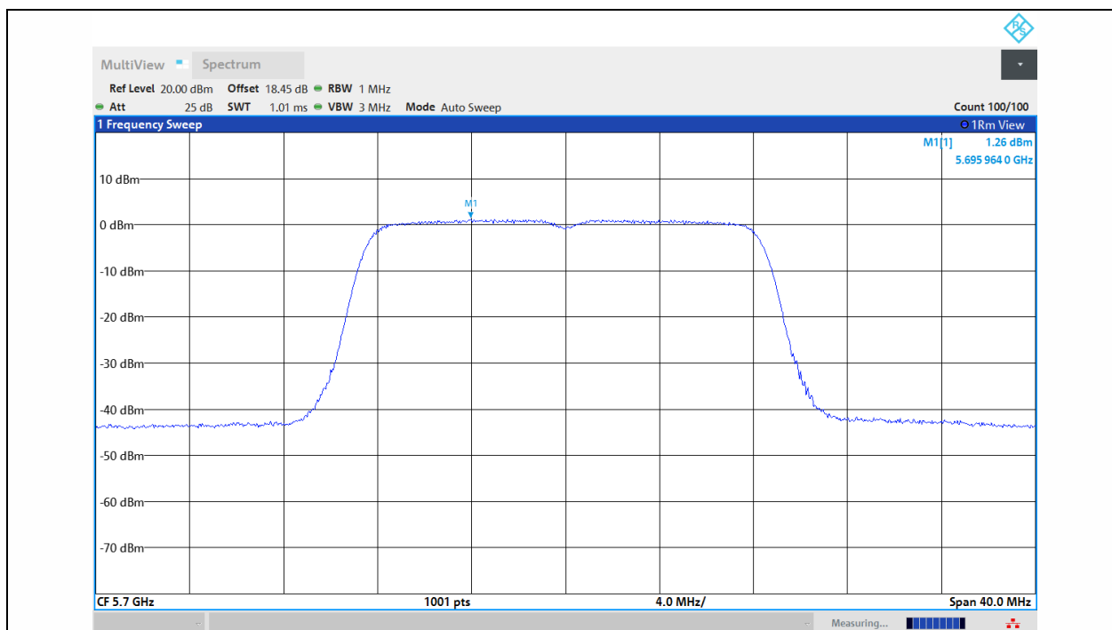
11A-Ant1-5700-PASS
