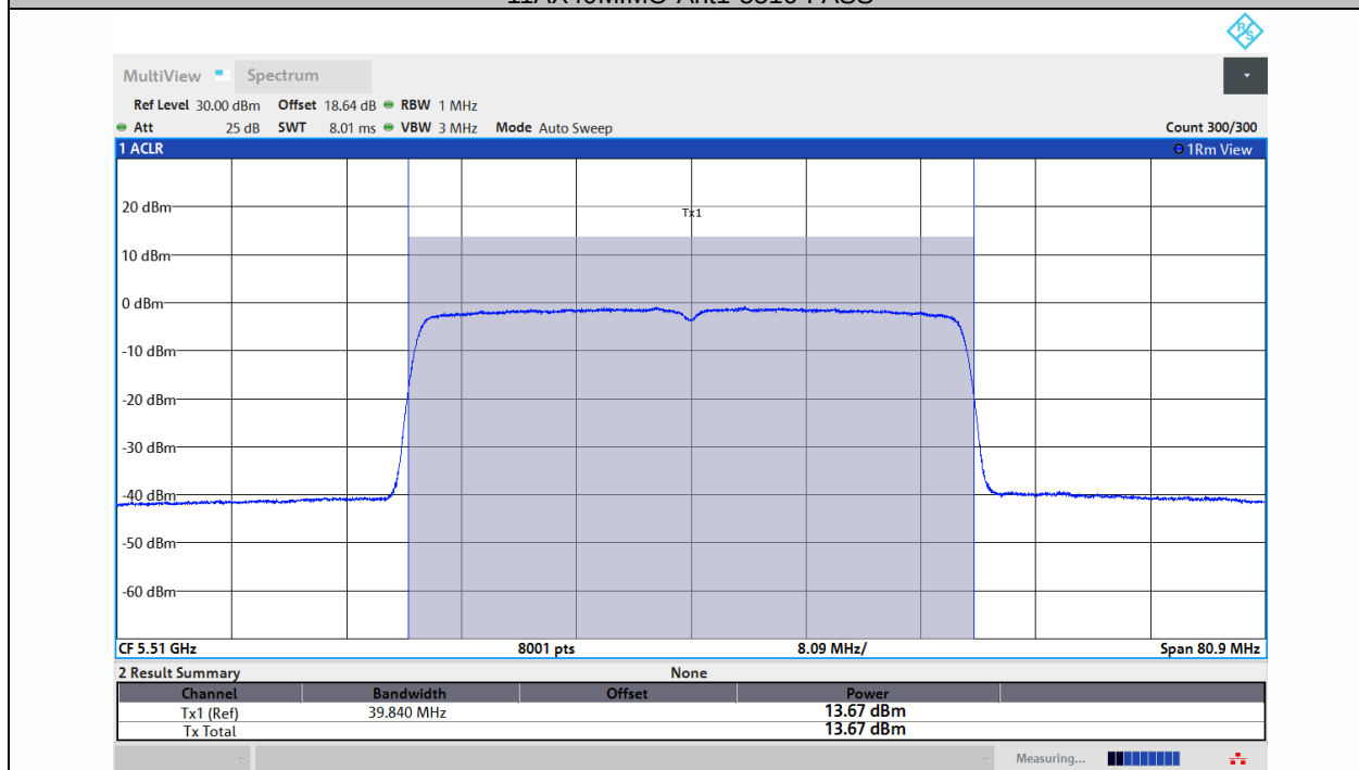
11AX40MIMO-Ant2-5510-PASS
