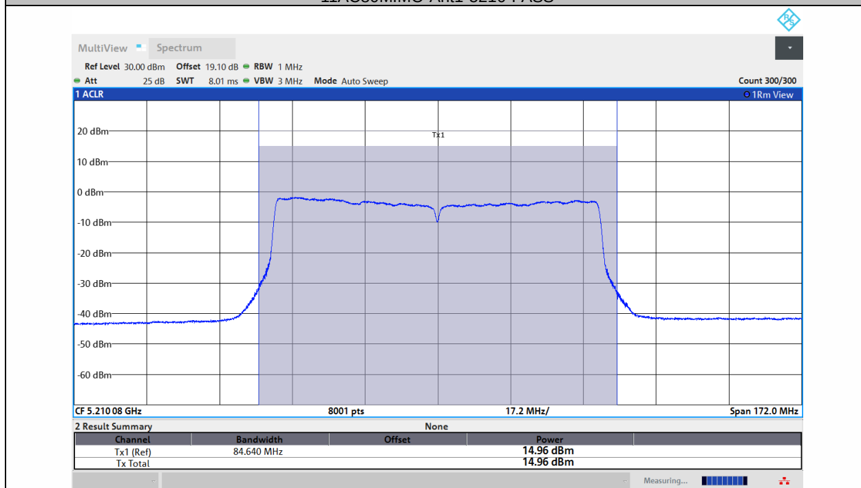
11AC80MIMO-Ant2-5210-PASS
