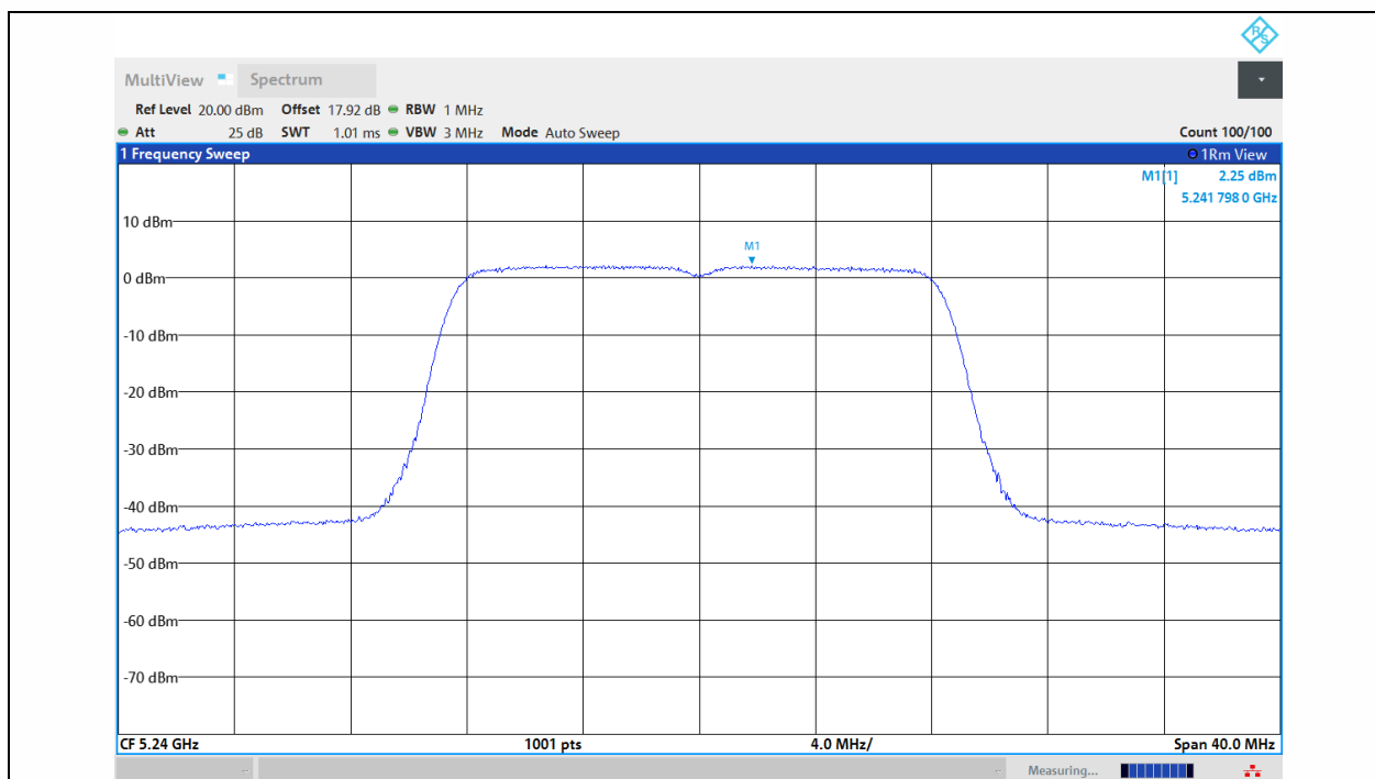
11A-Ant1-5240-PASS
