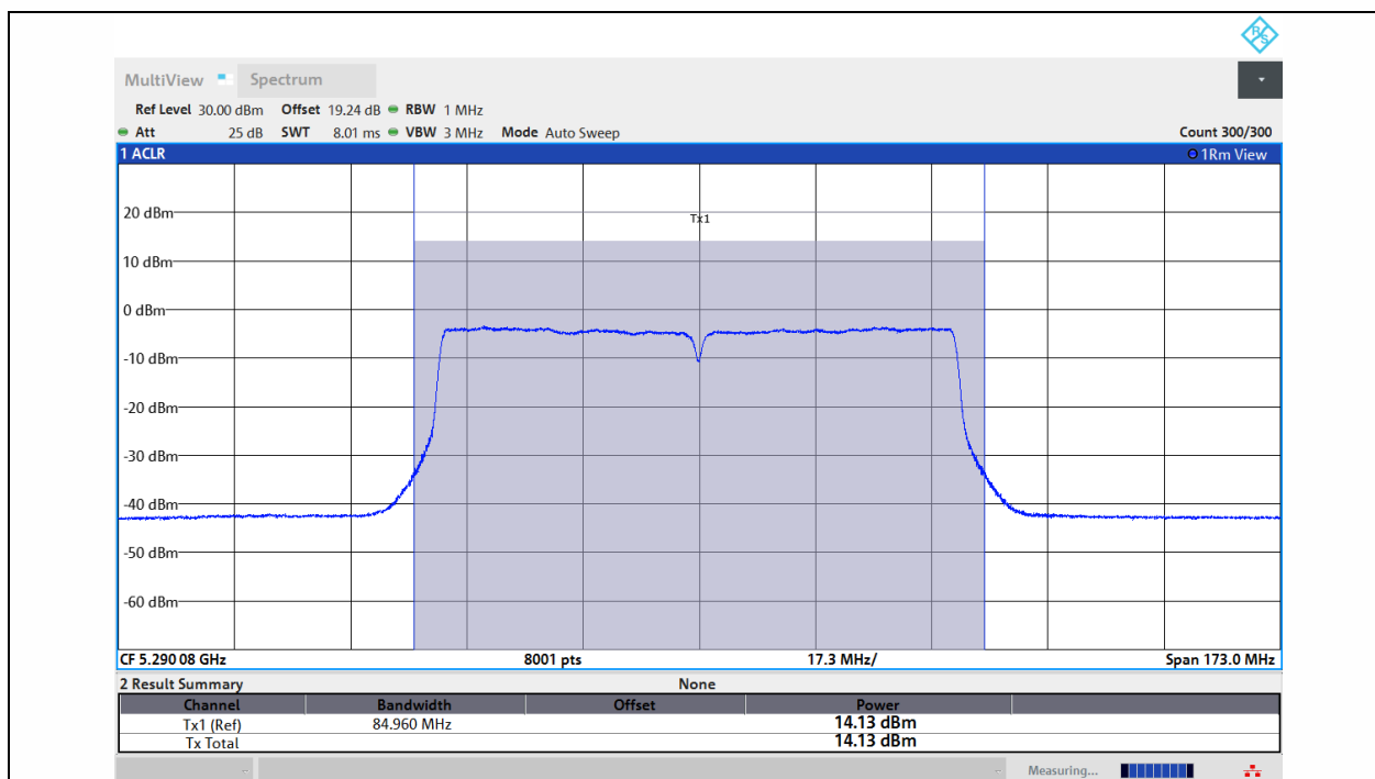
11AC80MIMO-Ant1-5290-PASS
