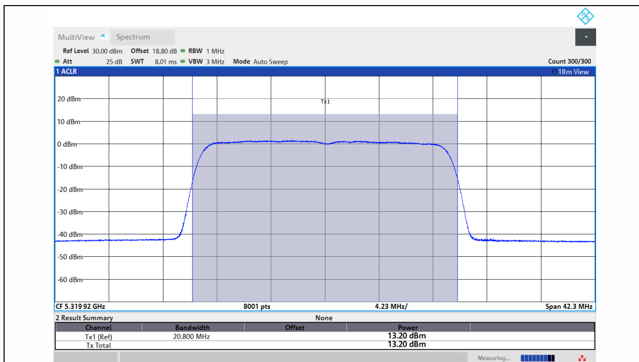
11AX20MIMO-Ant1-5320-PASS
