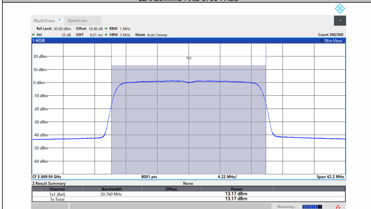
11AX20MIMO-Ant2-5700-PASS
