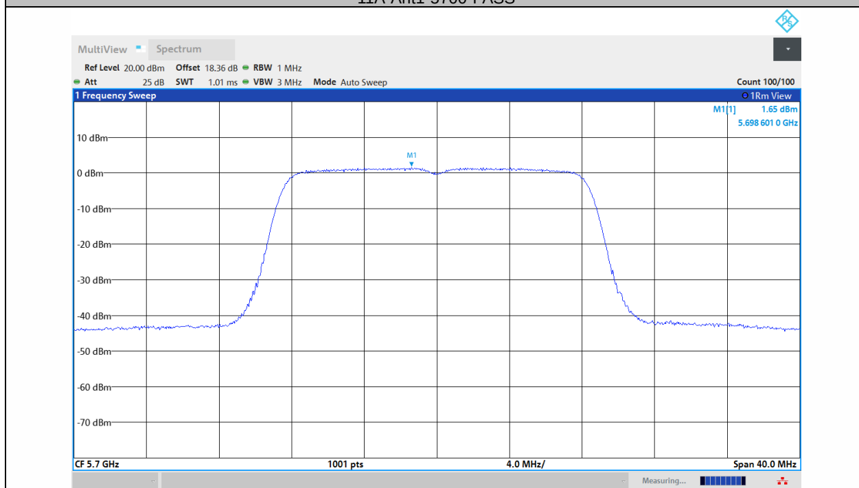
11A-Ant2-5700-PASS
