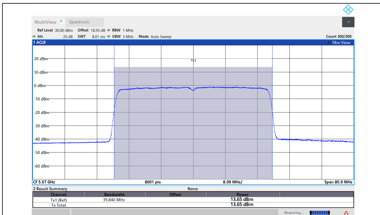
11AX40MIMO-Ant1-5670-PASS
