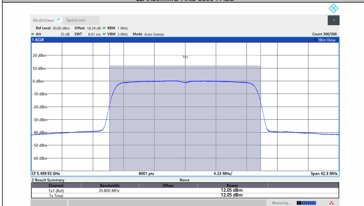
11AX20MIMO-Ant2-5500-PASS
