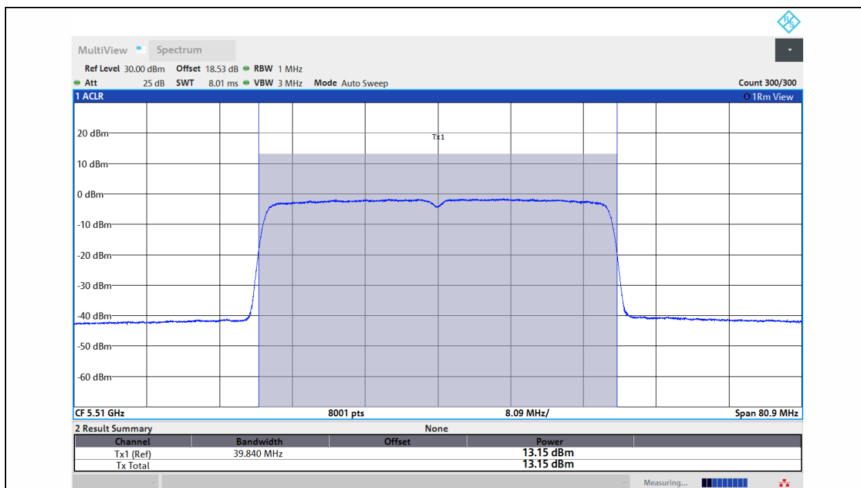
11AX40MIMO-Ant1-5510-PASS
