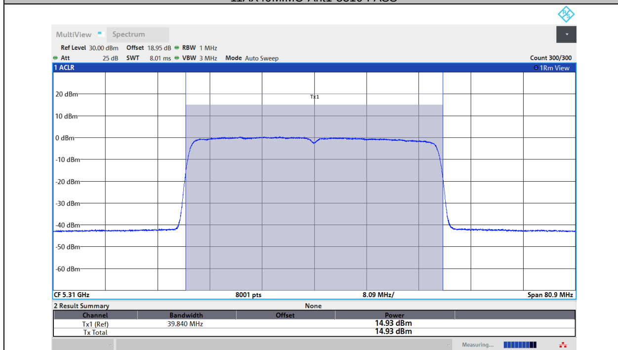
11AX40MIMO-Ant2-5310-PASS
