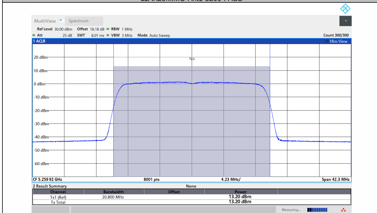
11AX20MIMO-Ant2-5260-PASS
