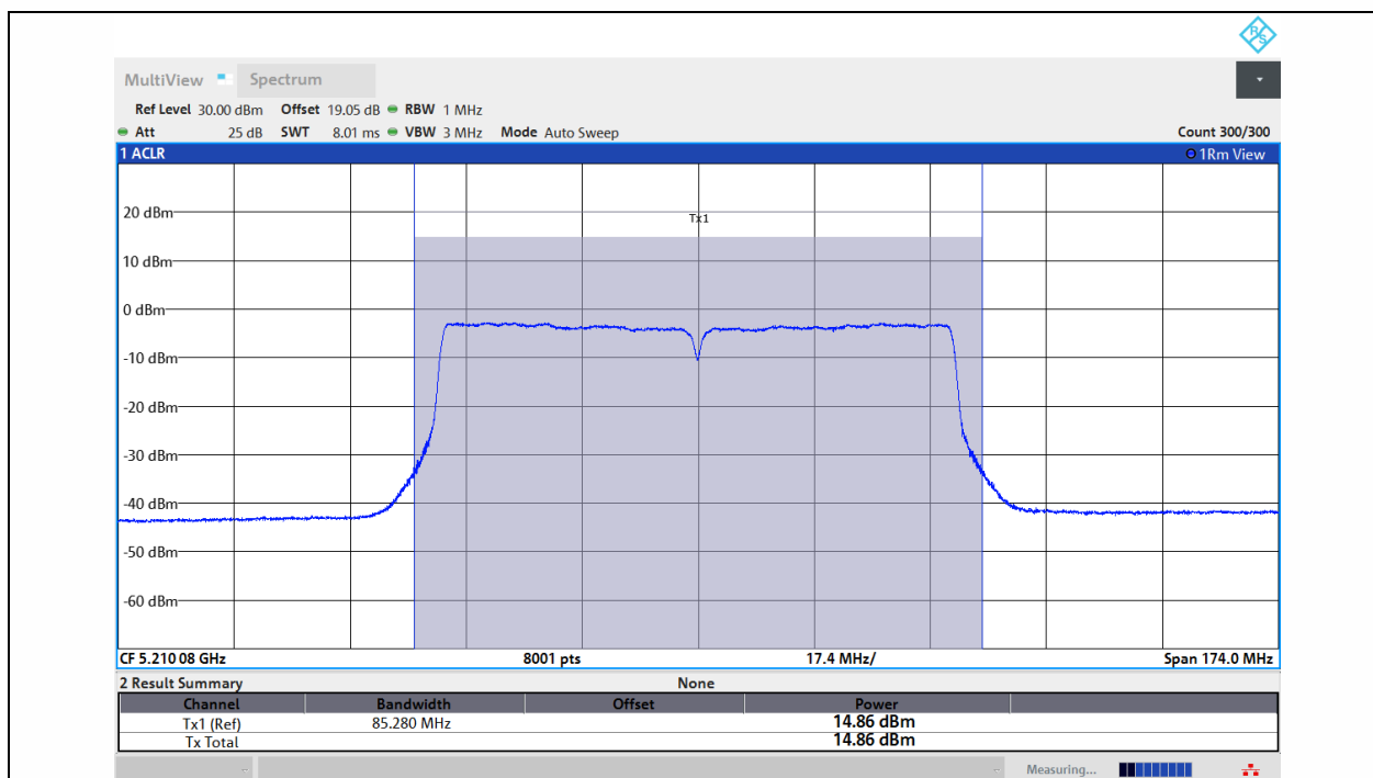
11AC80MIMO-Ant1-5210-PASS
