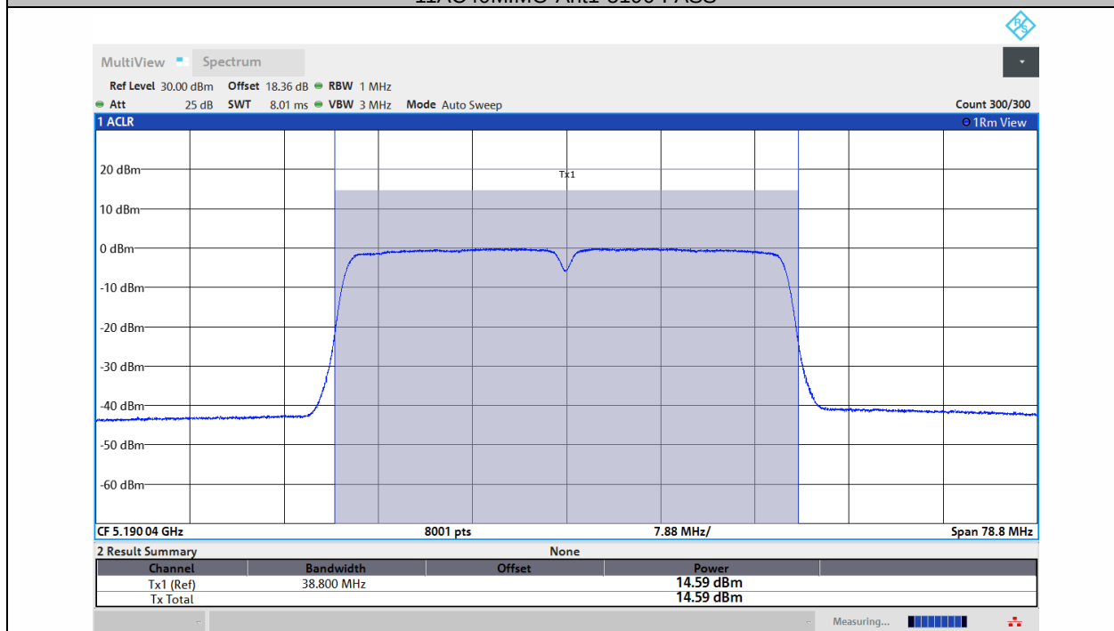
11AC40MIMO-Ant2-5190-PASS
