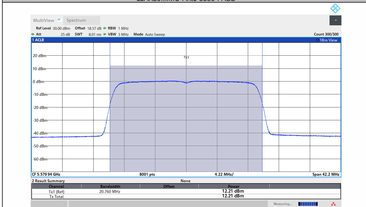
11AX20MIMO-Ant2-5580-PASS
