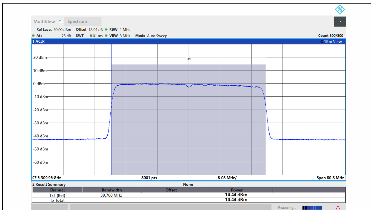
11AX40MIMO-Ant1-5310-PASS
