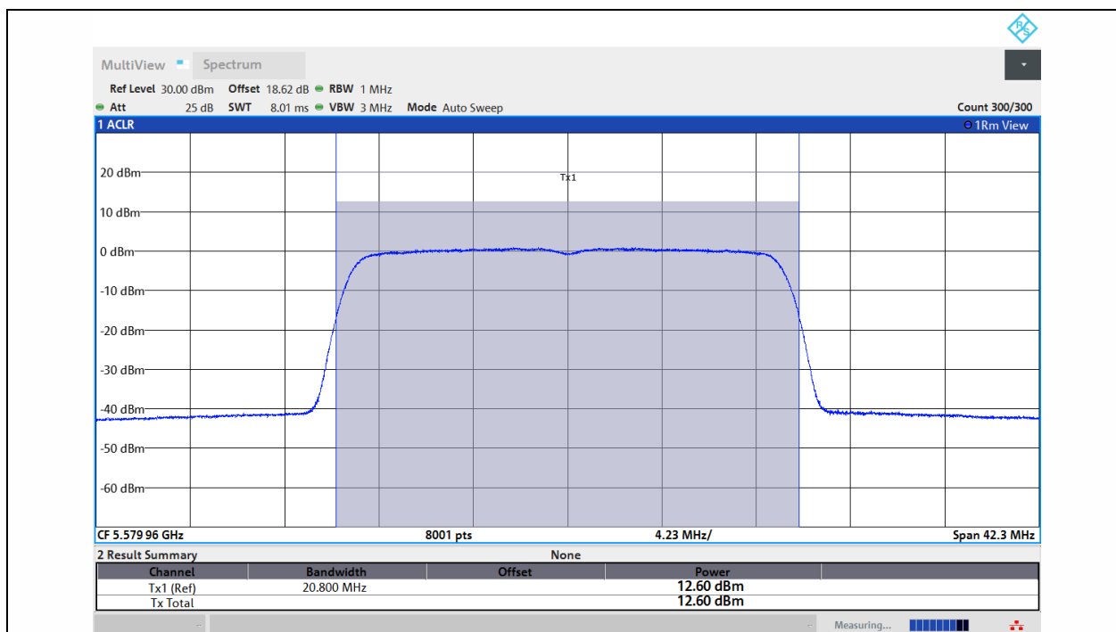
11AX20MIMO-Ant1-5580-PASS
