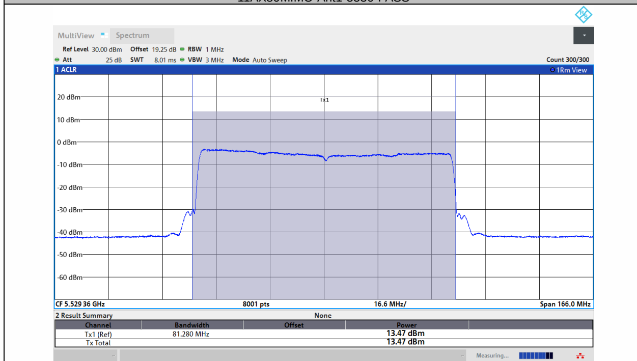
11AX80MIMO-Ant2-5530-PASS
