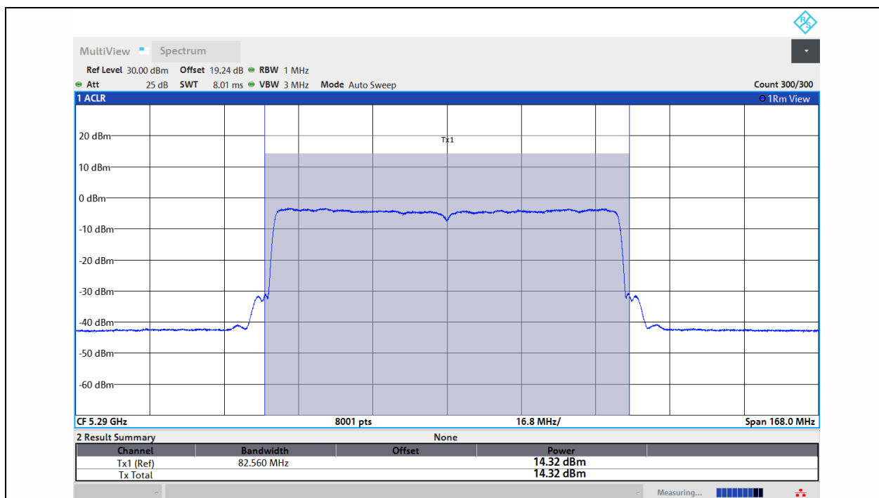
11AX80MIMO-Ant1-5290-PASS
