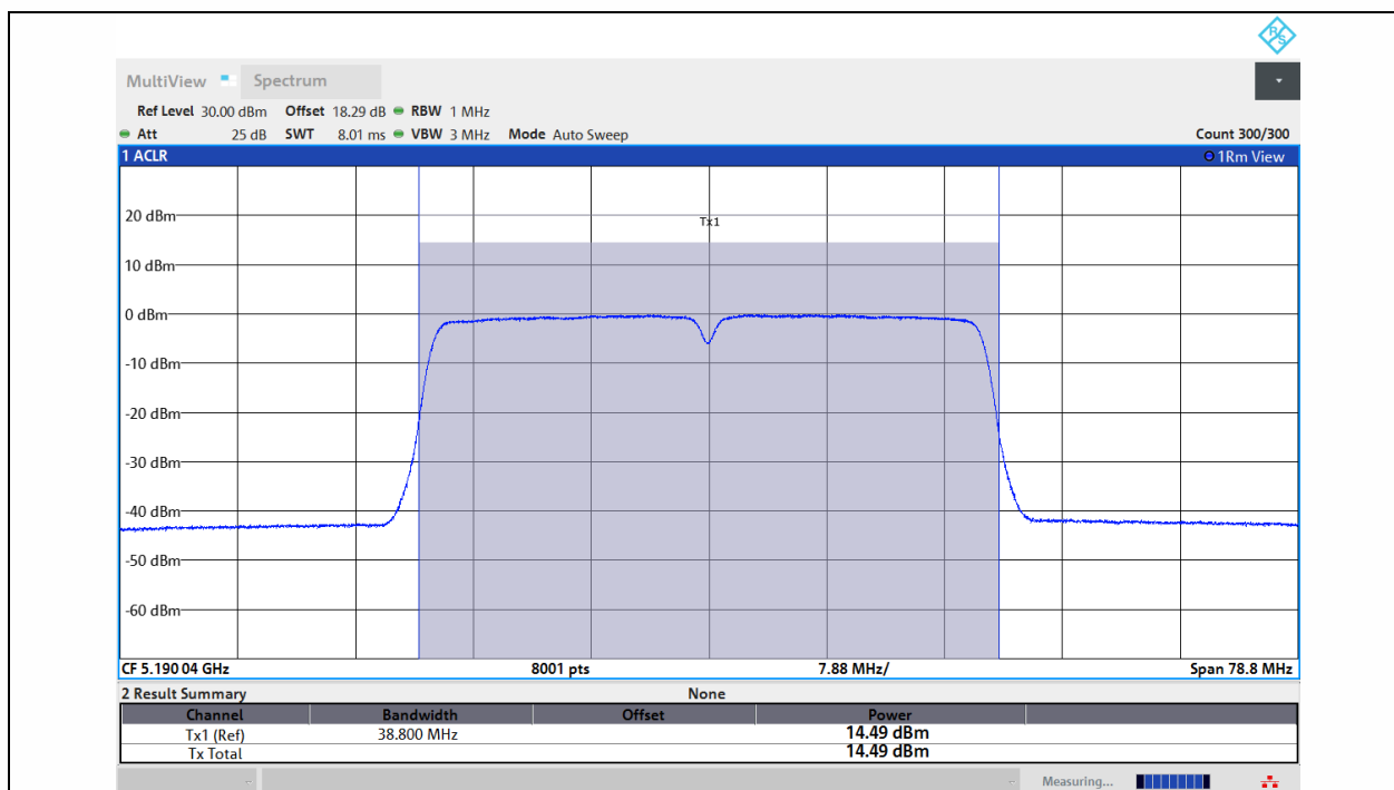
11AC40MIMO-Ant1-5190-PASS
