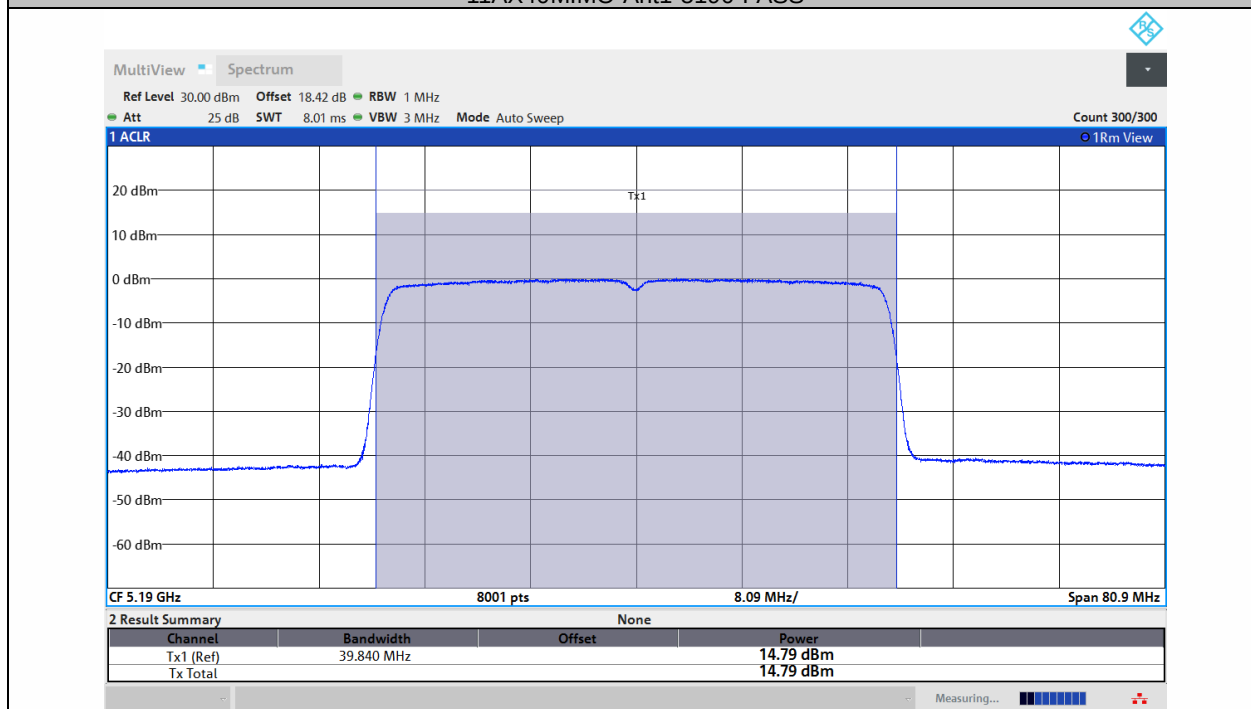
11AX40MIMO-Ant2-5190-PASS
