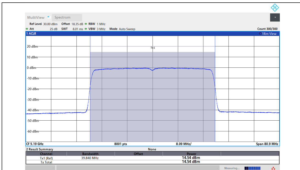
11AX40MIMO-Ant1-5190-PASS
