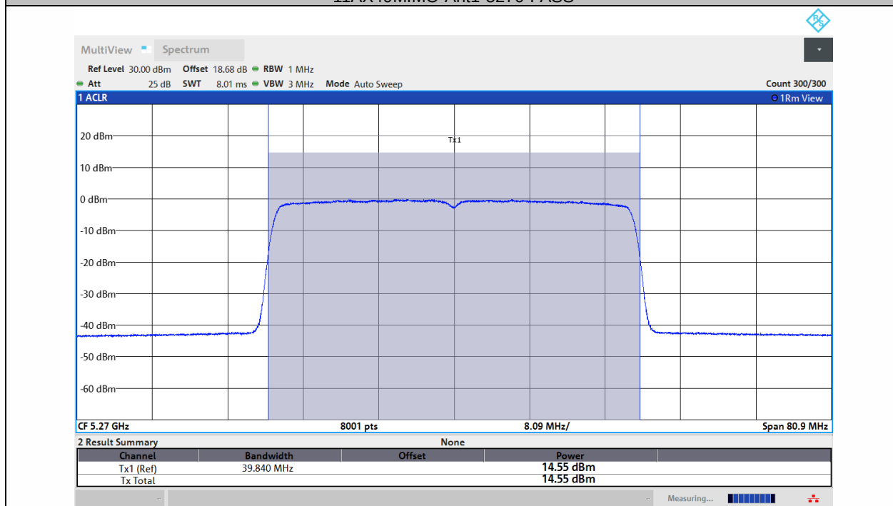
11AX40MIMO-Ant2-5270-PASS
