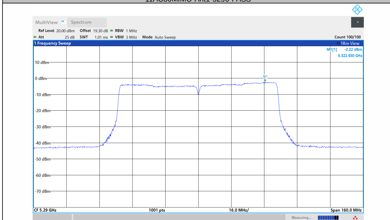
11AC80MIMO-Ant2-5290-PASS
