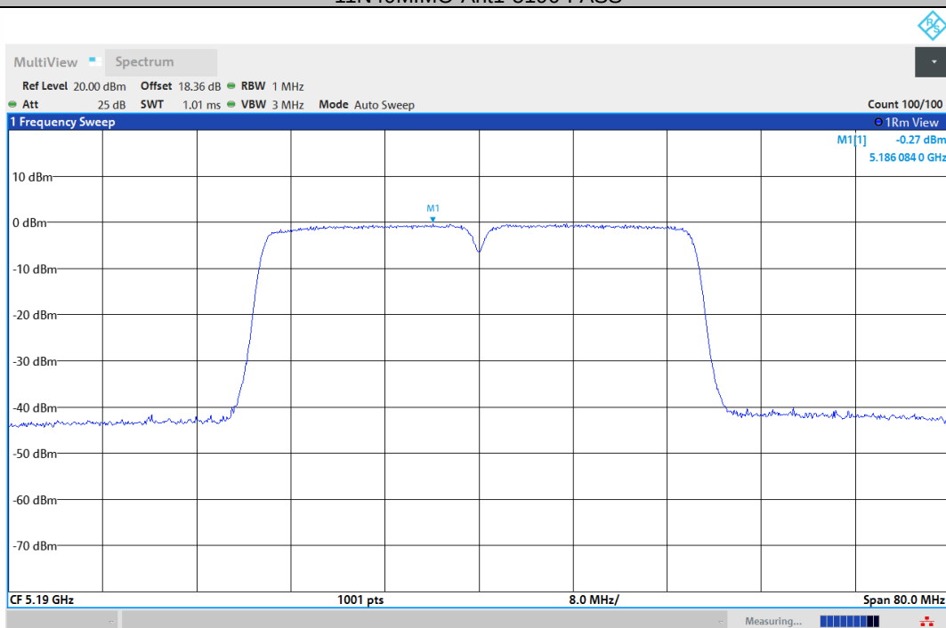
11N40MIMO-Ant2-5190-PASS
