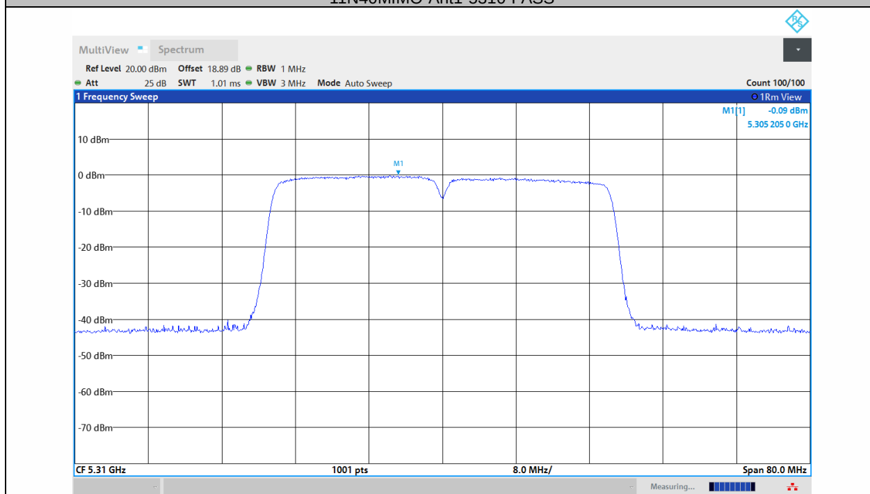
11N40MIMO-Ant2-5310-PASS
