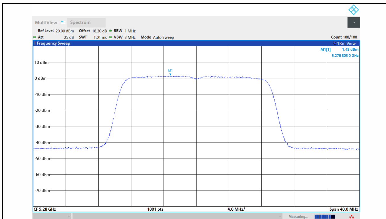
11AC20MIMO-Ant1-5280-PASS
