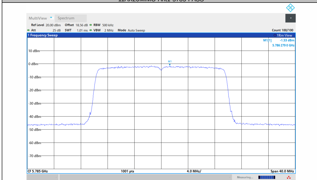
11AX20MIMO-Ant2-5785-PASS
