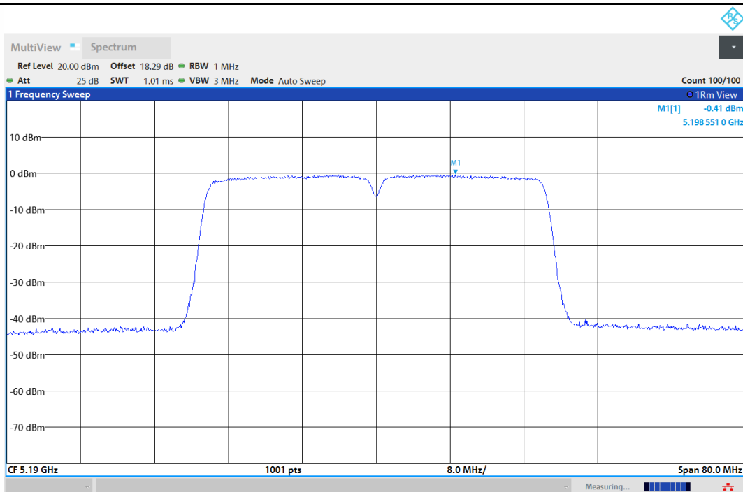
11N40MIMO-Ant1-5190-PASS
