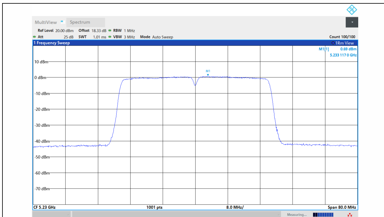
11AC40MIMO-Ant1-5230-PASS
