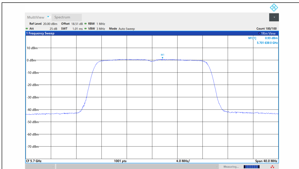
11N20MIMO-Ant1-5700-PASS
