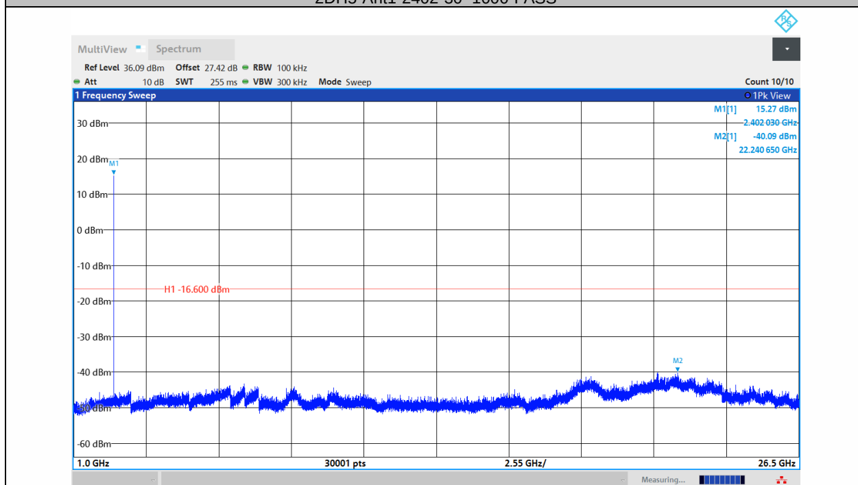
2DH5-Ant1-2402-1000~26500-PASS
