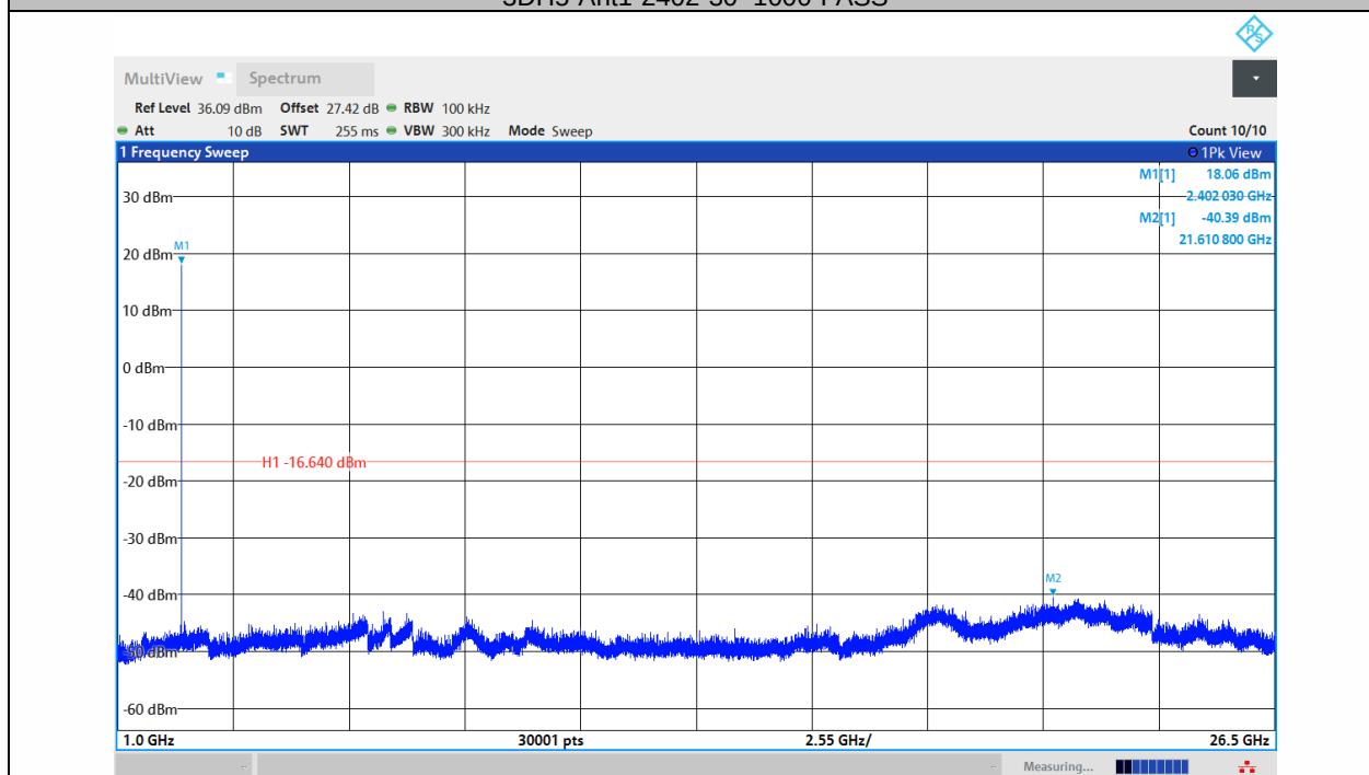
3DH5-Ant1-2402-1000~26500-PASS
