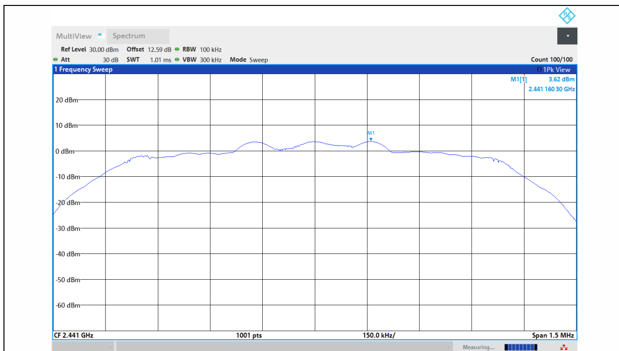
2DH5-Ant1-2441-PASS
