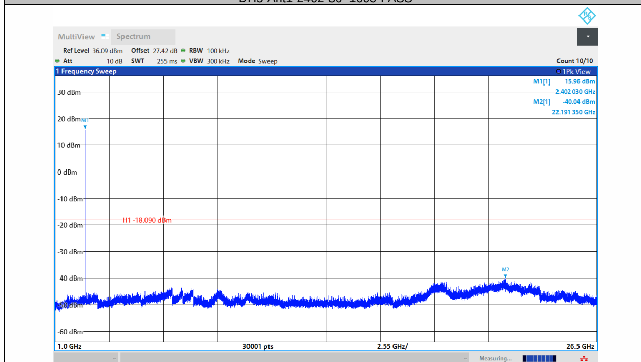
DH5-Ant1-2402-1000~26500-PASS
