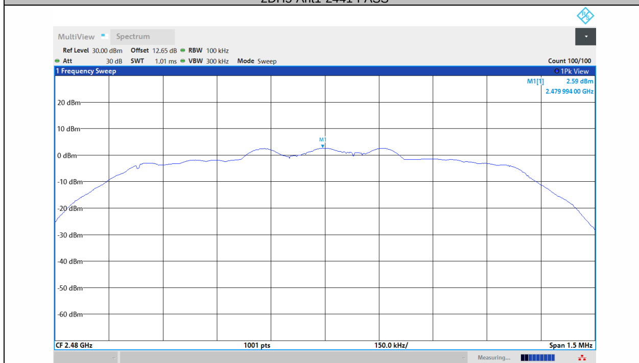
2DH5-Ant1-2480-PASS
