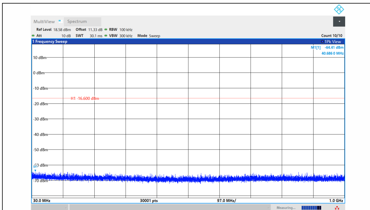
2DH5-Ant1-2402-30~1000-PASS
