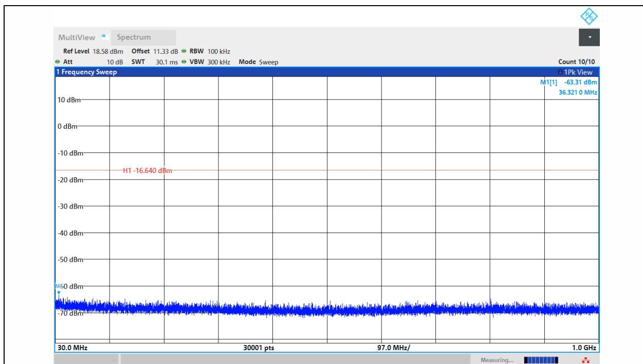
3DH5-Ant1-2402-30~1000-PASS
