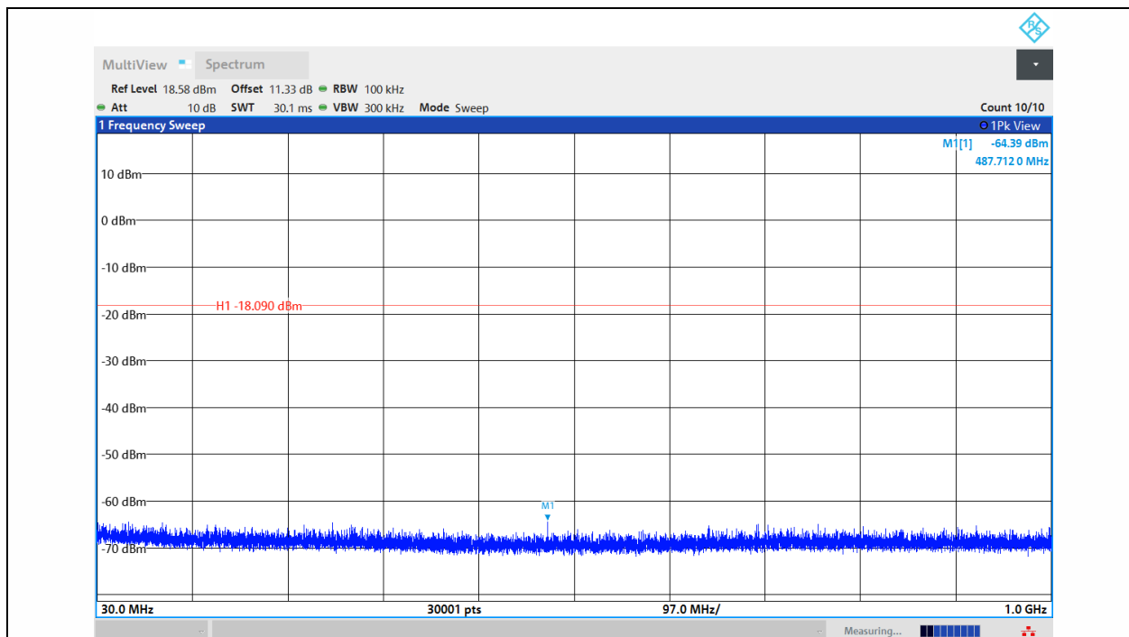
DH5-Ant1-2402-30~1000-PASS
