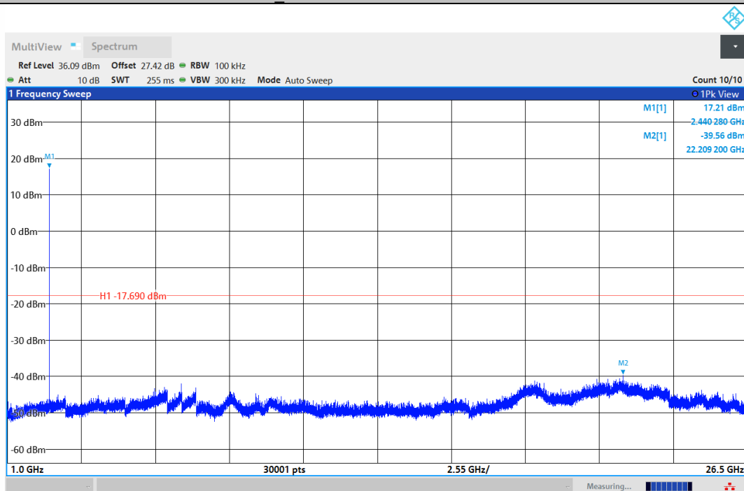
BLE_1M-Ant1-2440-1000~26500-PASS
