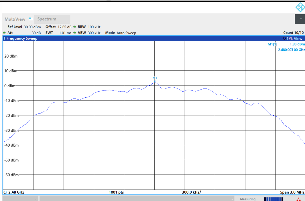
BLE_2M-Ant1-2480-0-Reference-PASS
