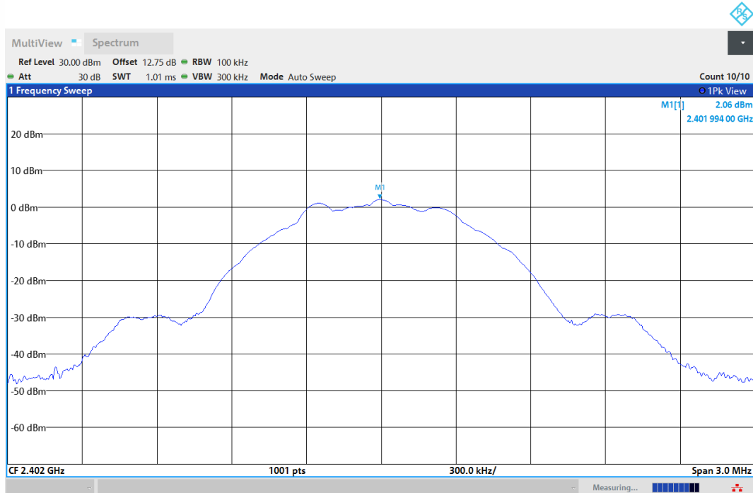
BLE_1M-Ant1-2402-0-Reference-PASS
