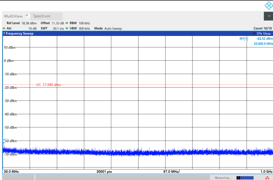
BLE_1M-Ant1-2402-30-1000-PASS
