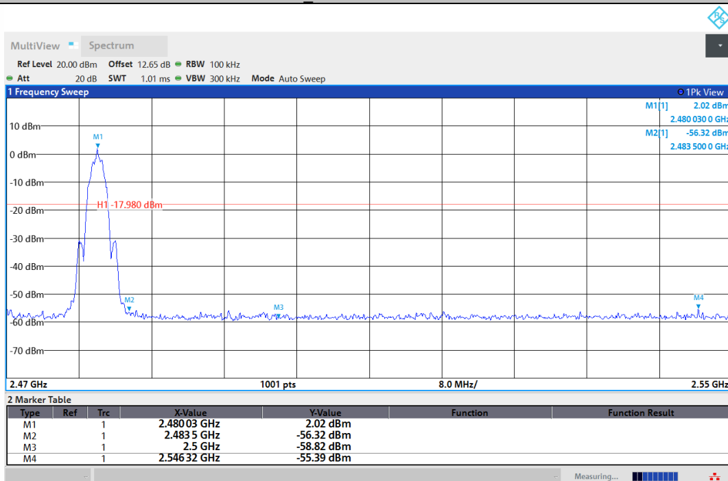
BLE_2M-Ant1-2480-PASS
