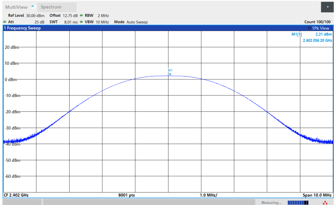
BLE_1M-Ant1-2402-PASS
