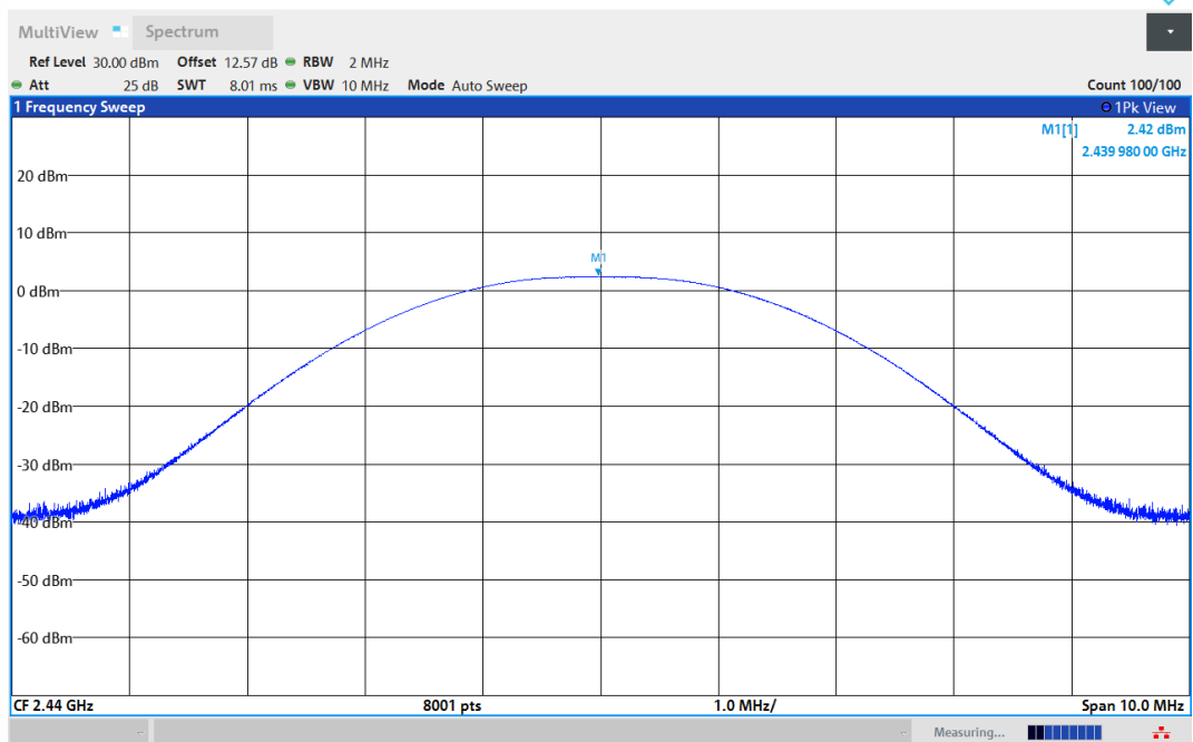
BLE_1M-Ant1-2440-PASS
