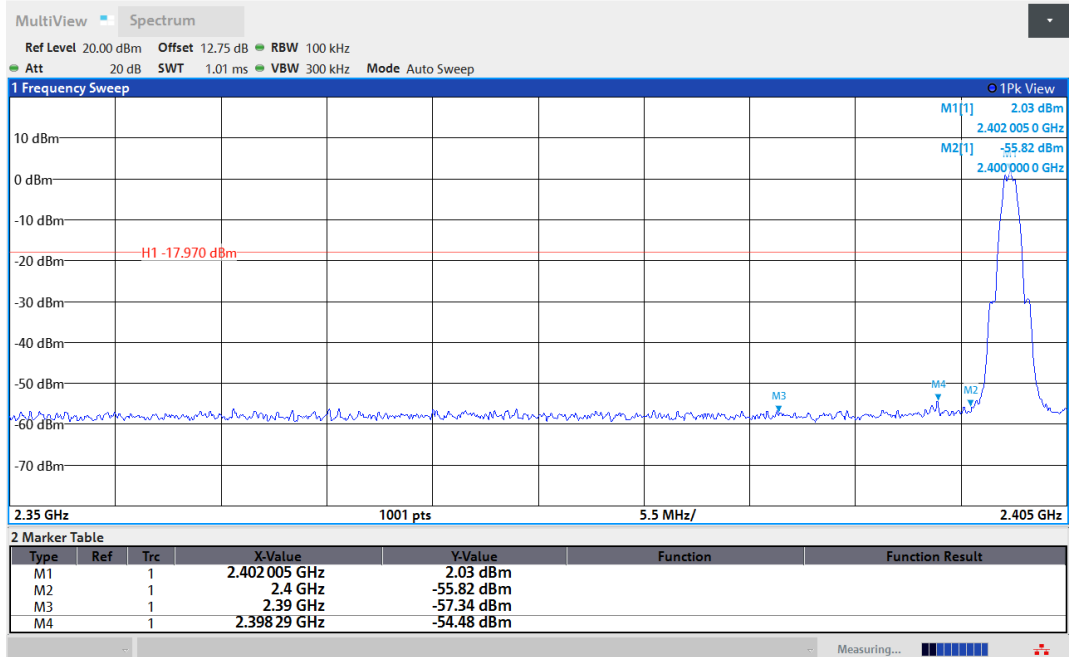
BLE_1M-Ant1-2402-PASS
