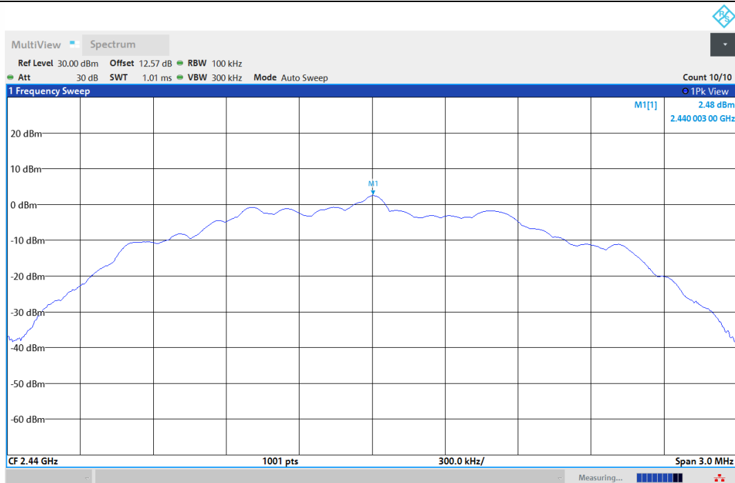
BLE_2M-Ant1-2440-0-Reference-PASS
