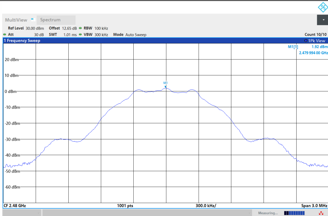
BLE_1M-Ant1-2480-0-Reference-PASS
