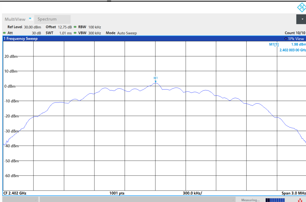
BLE_2M-Ant1-2402-0~Reference-PASS
