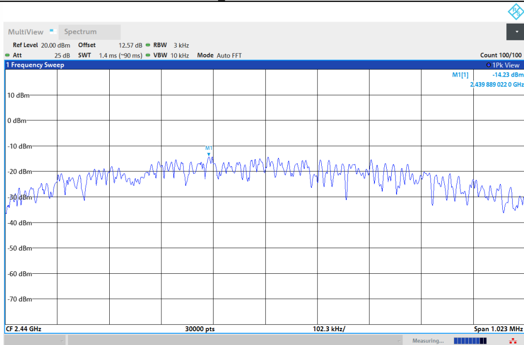
BLE_1M-Ant1-2440-PASS
