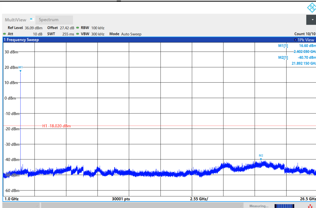
BLE_2M-Ant1-2402-1000~26500-PASS
