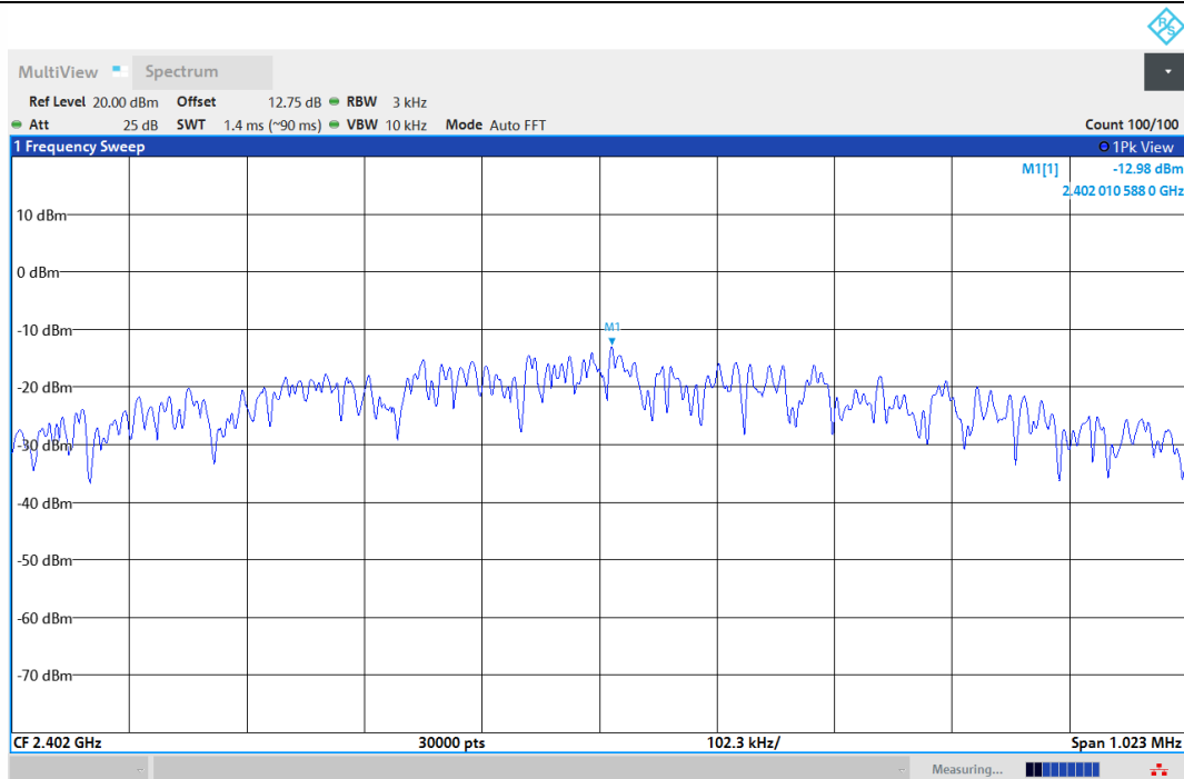
BLE_1M-Ant1-2402-PASS
