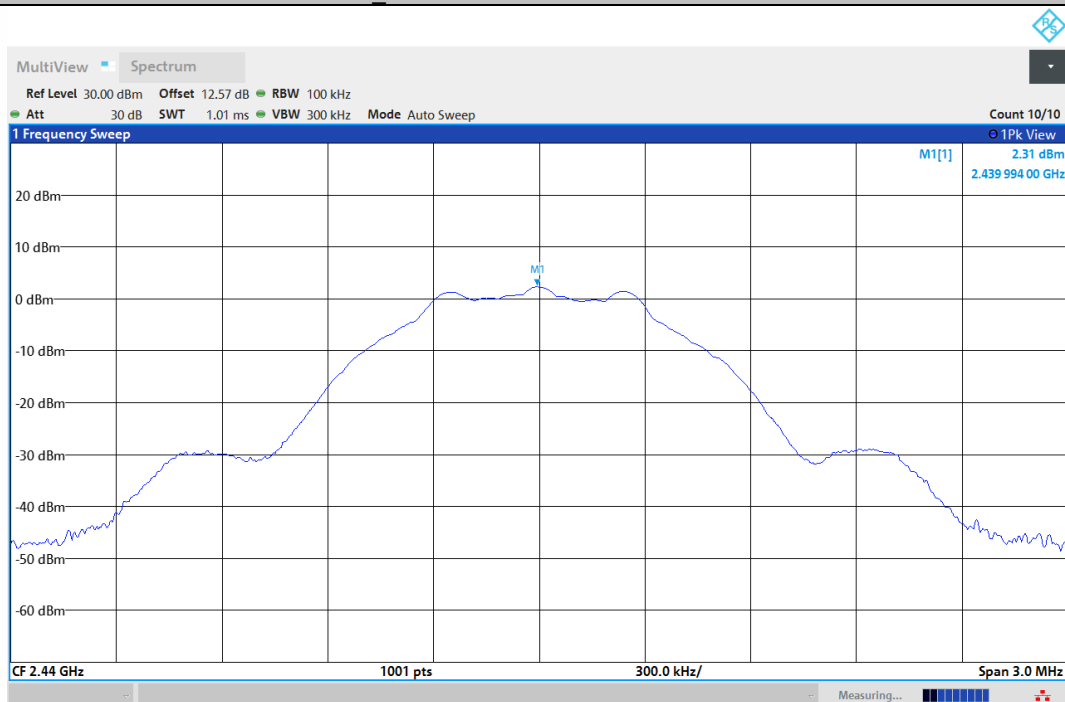
BLE_1M-Ant1-2440-0-Reference-PASS
