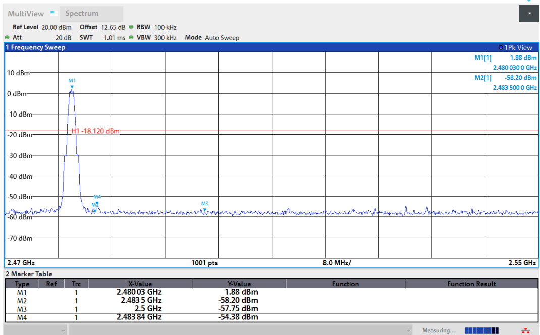
BLE_1M-Ant1-2480-PASS
