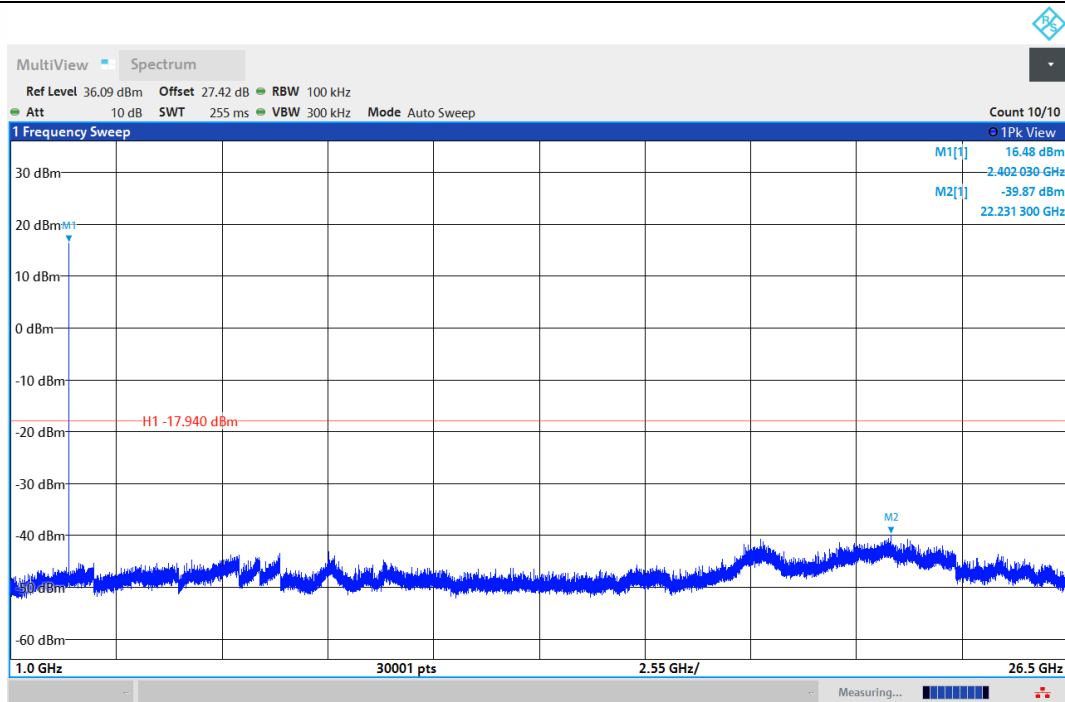
BLE_1M-Ant1-2402-1000~26500-PASS
