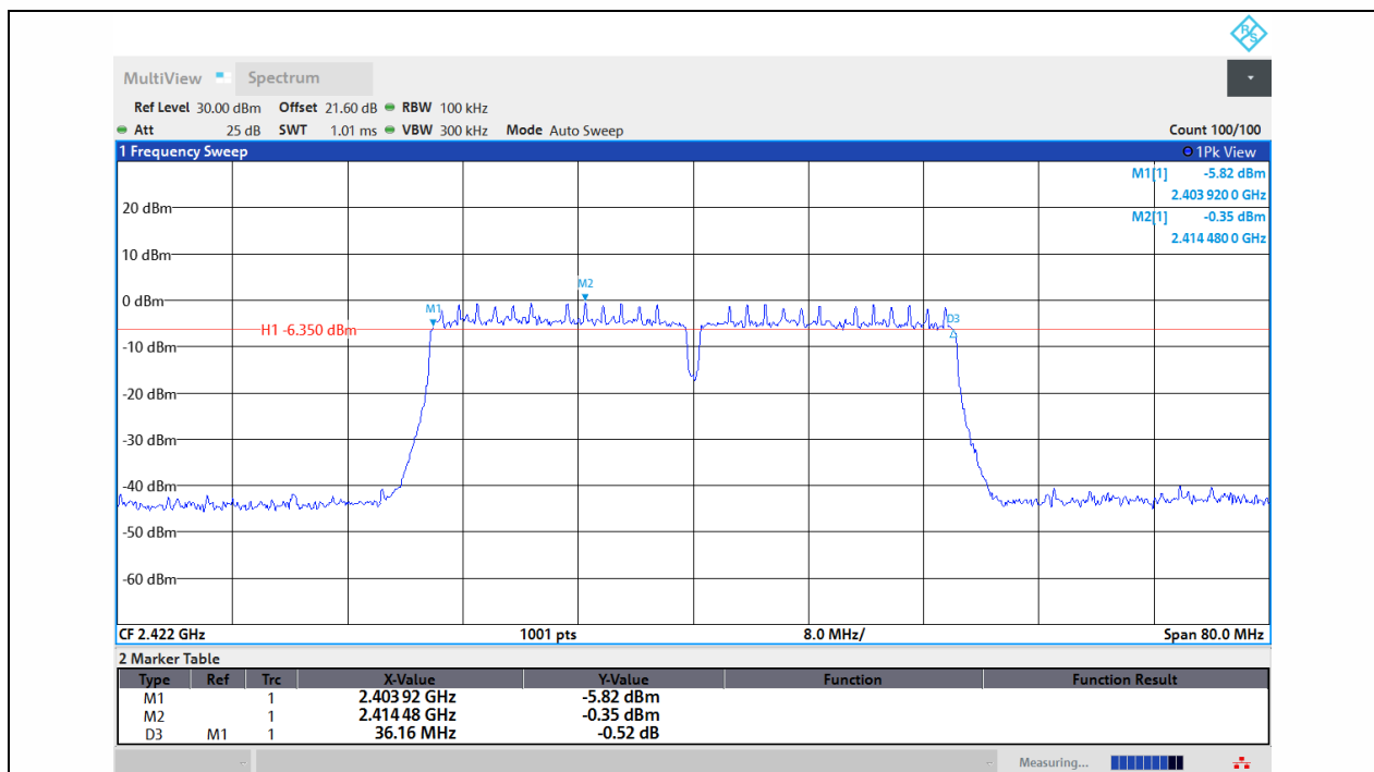
11N40MIMO-Ant1-2422-PASS
