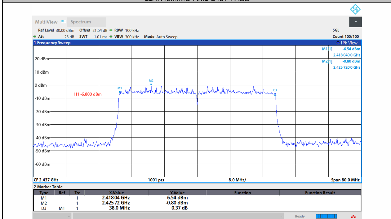
11AX40MIMO-Ant2-2437-PASS
