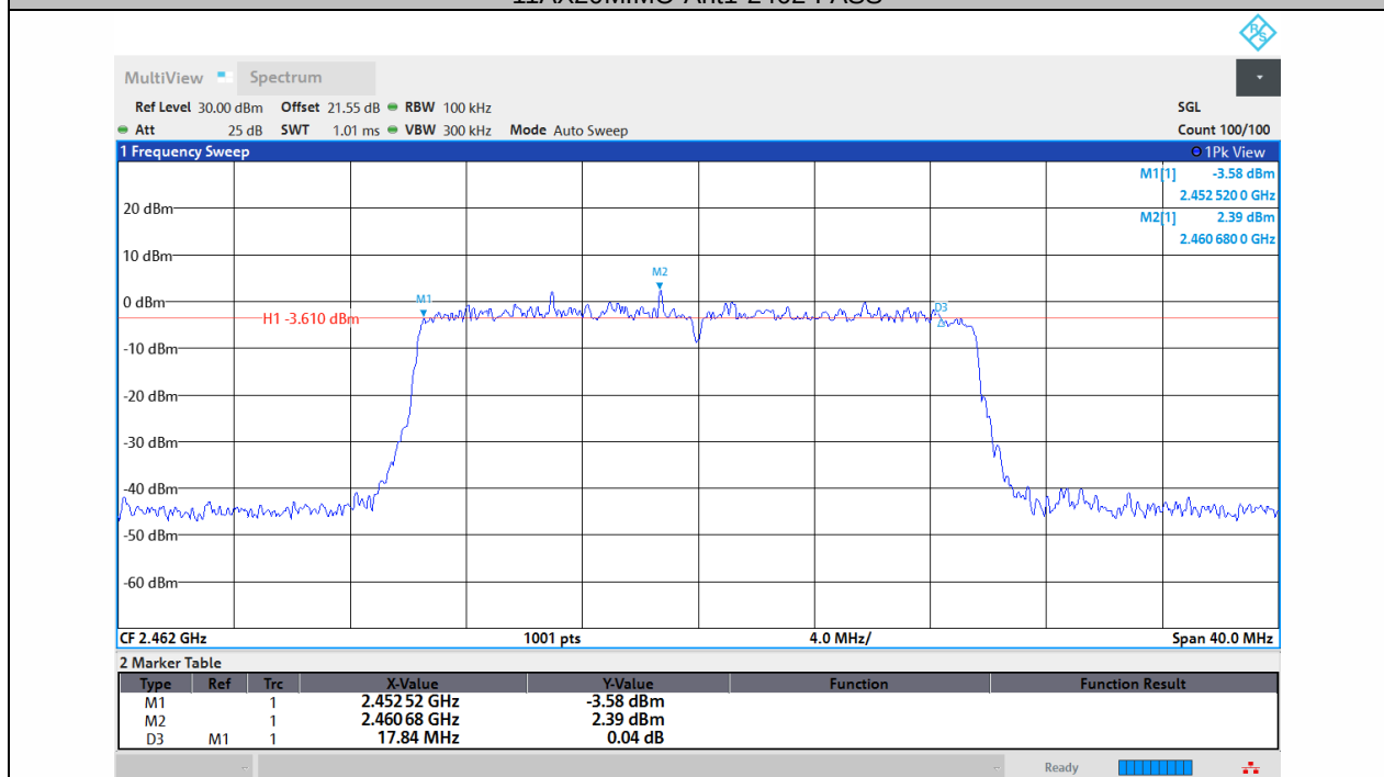
11AX20MIMO-Ant2-2462-PASS
