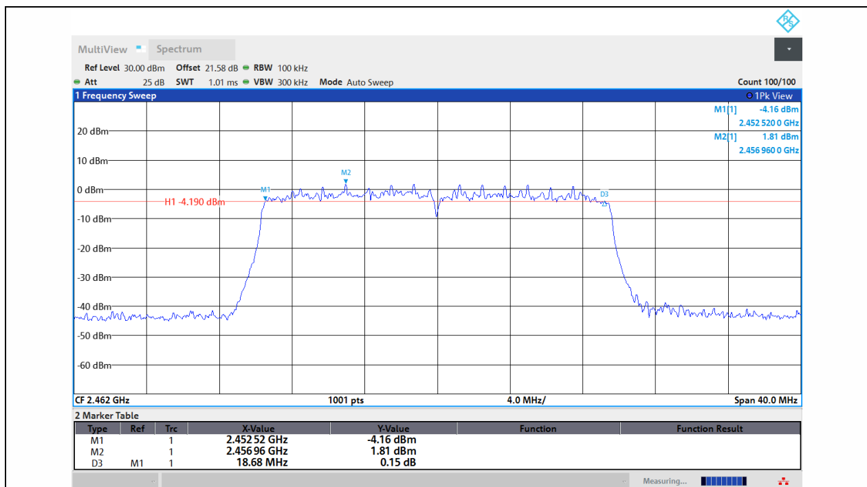
11AX20MIMO-Ant1-2462-PASS
