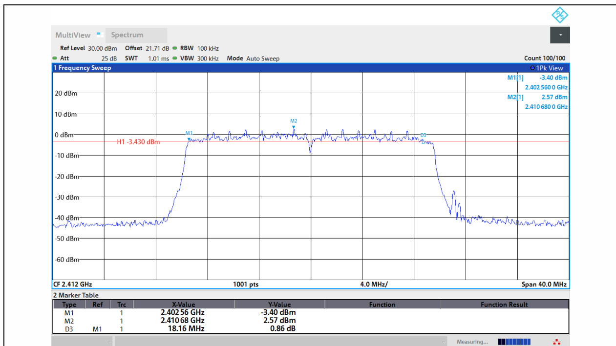
11AX20MIMO-Ant1-2412-PASS
