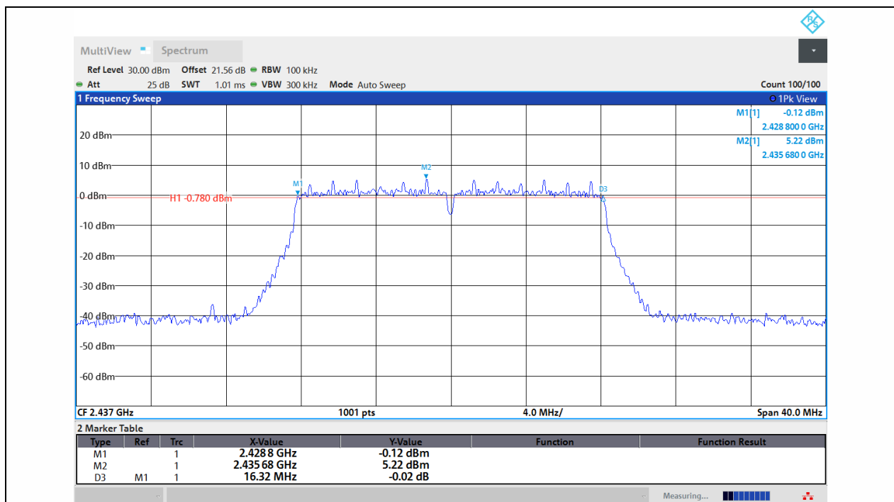
11G-Ant1-2437-PASS
