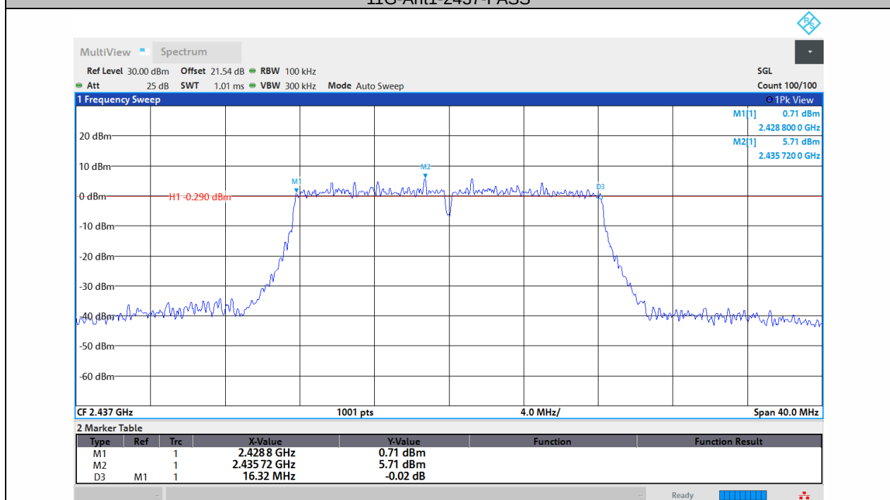
11G-Ant2-2437-PASS
