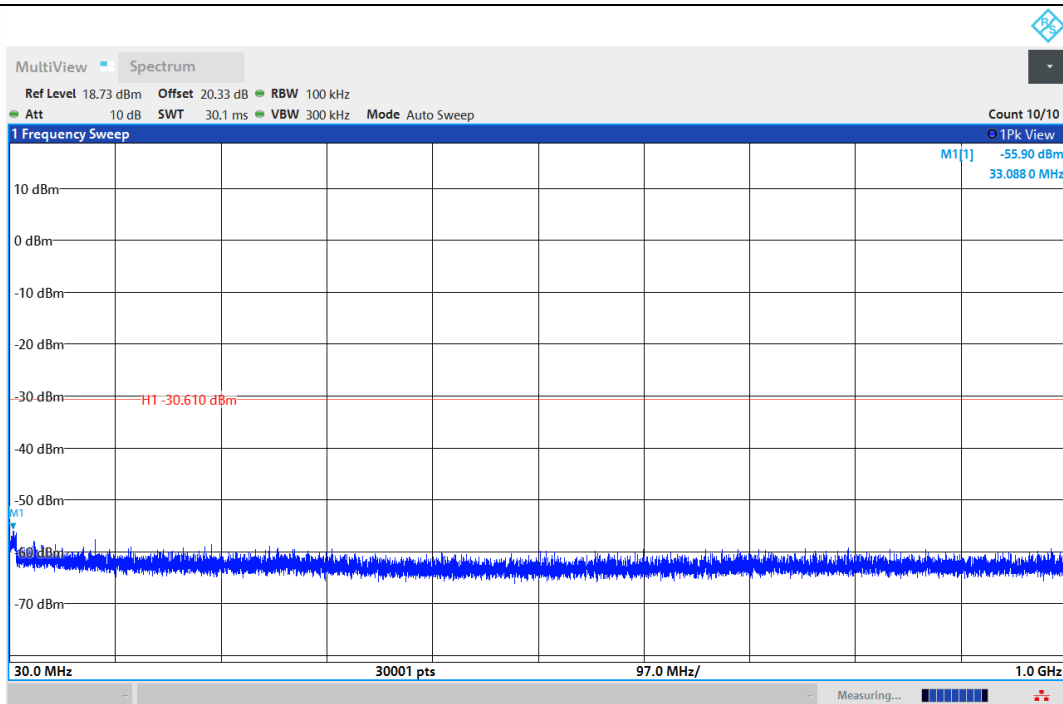
11AX40MIMO-Ant1-2422-30~1000-PASS
