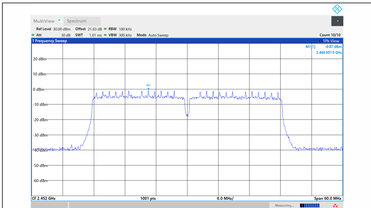
11N40MIMO-Ant1-2452-0~Reference-PASS
