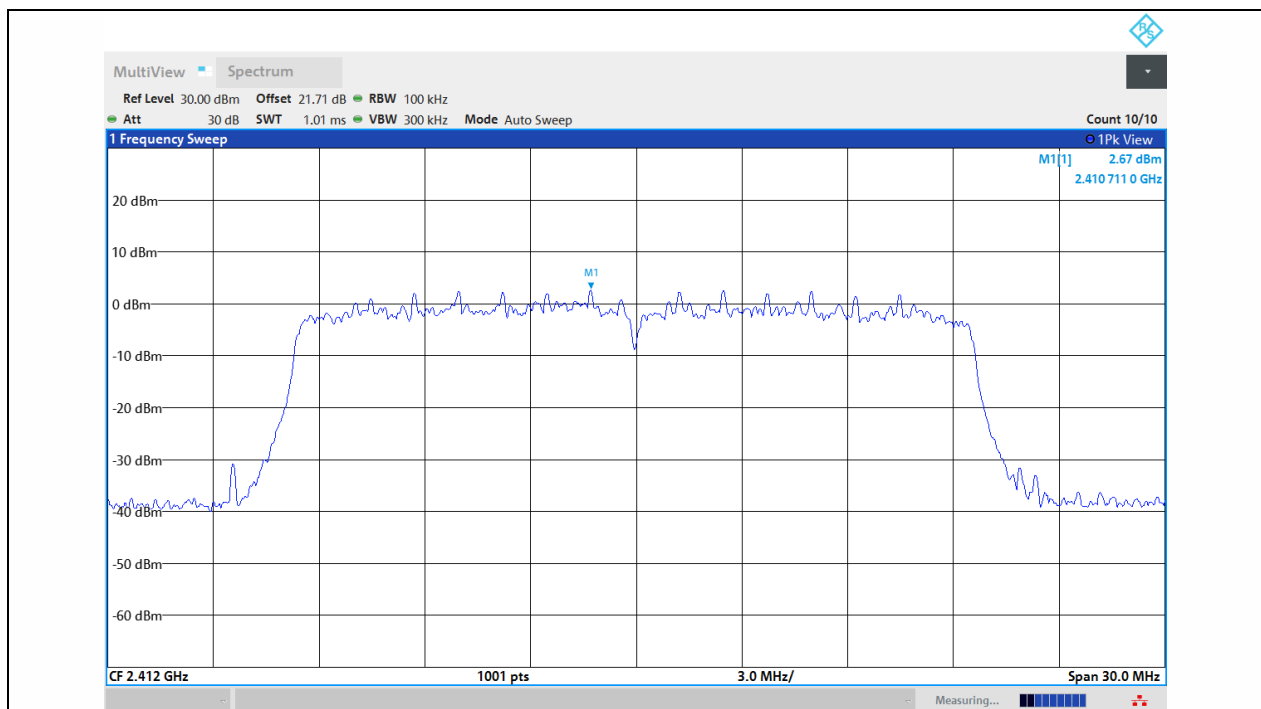
11AX20MIMO-Ant1-2412-0~Reference-PASS
