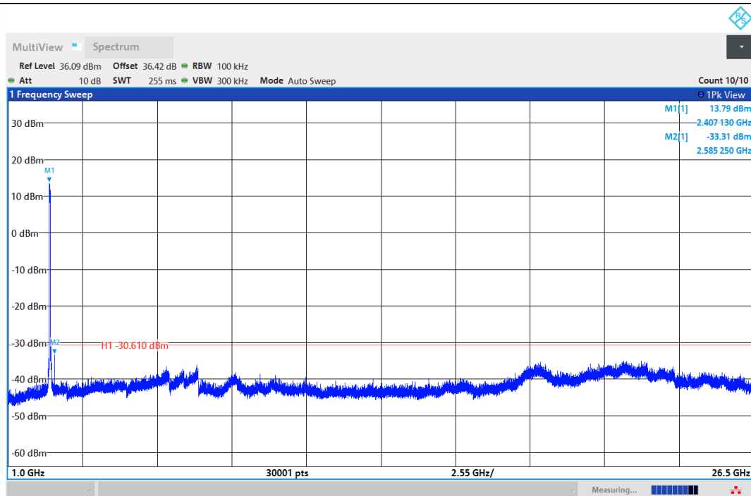
11AX40MIMO-Ant1-2422-1000~26500-PASS
