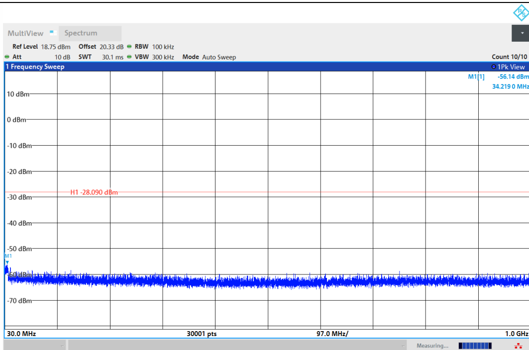
11AX20MIMO-Ant1-2462-30~1000-PASS
