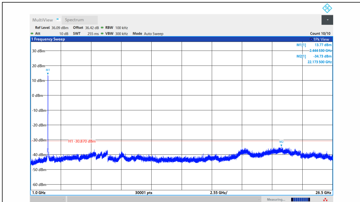
11N40MIMO-Ant1-2452-1000~26500-PASS
