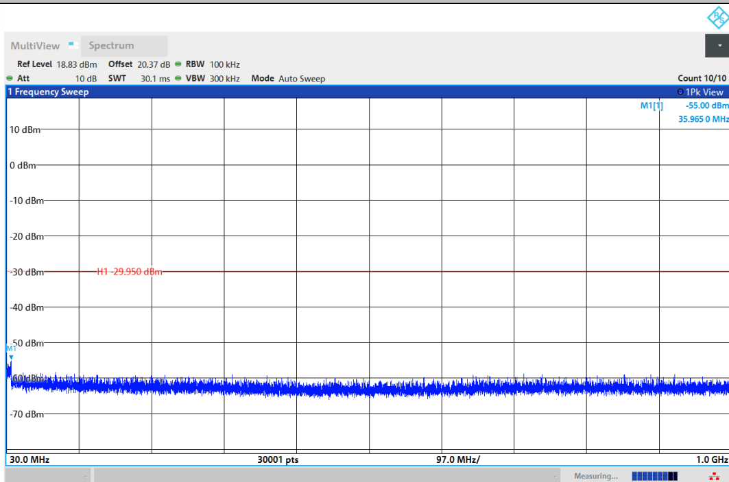
11AX40MIMO-Ant2-2437-30~1000-PASS
