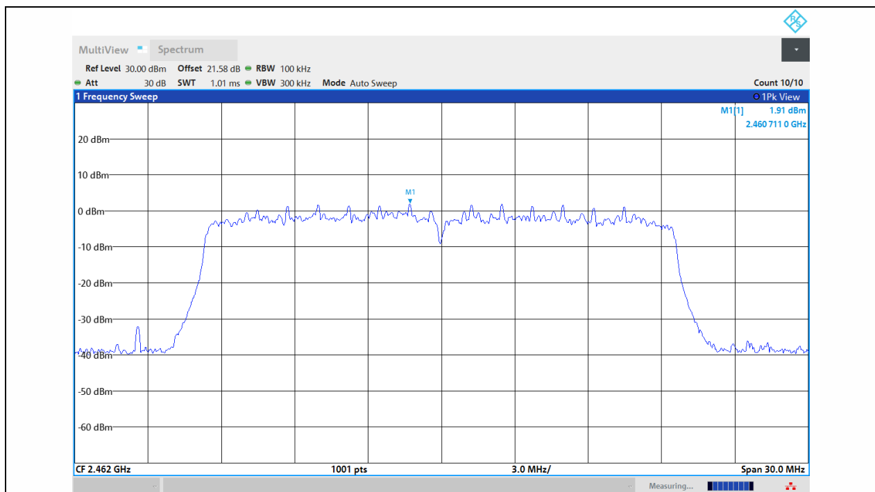
11AX20MIMO-Ant1-2462-0~Reference-PASS
