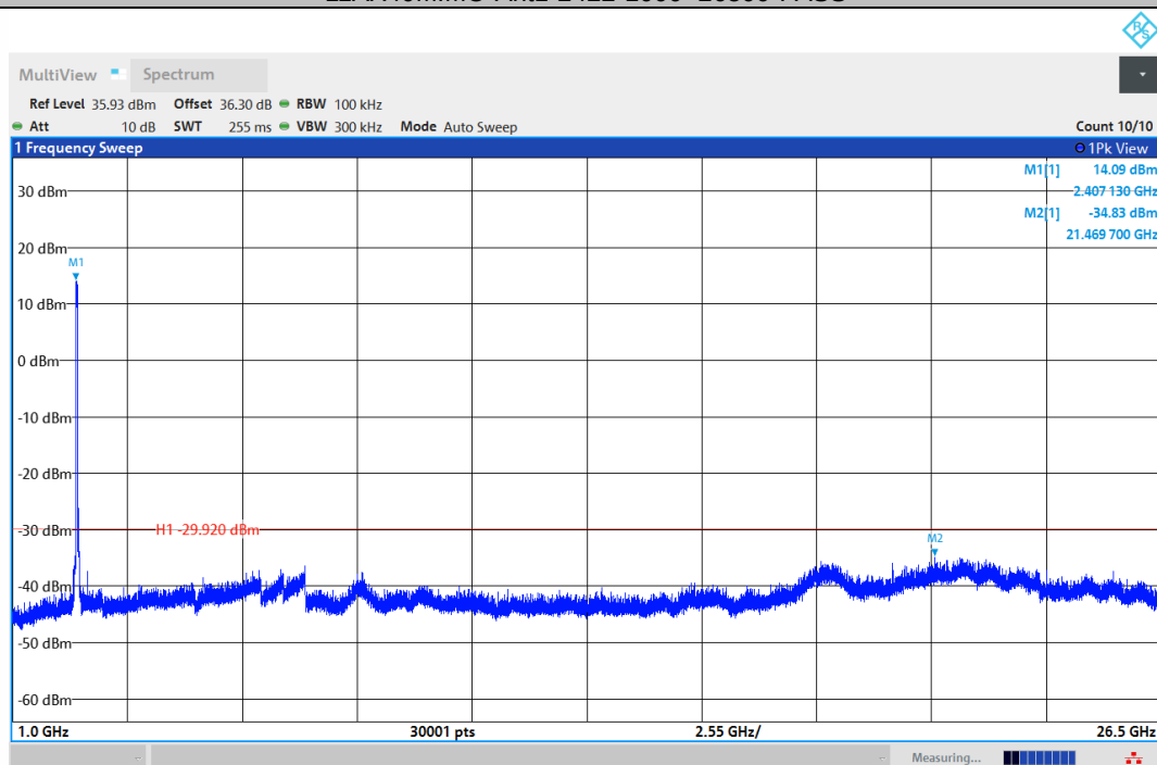
11AX40MIMO-Ant2-2422-1000~26500-PASS
