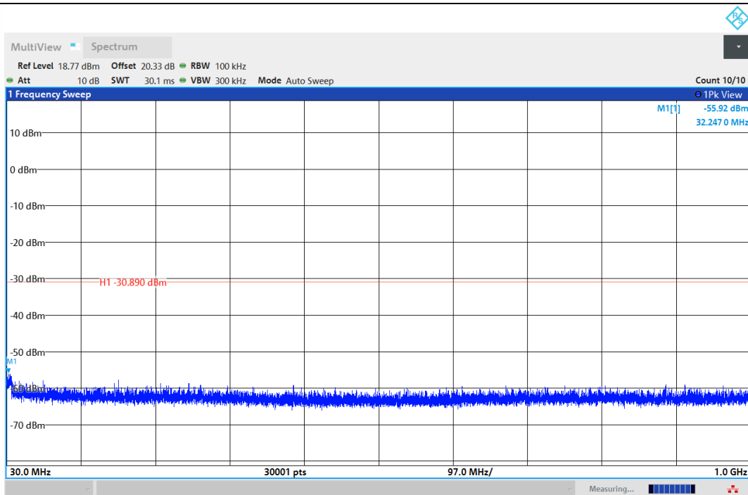
11AX40MIMO-Ant1-2437-30~1000-PASS
