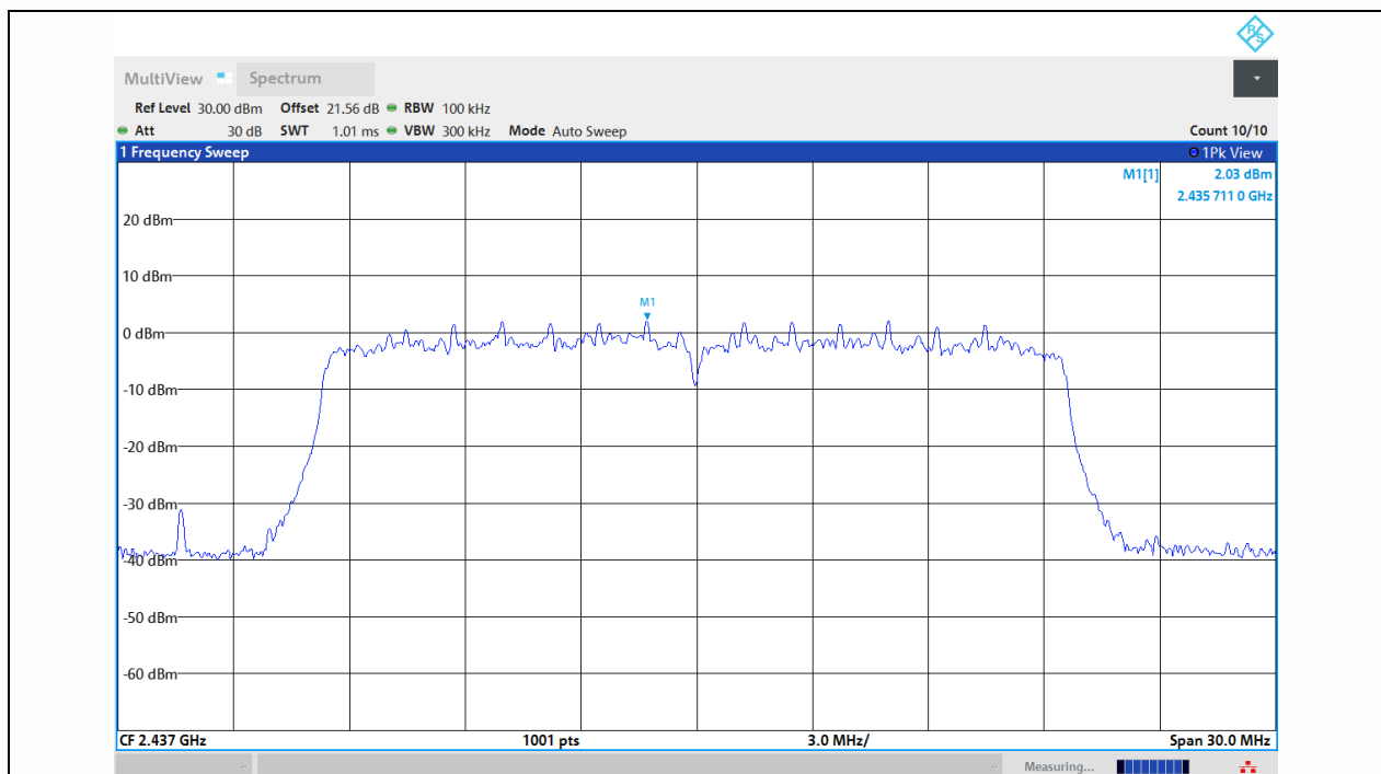
11AX20MIMO-Ant1-2437-0~Reference-PASS
