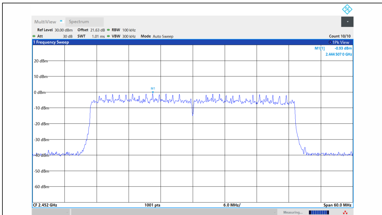
11AX40MIMO-Ant1-2452-0~Reference-PASS
