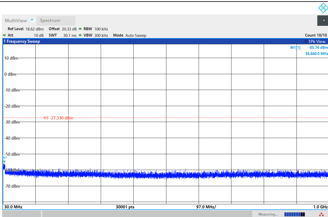
11AX20MIMO-Ant1-2412-30~1000-PASS
