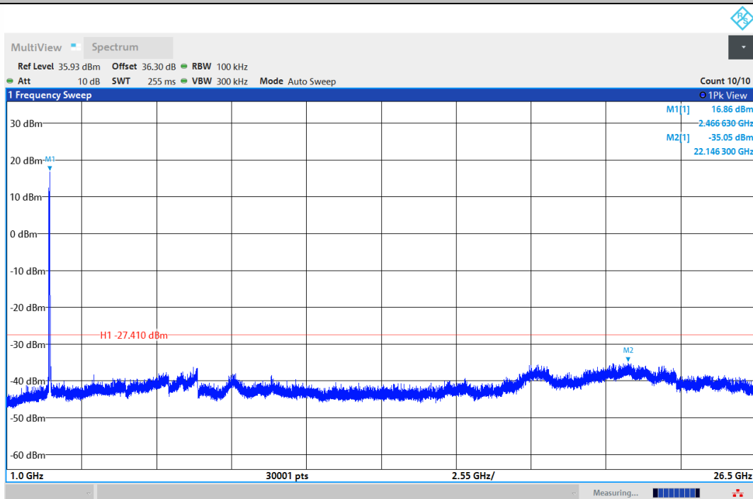
11AX20MIMO-Ant2-2462-1000~26500-PASS
