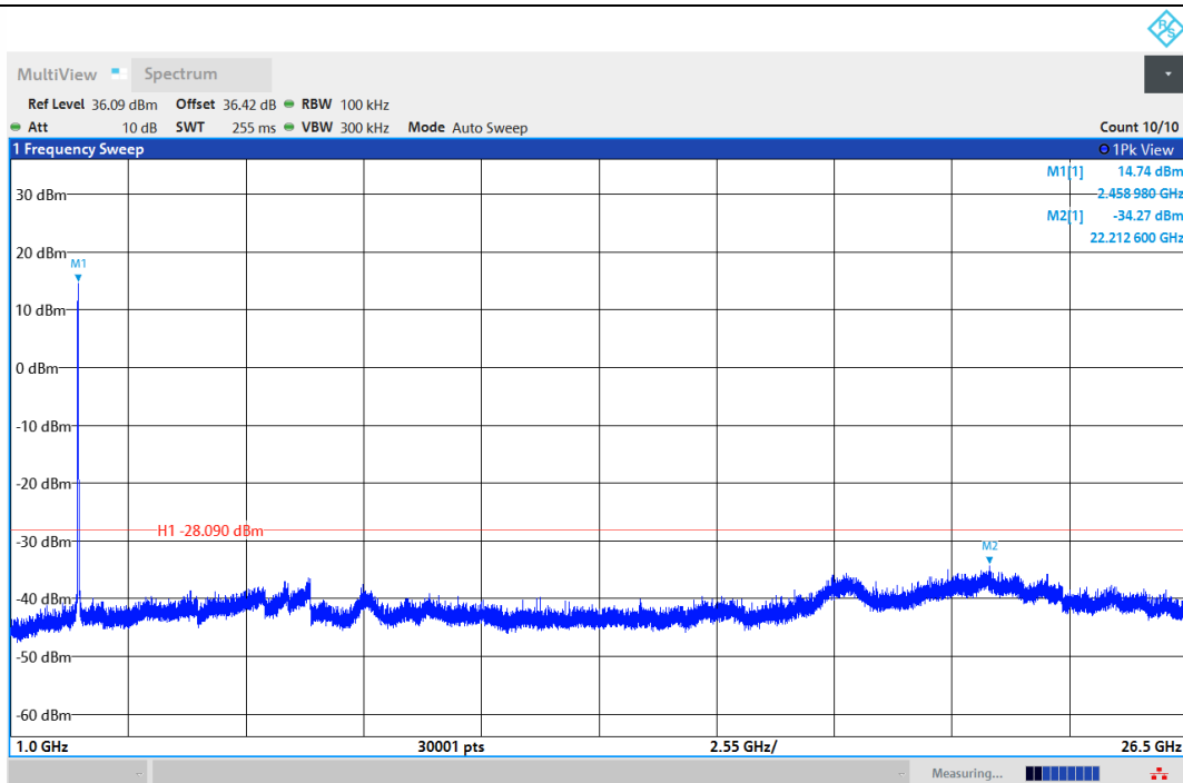
11AX20MIMO-Ant1-2462-1000~26500-PASS
