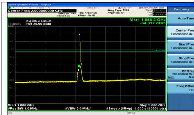
Band2-15MHz-16QAM-18675-75RB#0-1000~3000-PASS
