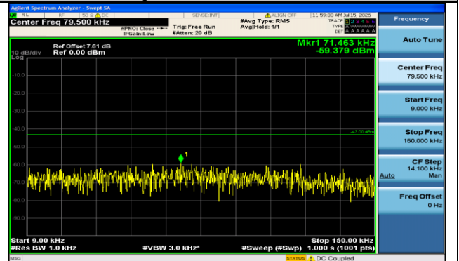
Band2-15MHz-16QAM-19125-1RB#0-0.009~0.15-PASS
