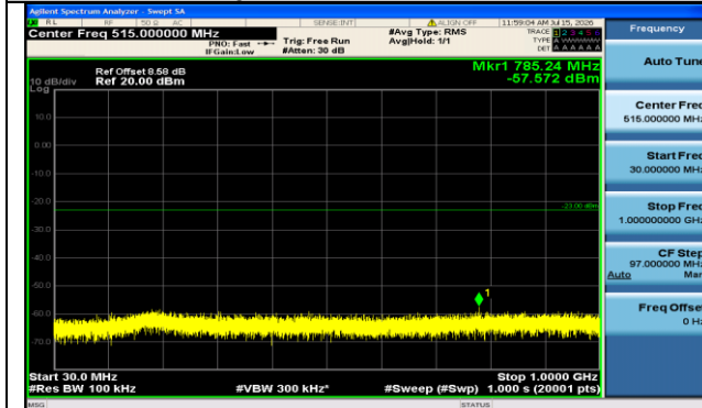
Band2-15MHz-QPSK-19125-1RB#0-30~1000-PASS
