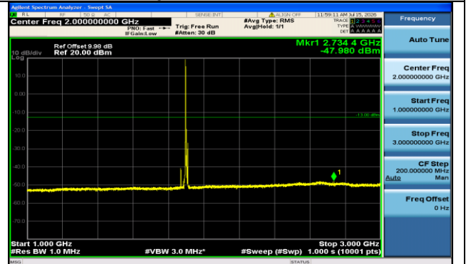
Band2-15MHz-QPSK-19125-1RB#0-1000~3000-PASS
