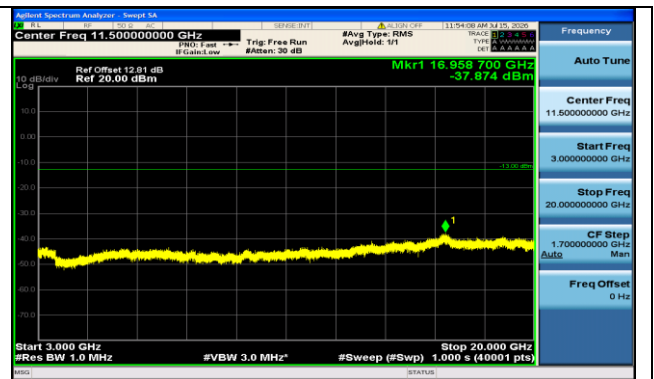
Band2-15MHz-16QAM-18675-75RB#0-3000~20000-PASS
