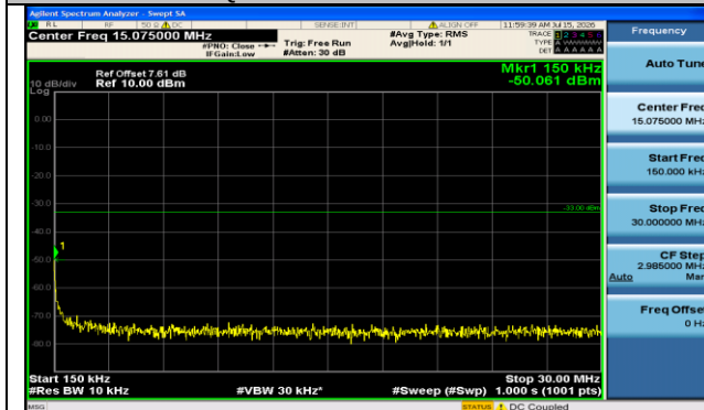
Band2-15MHz-16QAM-19125-1RB#0-0.15~30-PASS
