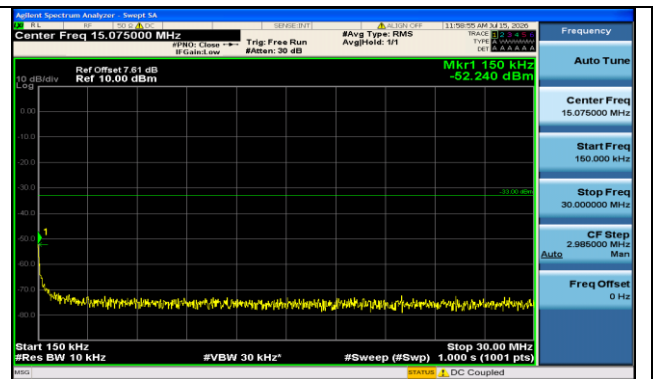
Band2-15MHz-QPSK-19125-1RB#0-0.15~30-PASS
