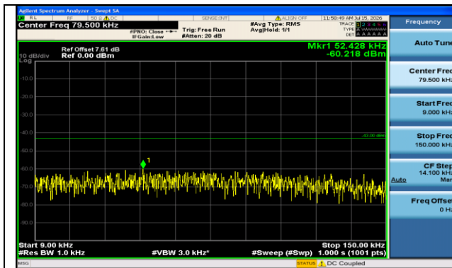
Band2-15MHz-QPSK-19125-1RB#0-0.009~0.15-PASS
