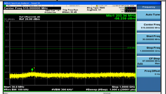
Band2-15MHz-16QAM-19125-1RB#0-30~1000-PASS
