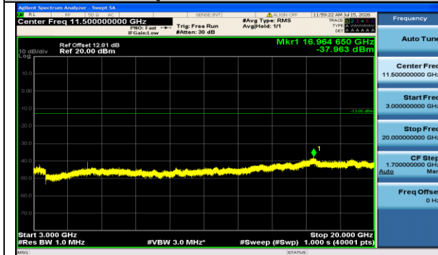
Band2-15MHz-QPSK-19125-1RB#0-3000~20000-PASS
