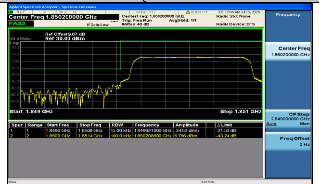
Band2-1.4MHz-16QAM-18607-6RB#0-PASS
