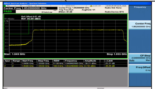
Band2-5MHz-16OAM-18625-25RB#0-PASS
