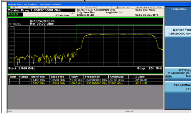
Band2-1.4MHz-QPSK-18607-6RB#0-PASS
