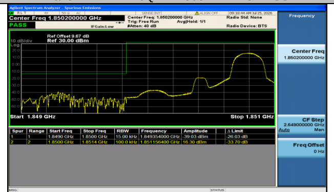
Band2-1.4MHz-16QAM-18607-1RB#5-PASS
