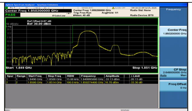
Band2-1.4MHz-16QAM-18607-1RB#0-PASS
