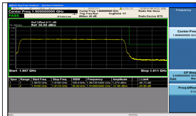
Band2-3MHz-QPSK-19185-15RB#0-PASS
