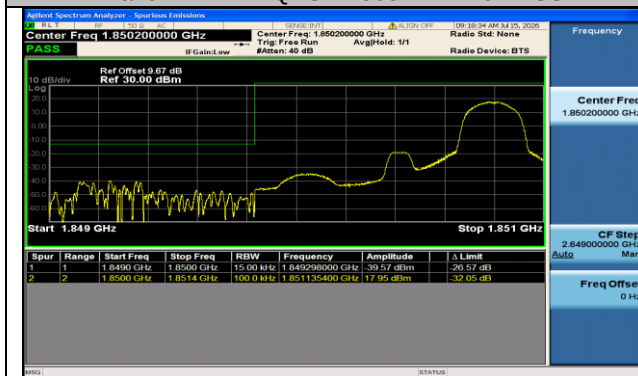
Band2-1.4MHz-QPSK-18607-1RB#5-PASS
