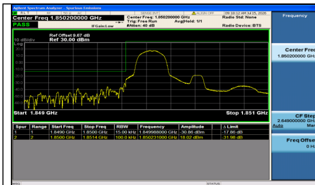
Band2-1.4MHz-QPSK-18607-1RB#0-PASS
