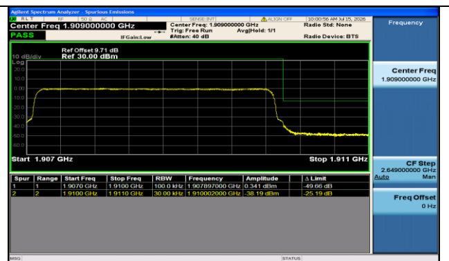
Band2-3MHz-16QAM-19185-15RB#0-PASS
