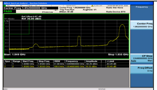
Band2-5MHz-16QAM-18625-1RB#24-PASS
