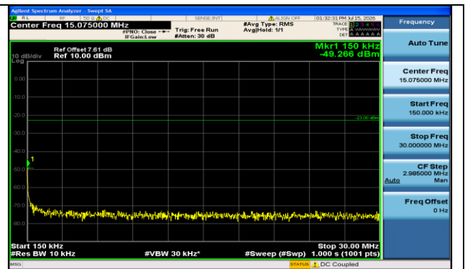
Band5-3MHz-QPSK-20635-15RB#0-0.15~30-PASS
