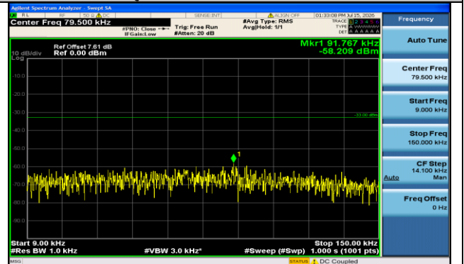
Band5-3MHz-16QAM-20635-15RB#0-0.009~0.15-PASS
