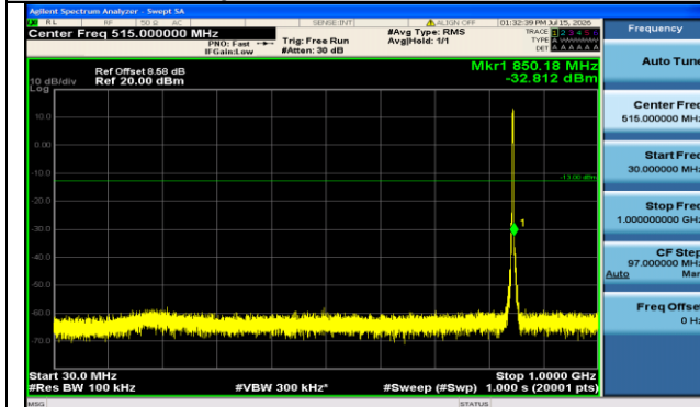
Band5-3MHz-QPSK-20635-15RB#0-30~1000-PASS
