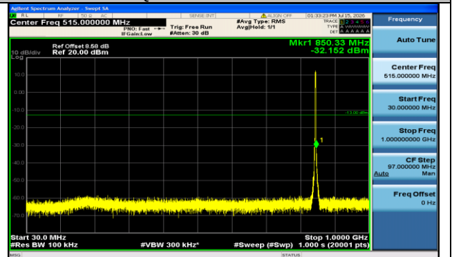
Band5-3MHz-16QAM-20635-15RB#0-30~1000-PASS
