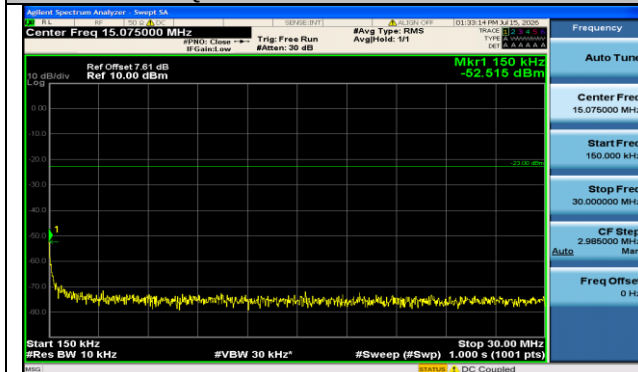
Band5-3MHz-16QAM-20635-15RB#0-0.15~30-PASS
