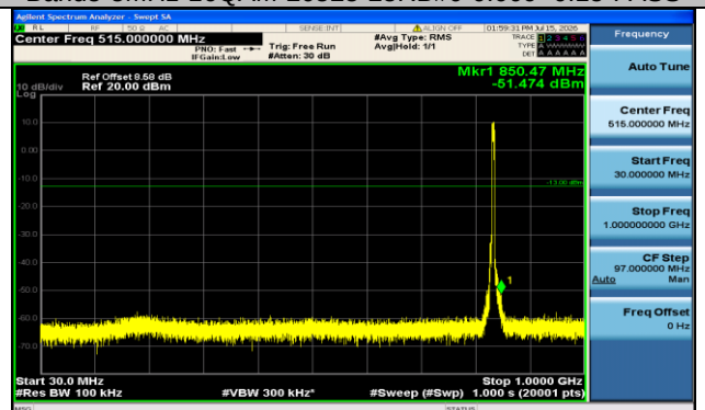
Band5-5MHz-16QAM-20525-25RB#0-30~1000-PASS
