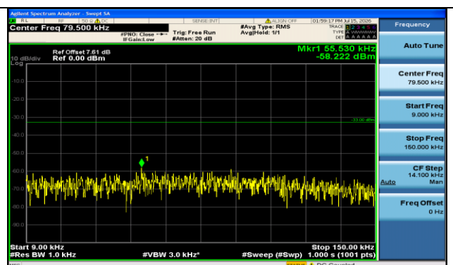
Band5-5MHz-16OAM-20525-25RB#0-0.009~0.15-PASS
