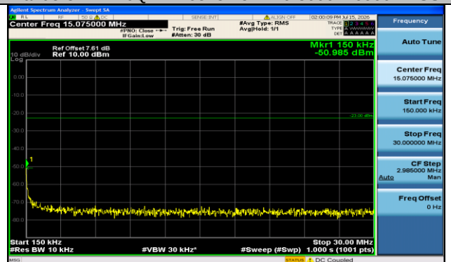
Band5-5MHz-OPSK-20625-1RB#0-0.15~30-PASS
