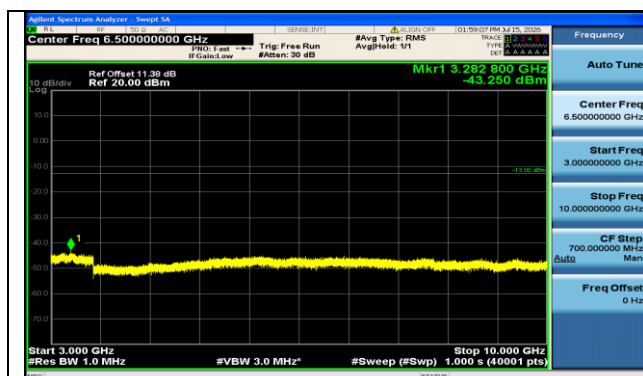
Band5-5MHz-OPSK-20525-25RB#0-3000~10000-PASS
