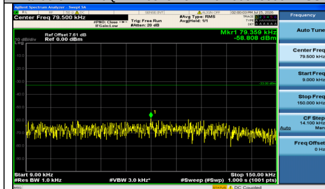
Band5-5MHz-OPSK-20625-1RB#0-0.009~0.15-PASS
