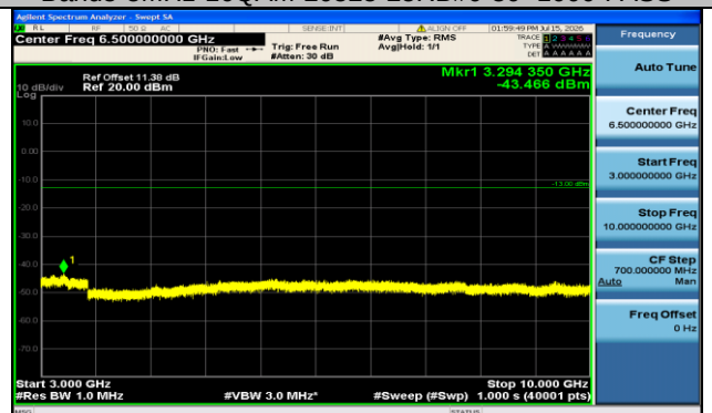
Band5-5MHz-16QAM-20525-25RB#0-3000~10000-PASS
