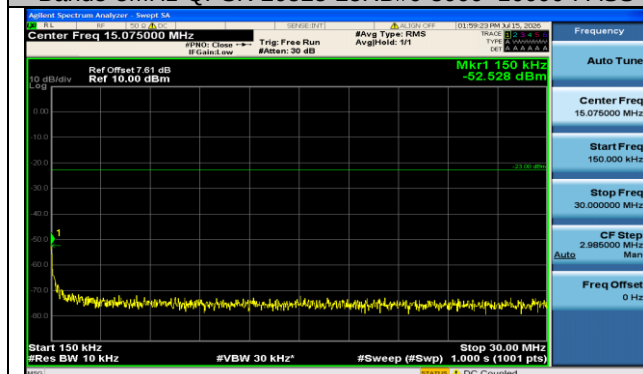
Band5-5MHz-16QAM-20525-25RB#0-0.15~30-PASS
