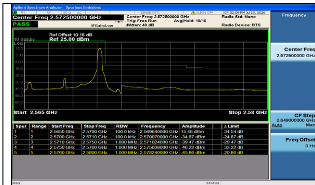
Band7-5MHz-QPSK-21425-1RB#24-PASS
