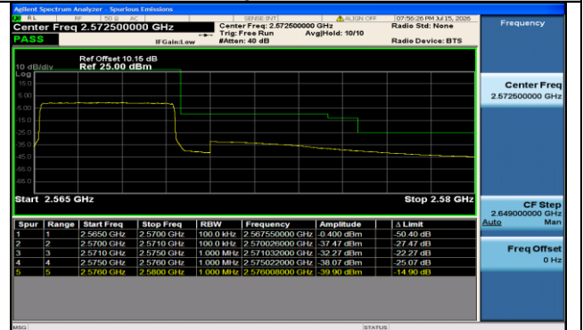
Band7-5MHz-16QAM-21425-25RB#0-PASS
