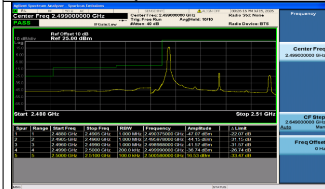
Band7-10MHz-QPSK-20800-1RB#0-PASS
