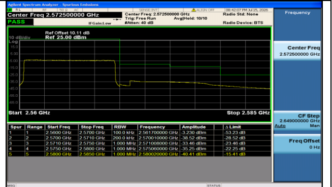
Band7-10MHz-16QAM-21400-50RB#0-PASS
