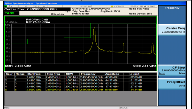
Band7-10MHz-16QAM-20800-1RB#0-PASS
