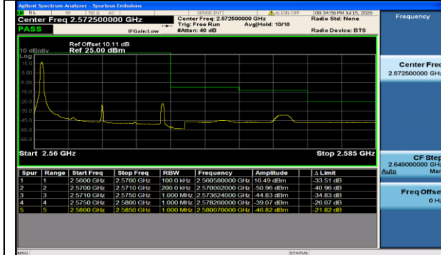
Band7-10MHz-QPSK-21400-1RB#0-PASS
