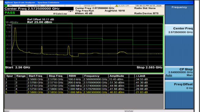
Band7-10MHz-16QAM-21400-1RB#0-PASS
