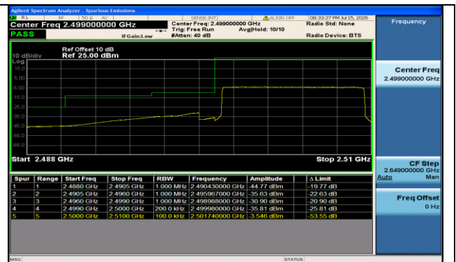
Band7-10MHz-16QAM-20800-50RB#0-PASS
