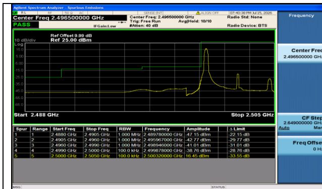
Band7-5MHz-QPSK-20775-1RB#0-PASS
