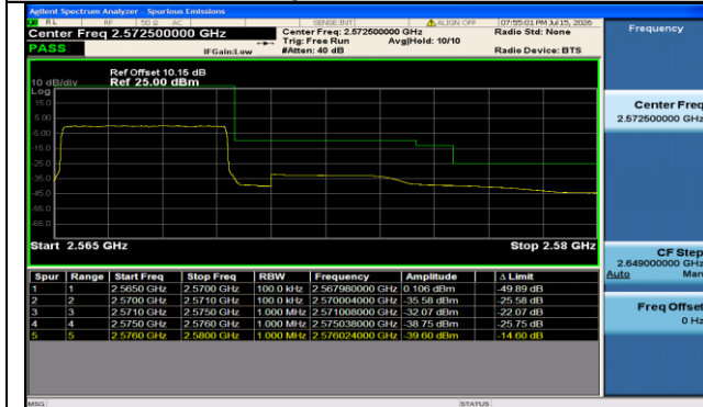
Band7-5MHz-QPSK-21425-25RB#0-PASS
