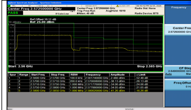
Band7-10MHz-QPSK-21400-50RB#0-PASS
