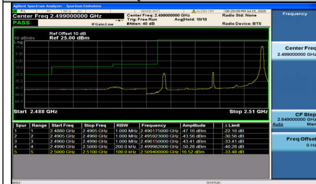
Band7-10MHz-QPSK-20800-1RB#49-PASS
