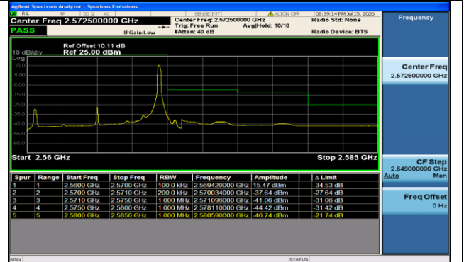
Band7-10MHz-16QAM-21400-1RB#49-PASS
