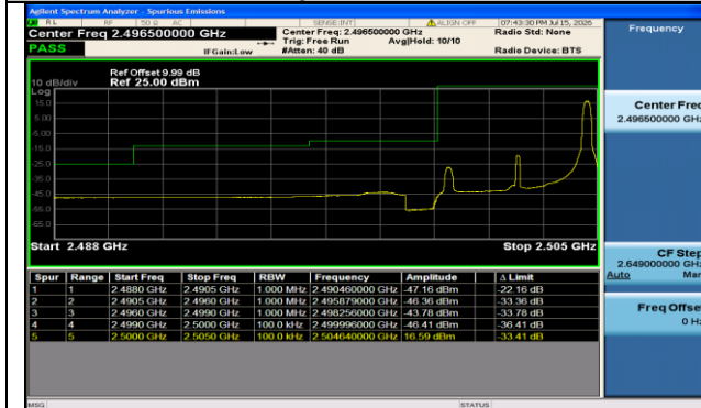
Band7-5MHz-QPSK-20775-1RB#24-PASS
