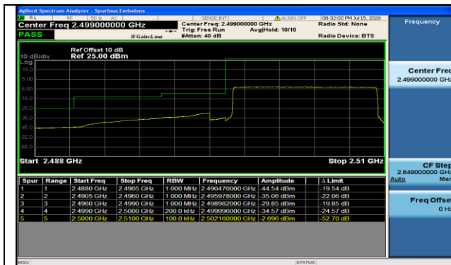
Band7-10MHz-QPSK-20800-50RB#0-PASS
