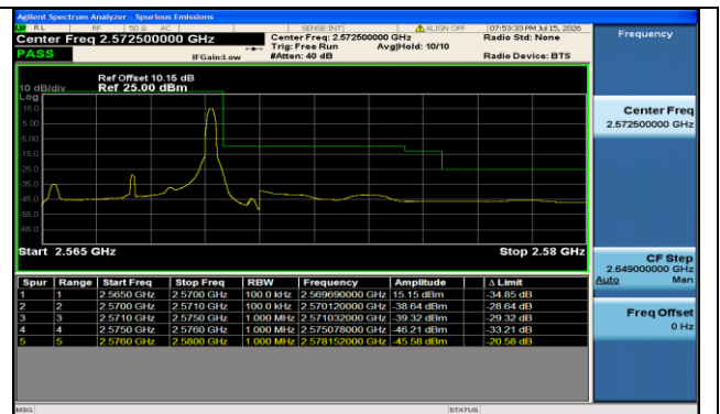
Band7-5MHz-16QAM-21425-1RB#24-PASS
