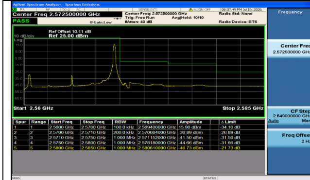
Band7-10MHz-QPSK-21400-1RB#49-PASS
