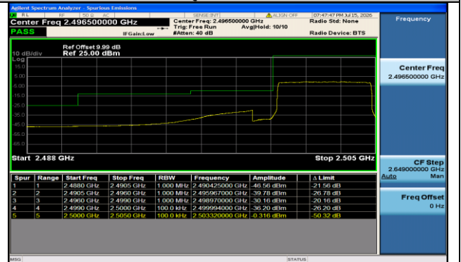
Band7-5MHz-16QAM-20775-25RB#0-PASS
