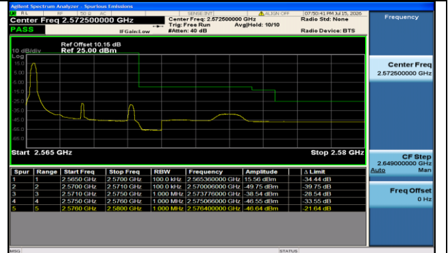
Band7-5MHz-16QAM-21425-1RB#0-PASS
