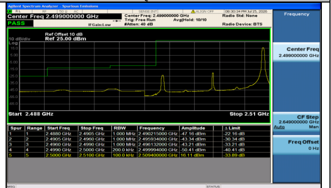
Band7-10MHz-16QAM-20800-1RB#49-PASS
