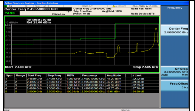
Band7-5MHz-16QAM-20775-1RB#24-PASS
