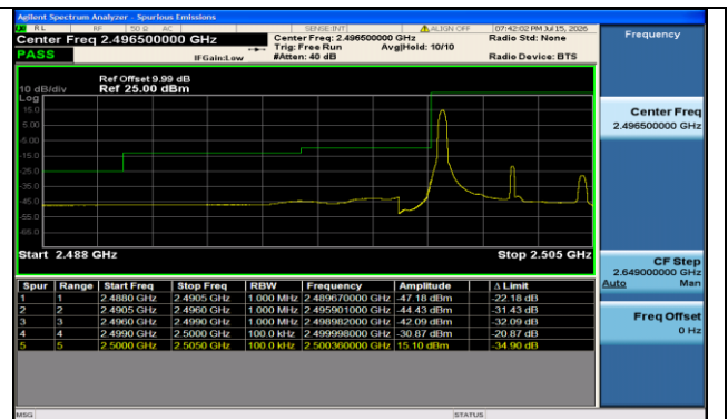
Band7-5MHz-16QAM-20775-1RB#0-PASS
