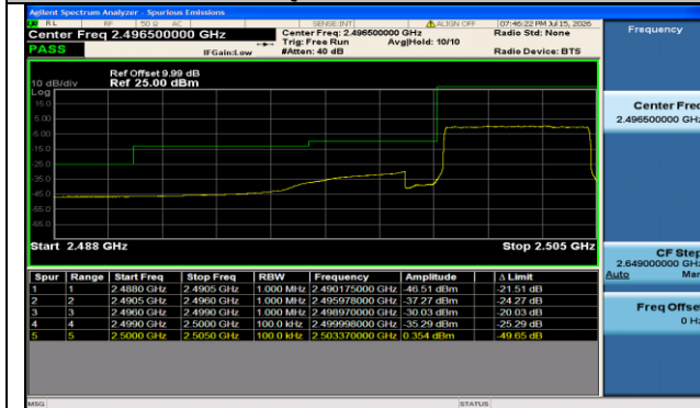
Band7-5MHz-QPSK-20775-25RB#0-PASS
