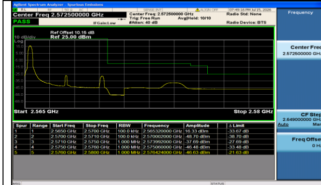
Band7-5MHz-QPSK-21425-1RB#0-PASS
