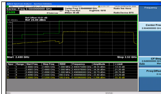
Band7-20MHz-QPSK-20850-100RB#0-PASS
