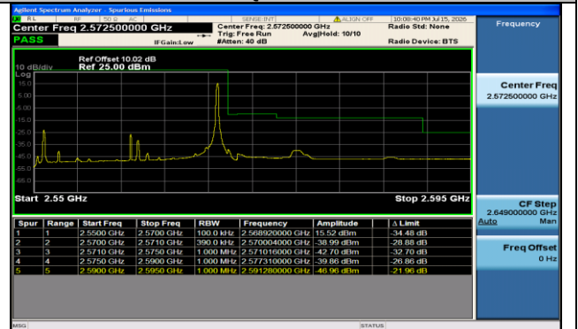
Band7-20MHz-16QAM-21350-1RB#99-PASS
