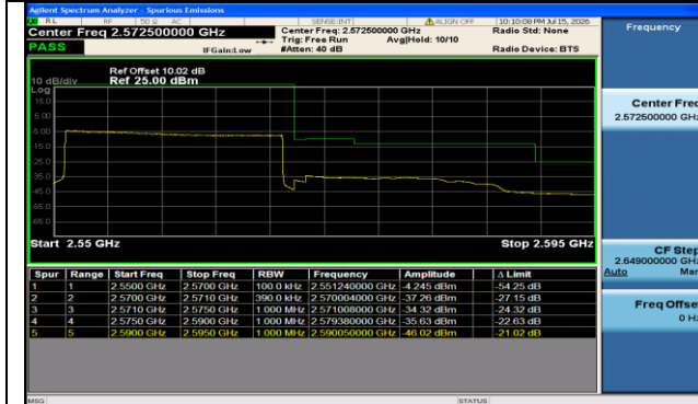
Band7-20MHz-QPSK-21350-100RB#0-PASS
