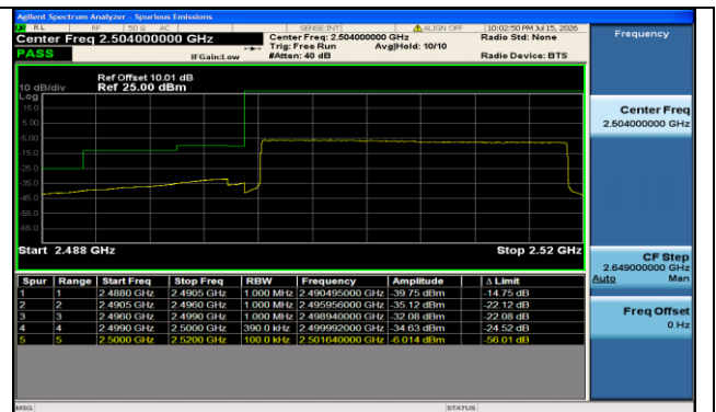
Band7-20MHz-16QAM-20850-100RB#0-PASS
