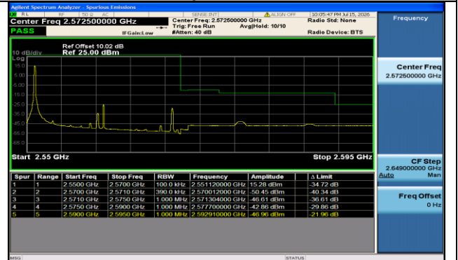
Band7-20MHz-16QAM-21350-1RB#0-PASS
