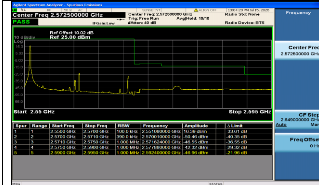
Band7-20MHz-QPSK-21350-1RB#0-PASS
