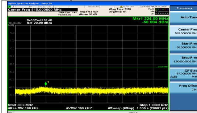
Band7-10MHz-16QAM-20800-50RB#0-30~1000-PASS
