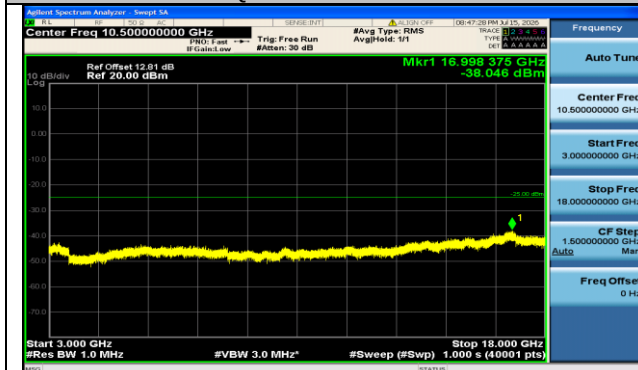
Band7-10MHz-16QAM-20800-50RB#0-3000~18000-PASS
