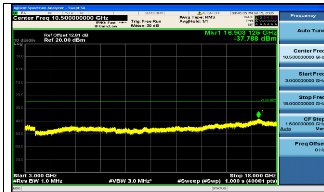
Band7-10MHz-QPSK-20800-50RB#0-3000~18000-PASS
