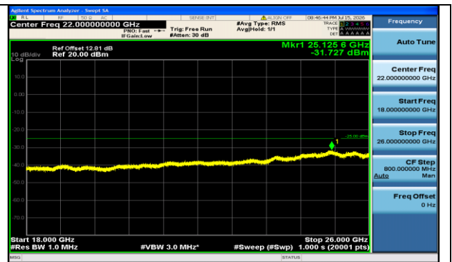
Band7-10MHz-QPSK-20800-50RB#0-18000~26000-PASS
