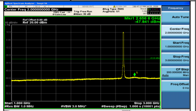
Band7-10MHz-16QAM-20800-50RB#0-1000~3000-PASS
