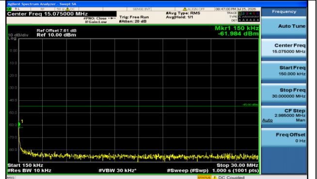
Band7-10MHz-16QAM-20800-50RB#0-0.15~30-PASS
