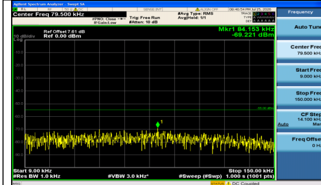
Band7-10MHz-16QAM-20800-50RB#0-0.009~0.15-PASS
