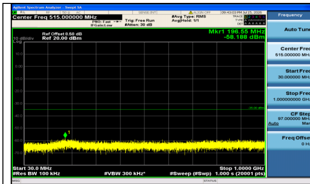
Band7-15MHz-16QAM-21375-75RB#0-30~1000-PASS
