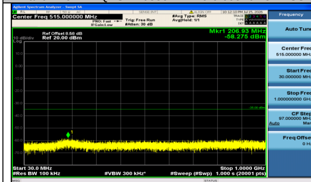
Band7-20MHz-QPSK-20850-1RB#0-30~1000-PASS
