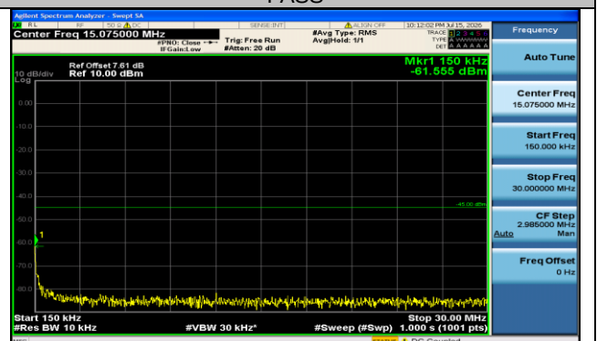
Band7-20MHz-QPSK-20850-1RB#0-0.15~30-PASS
