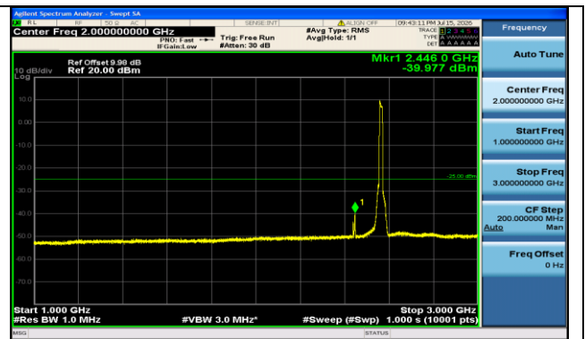
Band7-15MHz-16QAM-21375-75RB#0-1000~3000-PASS
