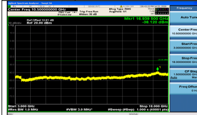
Band7-15MHz-16QAM-21375-75RB#0-3000~18000-PASS
