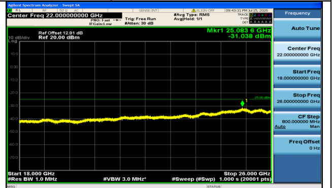
Band7-15MHz-16QAM-21375-75RB#0-18000~26000-PASS
