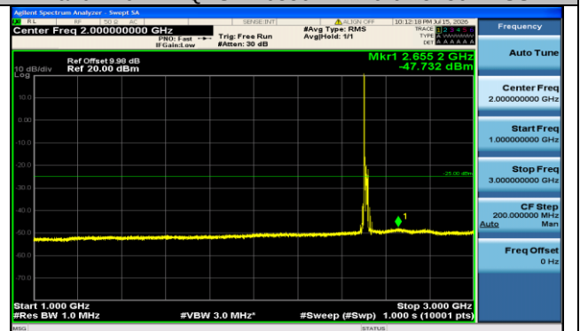
Band7-20MHz-QPSK-20850-1RB#0-1000~3000-PASS
