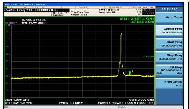
Band7-20MHz-16QAM-21100-100RB#0-1000~3000-PASS
