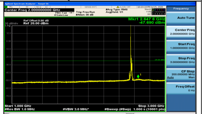
Band7-20MHz-QPSK-21350-1RB#0-1000~3000-PASS
