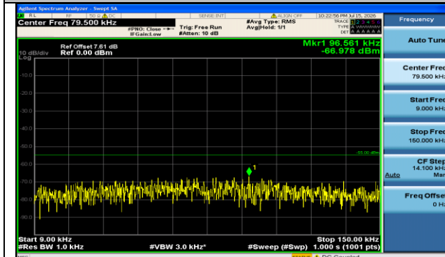
Band7-20MHz-QPSK-21350-1RB#0-0.009~0.15-PASS
