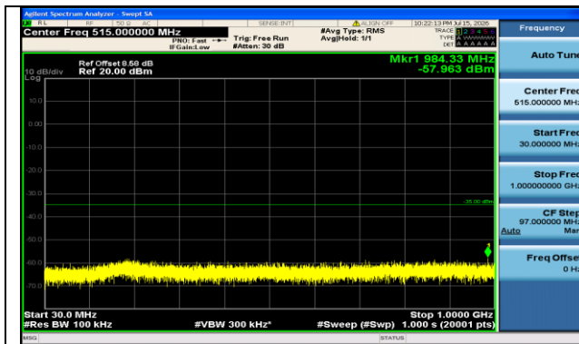
Band7-20MHz-16QAM-21100-100RB#0-30~1000-PASS
