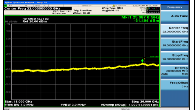
Band7-20MHz-16QAM-21100-100RB#0-18000~26000-PASS
