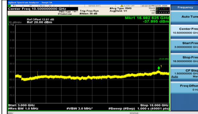
Band7-20MHz-16QAM-21100-100RB#0-3000~18000-PASS
