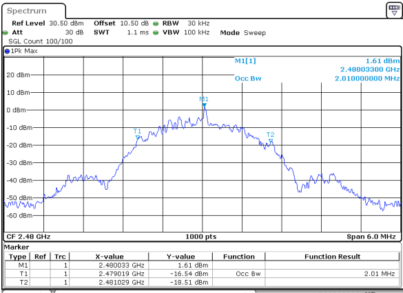
BLE_2M_High_Channel
