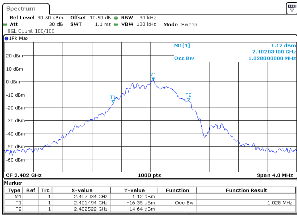
BLE_1M_Low_Channel
