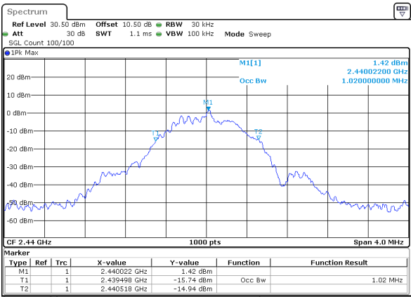
BLE_1M_Middle_Channel
