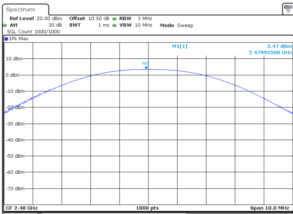
BLE_1M_High_Channel
