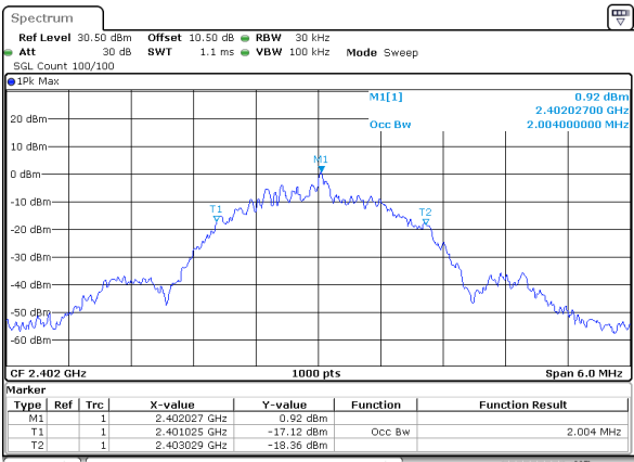
BLE_2M_Low_Channel
