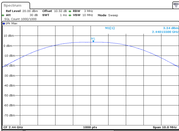
BLE_2M_Middle_Channel
