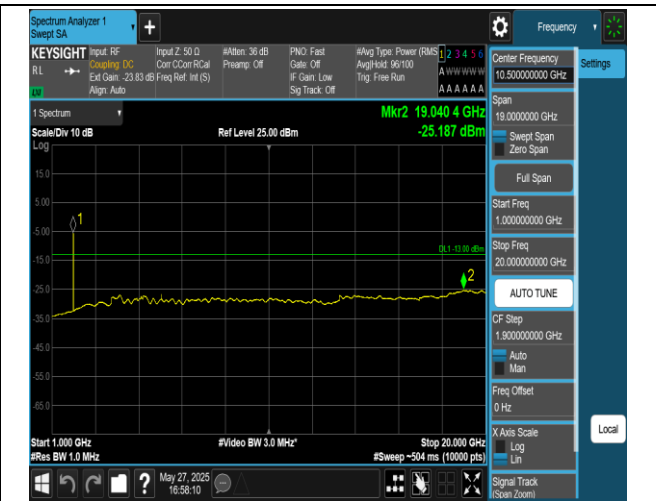
Band25-5MHz-QPSK-8365-E-TM1.1-1000~20000
