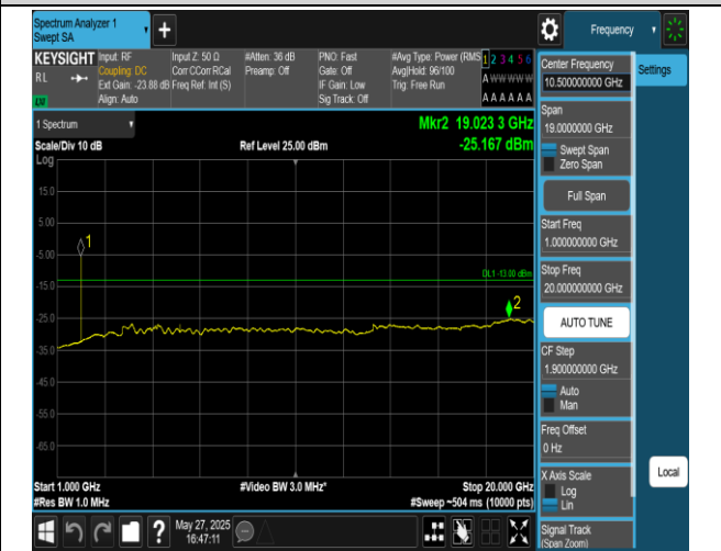
Band25-5MHz-QPSK-8665-E-TM1.1-1000~20000
