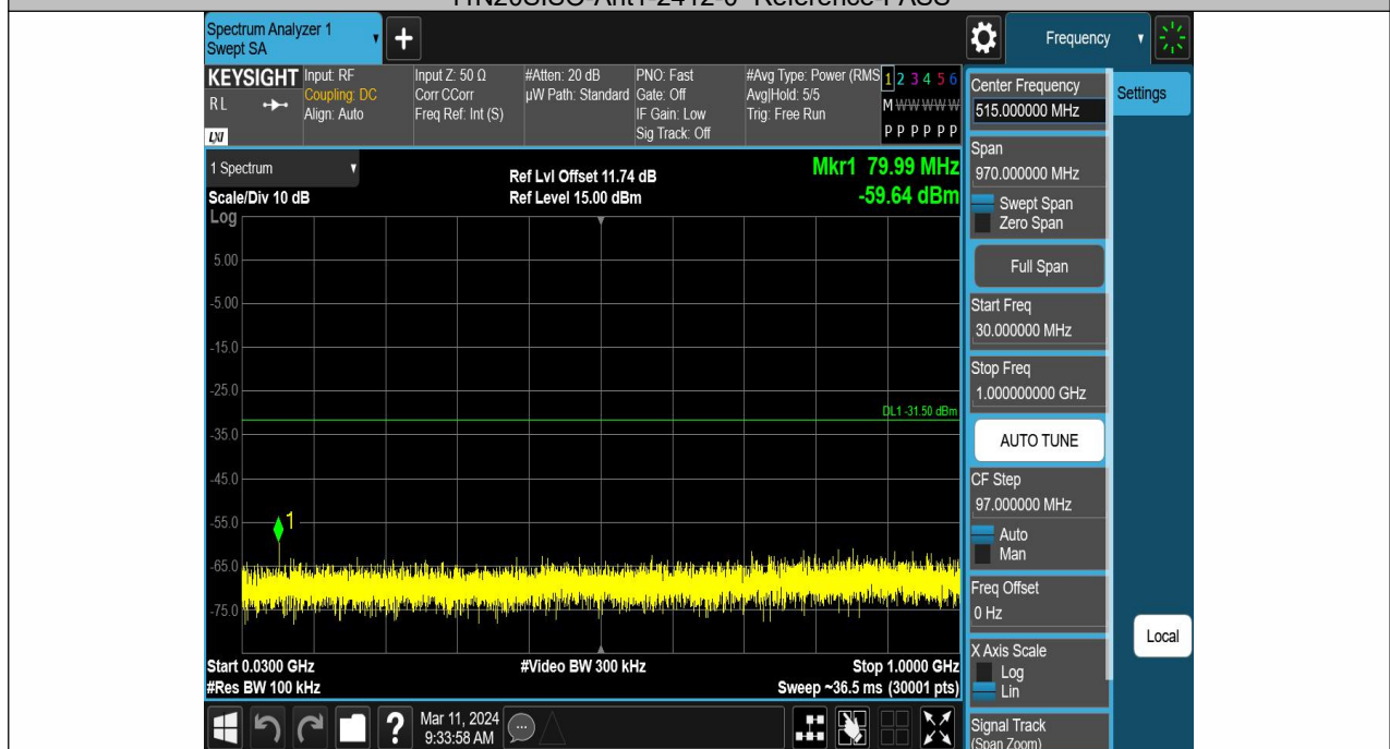
11N20SISO-Ant1-2412-30~1000-PASS
