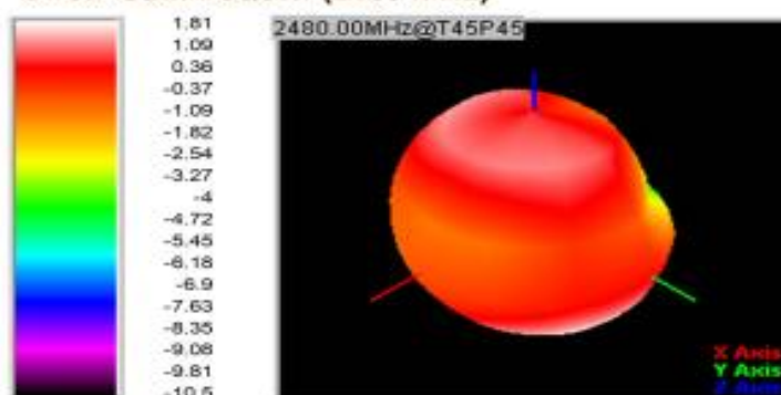
© 3D Gain Pattern (2480 MHz)
