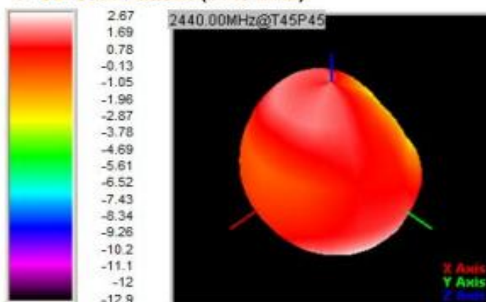
© 3D Gain Pattern (2440 MHz)
