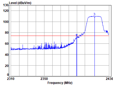
11n_HT(20M)_TX_CH_01_Horizontal-Peak
