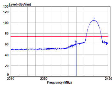
11b_TX_CH_01_Vertical-Peak
