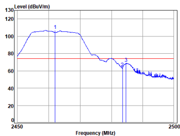
11g_TX_CH_11_Vertical-Peak
