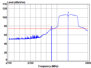
11n_HT(40M)_TX_CH_03_Horizontal-Peak
