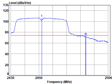
11n_HT(40M)_TX_CH_09_Horizontal-Peak
