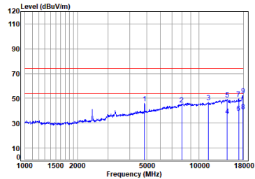
11g_TX_CH_06_Vertical
