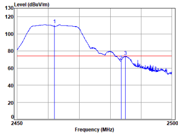
11g_TX_CH_11_Horizontal-Peak
