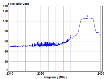
11n_HT(20M)_TX_CH_01_Vertical-Peak
