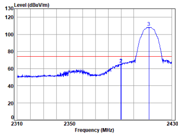
11b_TX_CH_01_Horizontal-Peak
