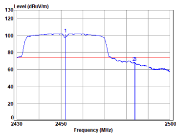
11n_HT(40M)_TX_CH_09_Vertical-Peak
