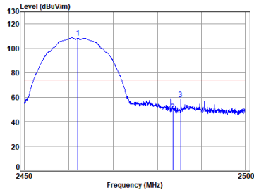
11b_TX_CH_11_Horizontal-Peak
