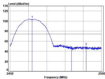
11b_TX_CH_11_Vertical-Peak
