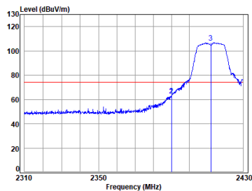
11g_TX_CH_01_Vertical-Peak
