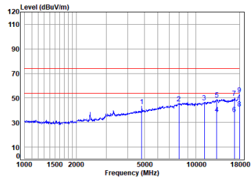
11g_TX_CH_01_Vertical
