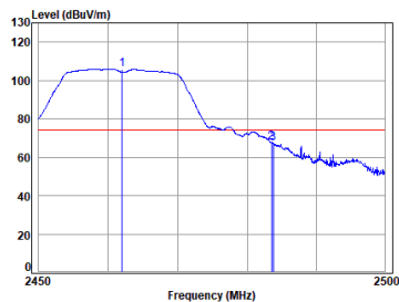
11n_HT(20M)_TX_CH_11_Vertical-Peak
