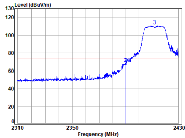
11g_TX_CH_01_Horizontal-Peak
