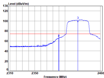
11n_HT(40M)_TX_CH_03_Vertical-Peak
