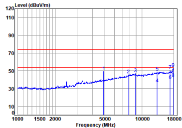
11g_TX_CH_11_Vertical
