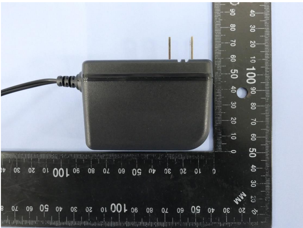
(8) EUT Photo (Brand: UNIFIVE CO., LTD., M/N: UMVU3012-050020SA)
