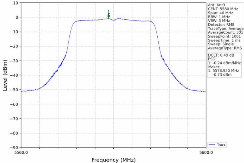
802.11ac(VHT20)_MCH_5580MHz_MIMO_NTNV
