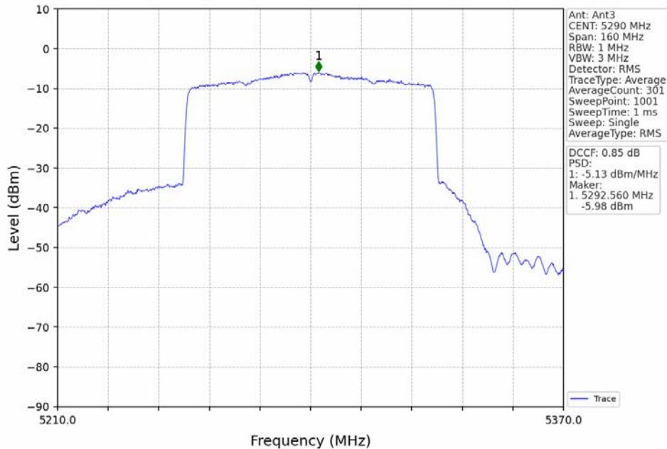
802.11ax(HEW80)_MCH_5290MHz_RU996_Left_MIMO_NTNV
