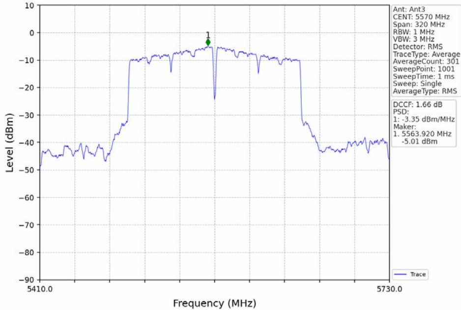
802.11ac(VHT160)_MCH_5570MHz_MIMO_NTNV
