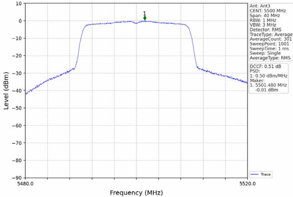
802.11ax(HEW20)_LCH_5500MHz_RU242_Left_MIMO_NTNV
