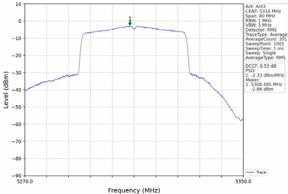
802.11ax(HEW40)_HCH_5310MHz_RU484_Left_MIMO_NTNV
