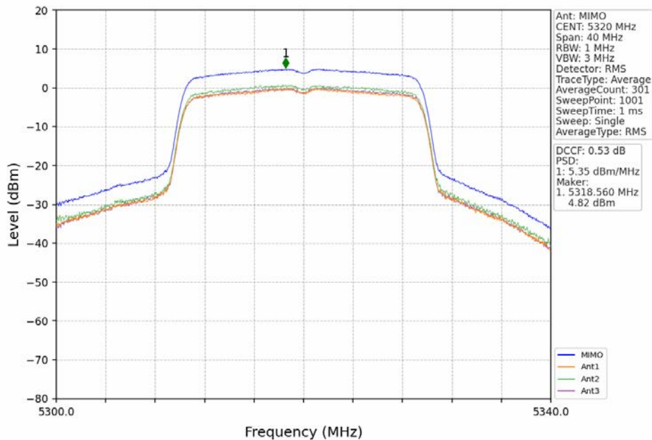
802.11ax(HEW20)_HCH_5320MHz_RU242_Left_MIMO_NTNV
