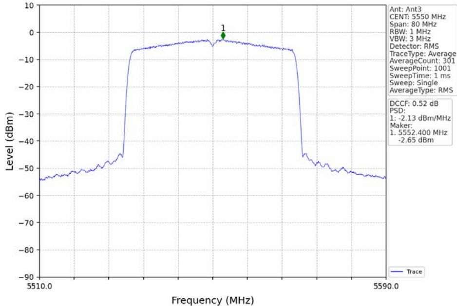
802.11ax(HEW40)_MCH_5550MHz_RU484_Left_MIMO_NTNV
