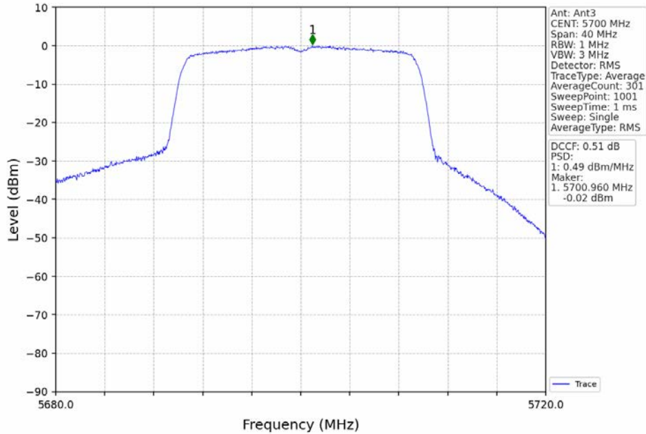
802.11ax(HEW20)_HCH_5700MHz_RU242_Left_MIMO_NTNV
