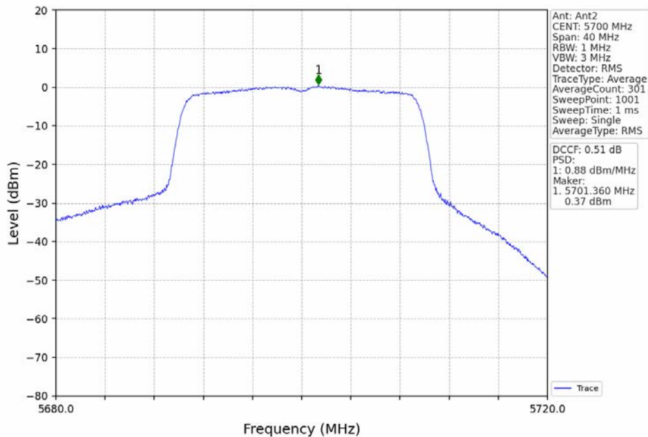
802.11ax(HEW20)_HCH_5700MHz_RU242_Left_Ant2_NTNV
