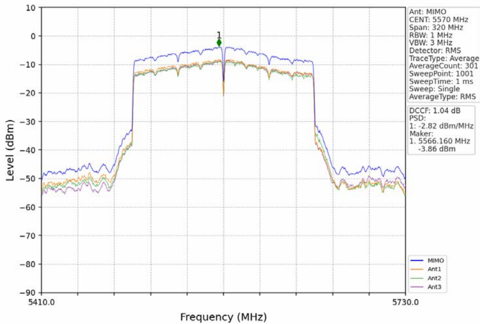
802.11ax(HEW160)_MCH_5570MHz_2xRU996_Left_MIMO_NTNV
