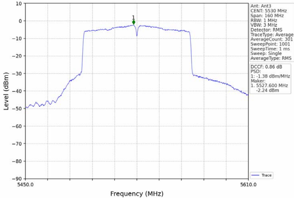
802.11ac(VHT80)_LCH_5530MHz_MIMO_NTNV
