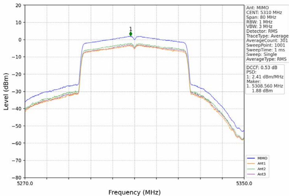
802.11ax(HEW40)_HCH_5310MHz_RU484_Left_MIMO_NTNV
