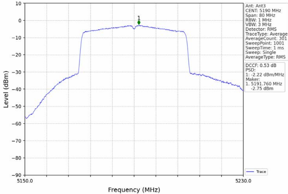
802.11ax(HEW40)_LCH_5190MHz_RU484_Left_MIMO_NTNV
