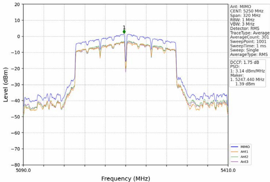
802.11ac(VHT160)_MCH_5250MHz_MIMO_NTNV
