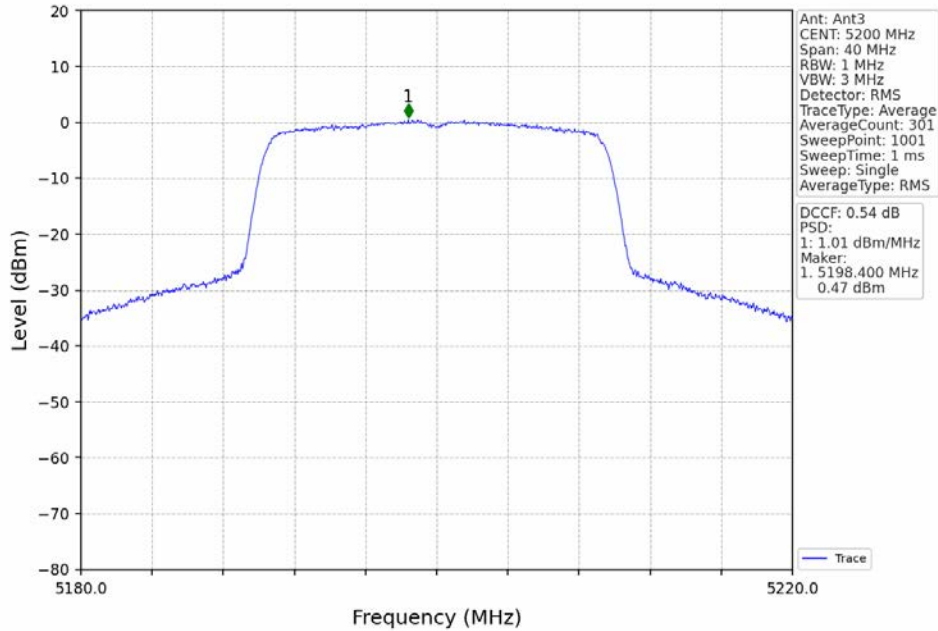
802.11ax(HEW20)_MCH_5200MHz_RU242_Left_MIMO_NTNV
