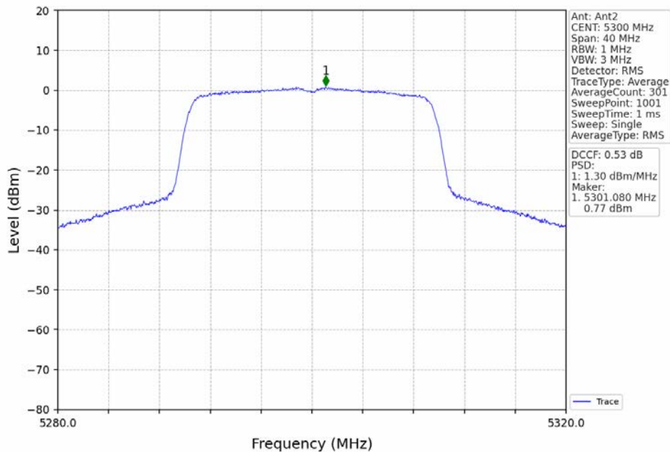
802.11ax(HEW20)_MCH_5300MHz_RU242_Left_Ant2_NTNV
