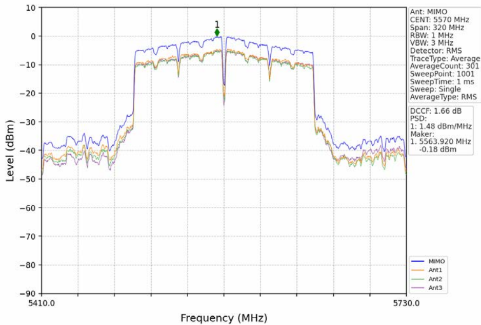
802.11ac(VHT160)_MCH_5570MHz_MIMO_NTNV
