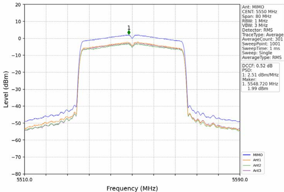
802.11ax(HEW40)_MCH_5550MHz_RU484_Left_MIMO_NTNV
