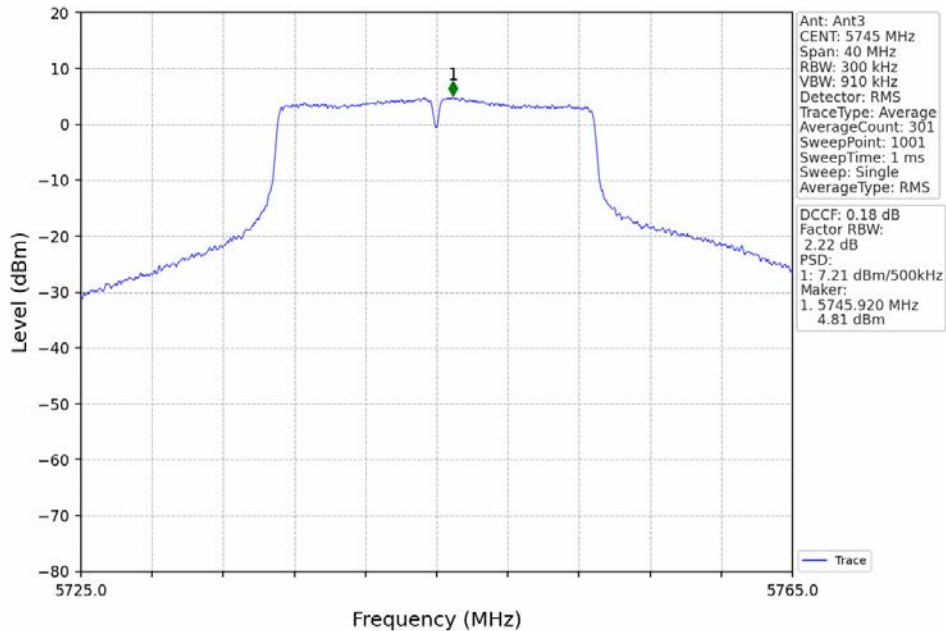
802.11n(HT20)_LCH_5745MHz_MIMO_NTNV
