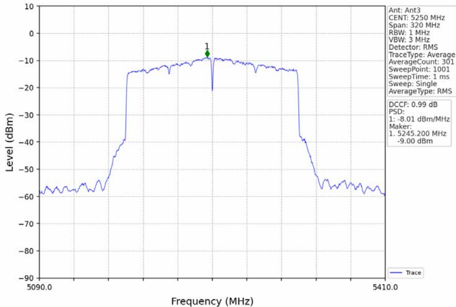
802.11ax(HEW160)_MCH_5250MHz_2xRU996_Left_MIMO_NTNV
