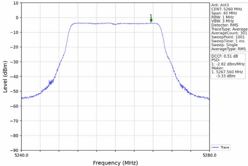
802.11ax(HEW20)_LCH_5260MHz_RU242_Left_MIMO_NTNV
