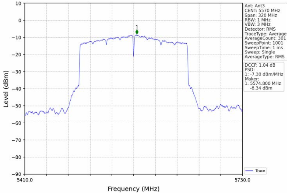
802.11ax(HEW160)_MCH_5570MHz_2xRU996_Left_MIMO_NTNV
