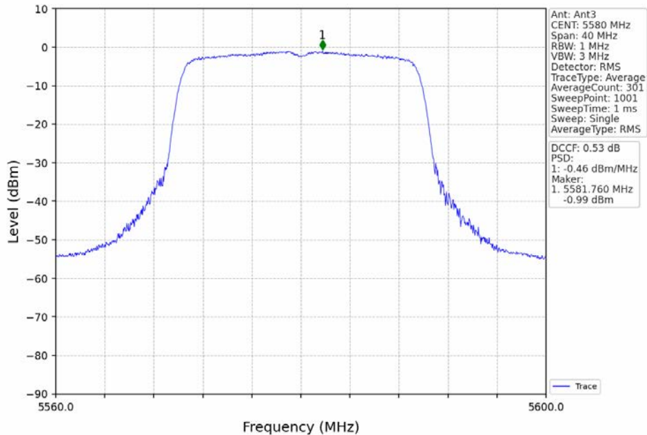
802.11ax(HEW20)_MCH_5580MHz_RU242_Left_MIMO_NTNV
