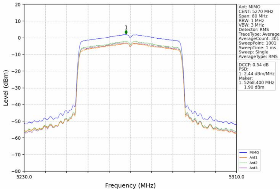
802.11ax(HEW40)_LCH_5270MHz_RU484_Left_MIMO_NTNV
