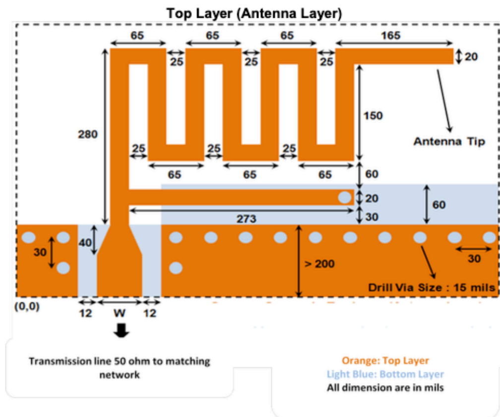
Figure 10. MIFA Layout
