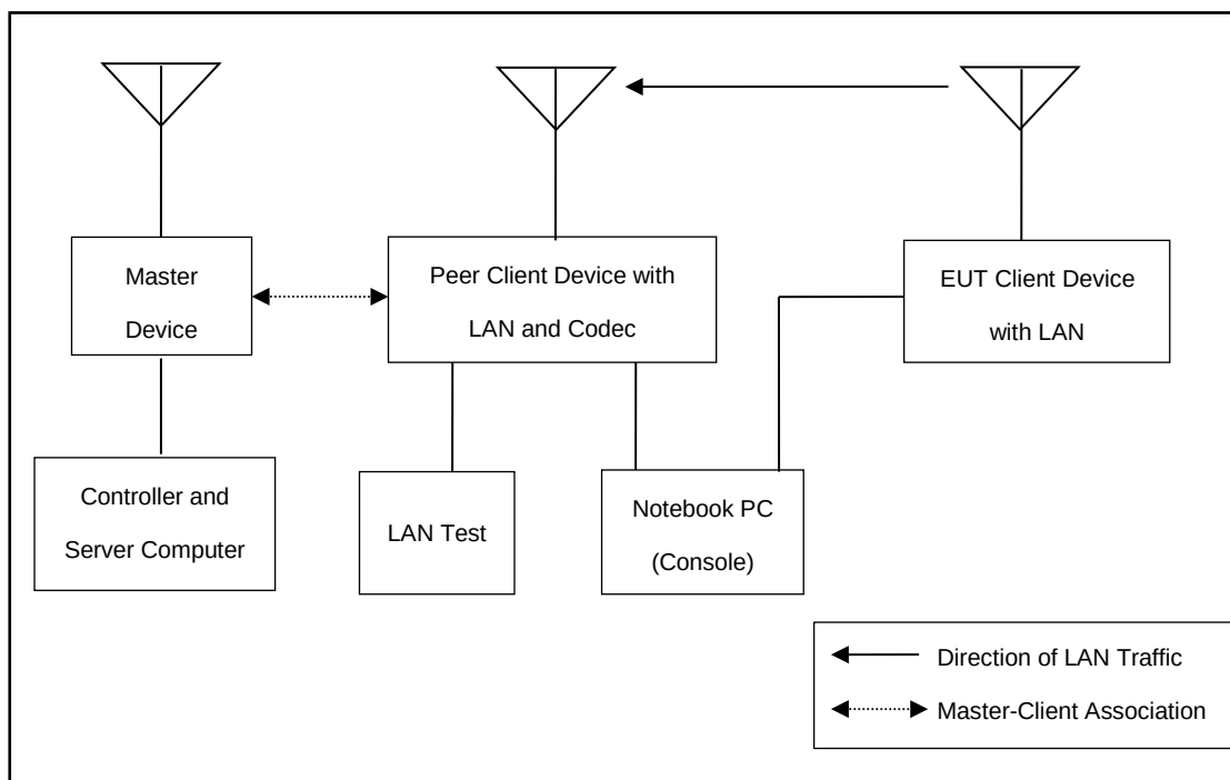
Radiated Test Setup
