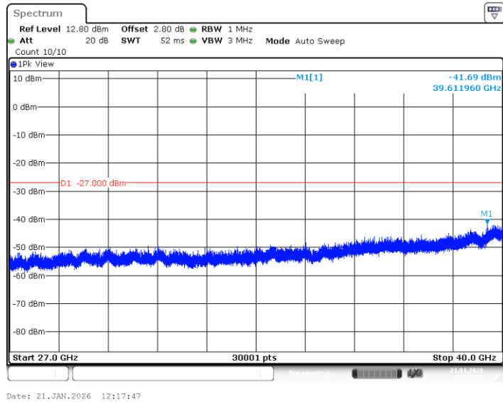
11AC40SISO_Ant1_5510_30~5460
