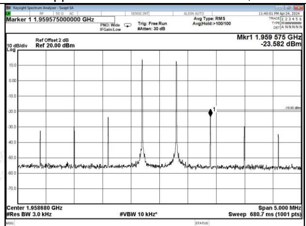
PCS Band AGC+10dB, DL
