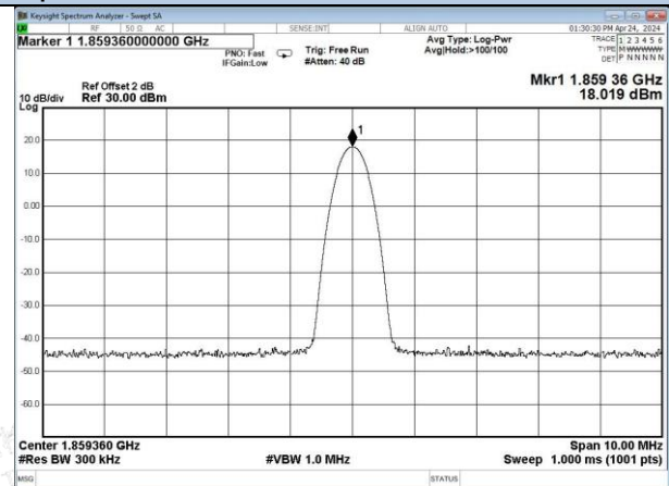
PCS Band CW, UL
