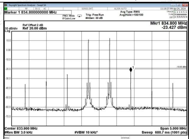
Cellular Band AGC+10dB, UL
