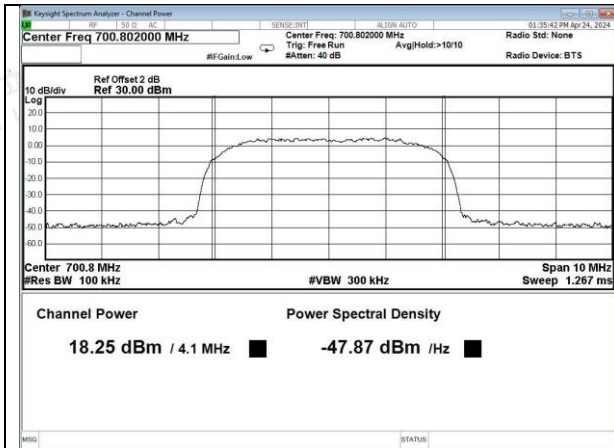
Lower 700MHz Band AWGN, UL
