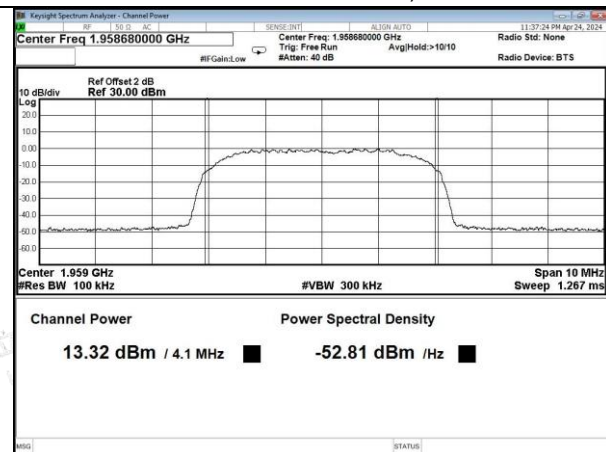
PCS Band AWGN, DL
