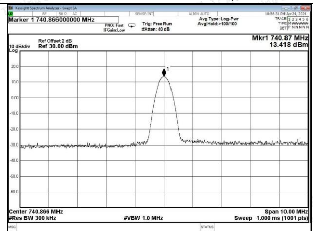
Lower 700MHz Band CW, DL
