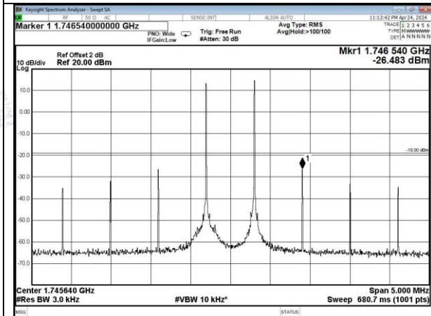
AWS Band Pre AGC, UL
