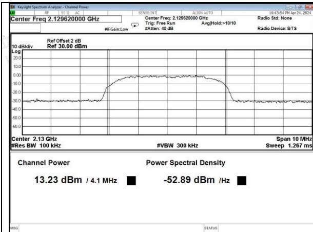
AWS Band AWGN, DL
