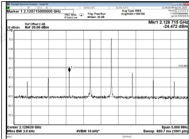
AWS Band Pre AGC, DL
