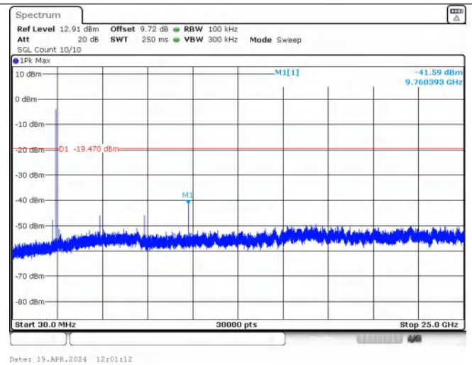
Spurious Emissions 2LE_Channel 19
