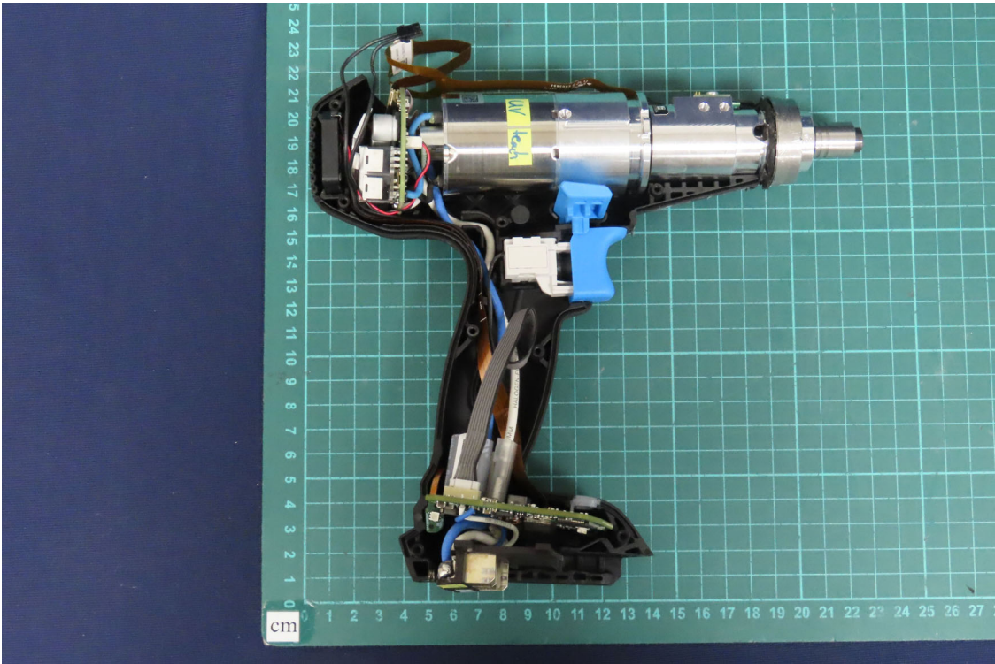
(27) EUT Photo
