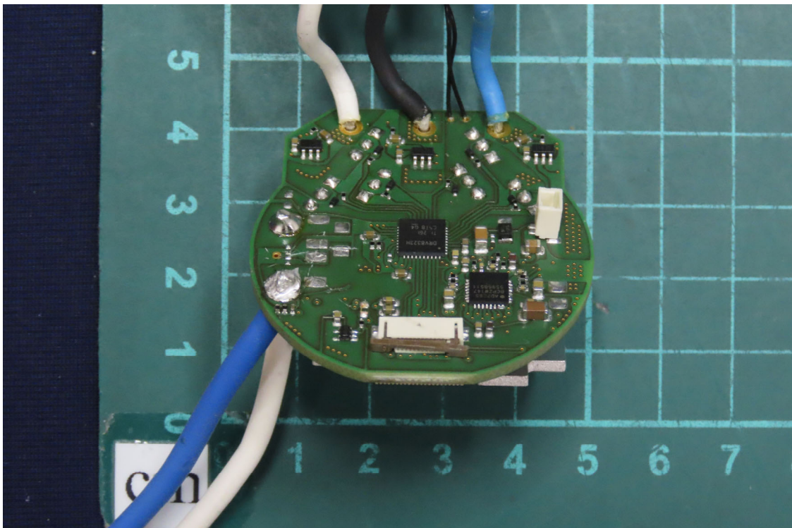
(32) EUT Photo
