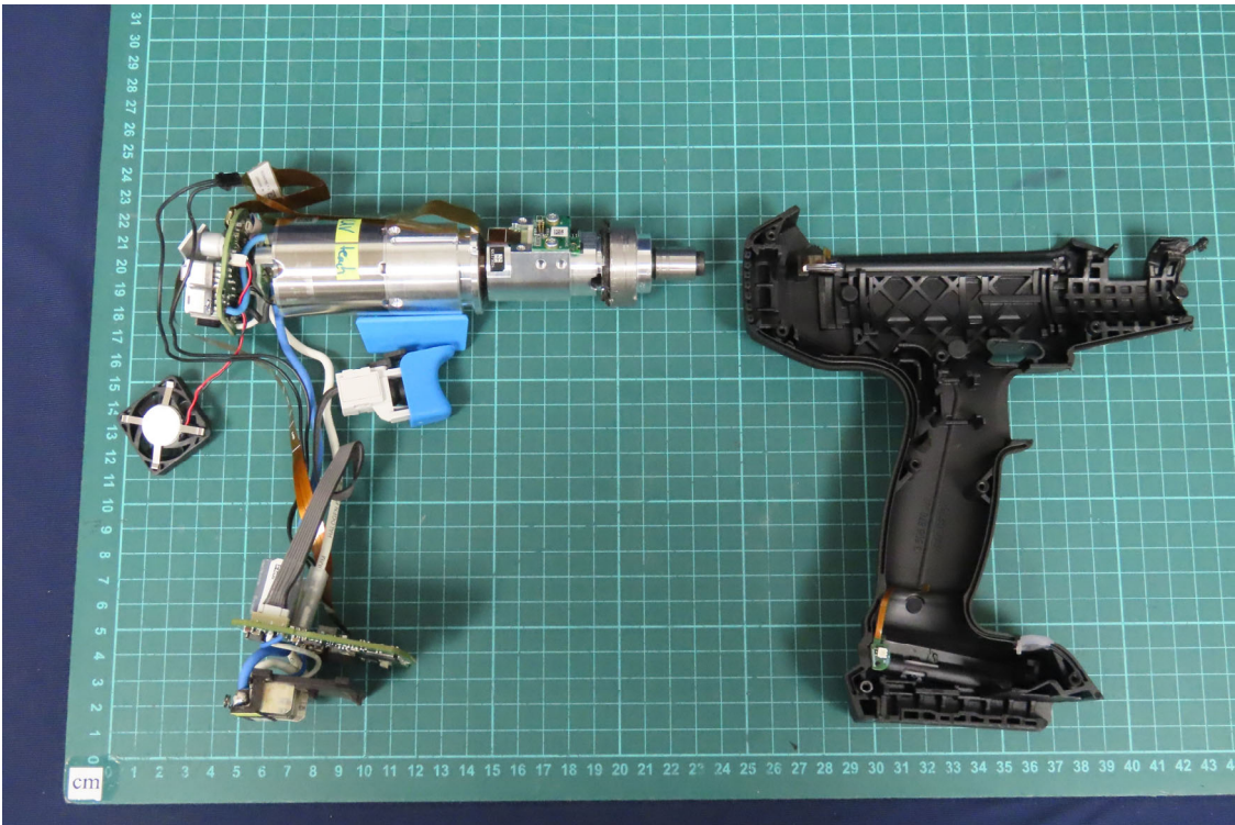
(28) EUT Photo
