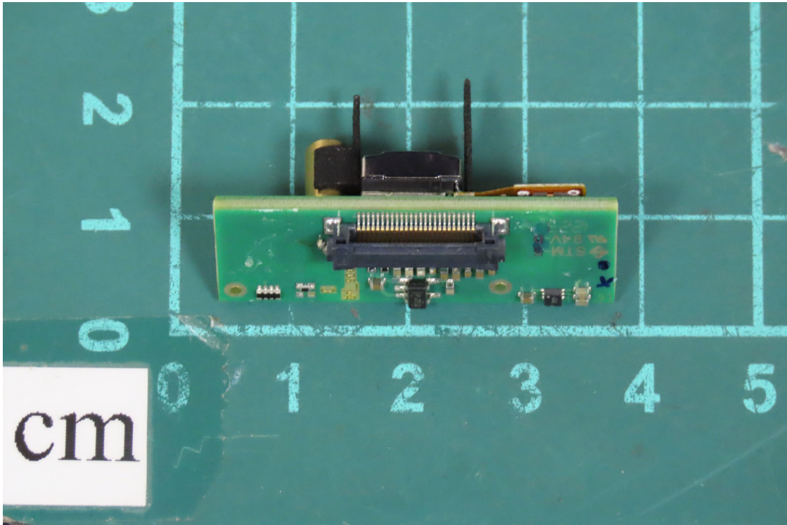
(45) EUT Photo
