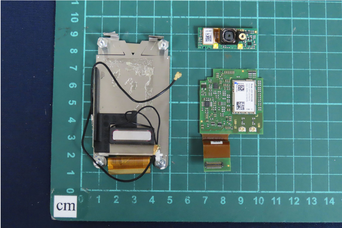
(43) EUT Photo
