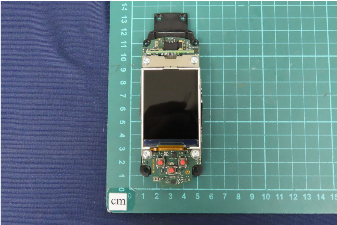
(38) EUT Photo
