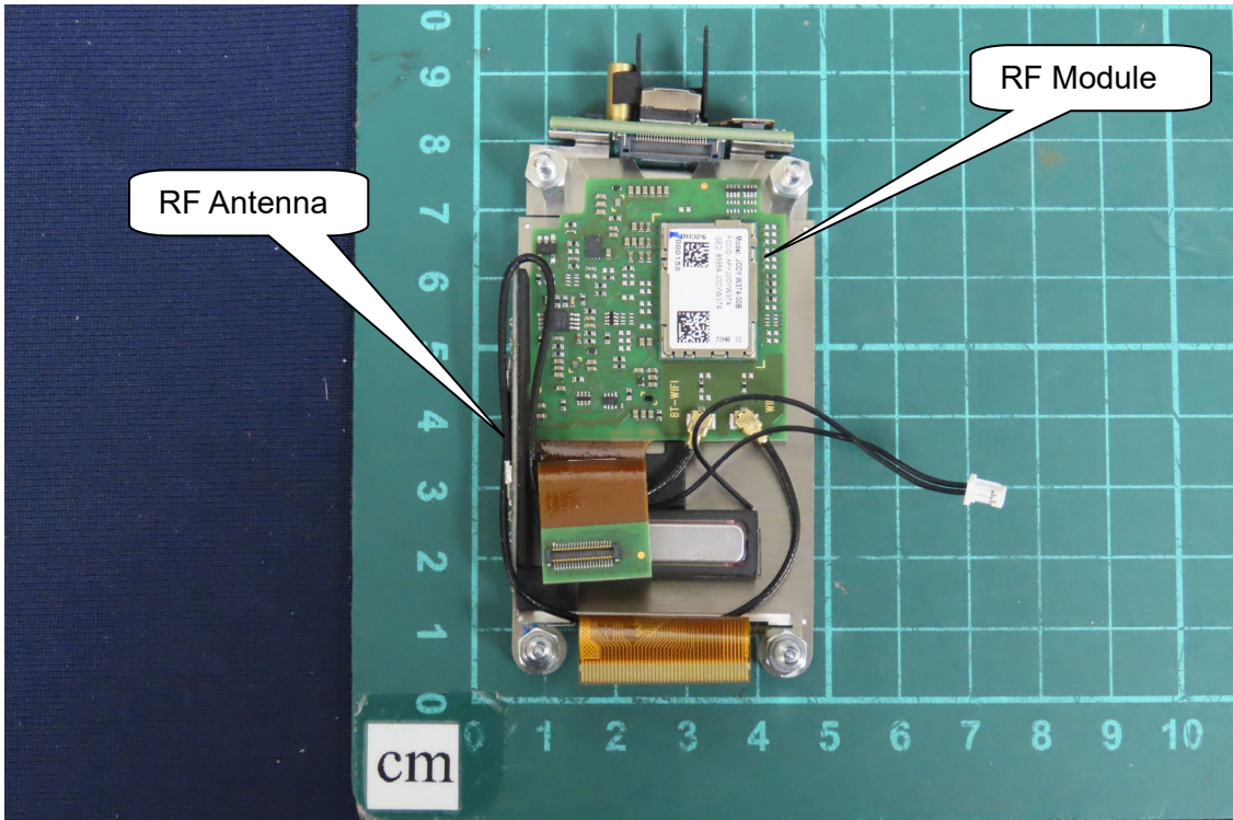
(42) EUT Photo
