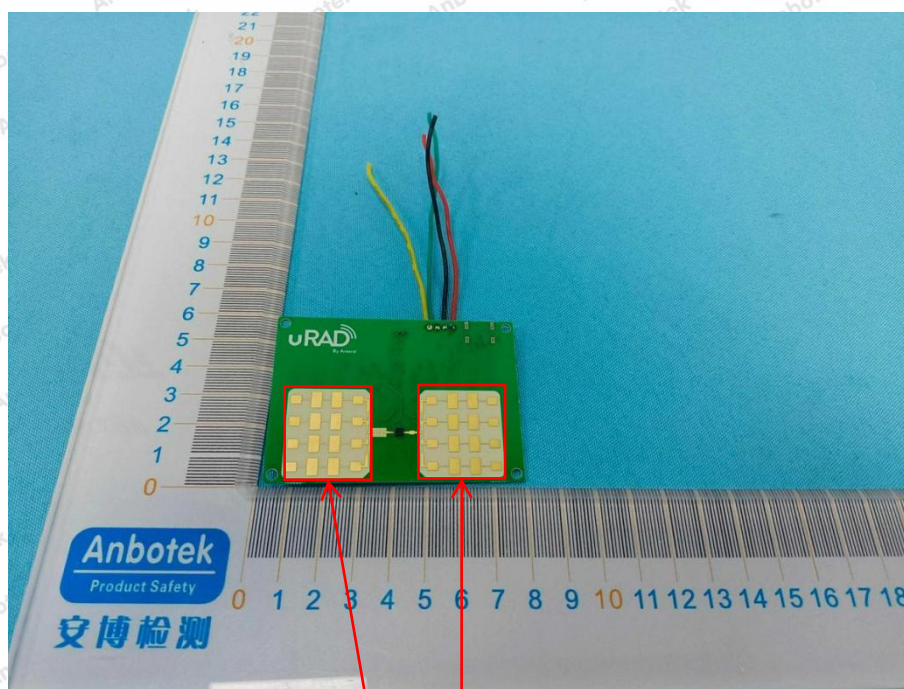
24.005GHz-24.245GHz ANT
