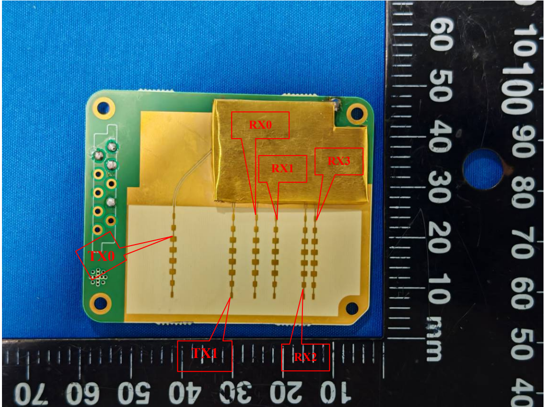
Radar Module and Antenna
