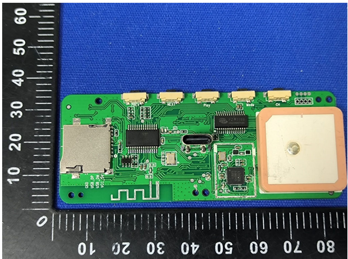
PCB Antenna
