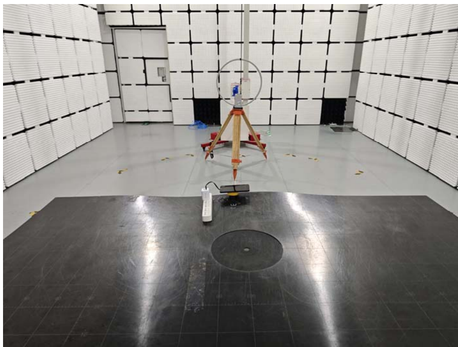
FCC ID:2BFZP-Y6 Test Photo
