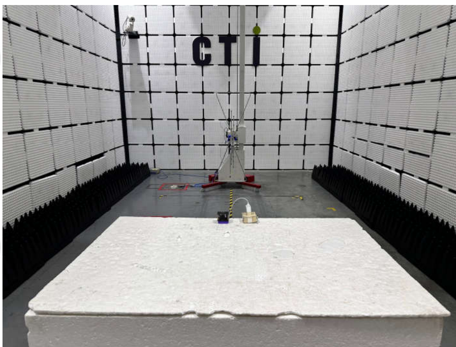
Radiated Emissions Test Setup (30MHz-1GHz)Mode b to Mode d
