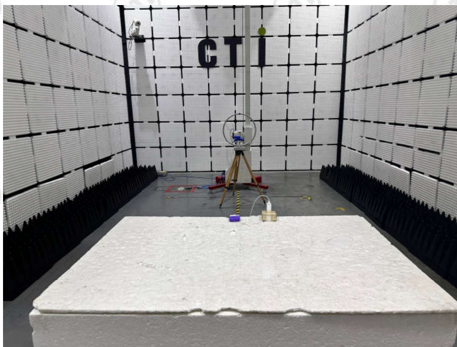
Radiated Emissions Test Setup (9kHz-30MHz) Mode a
