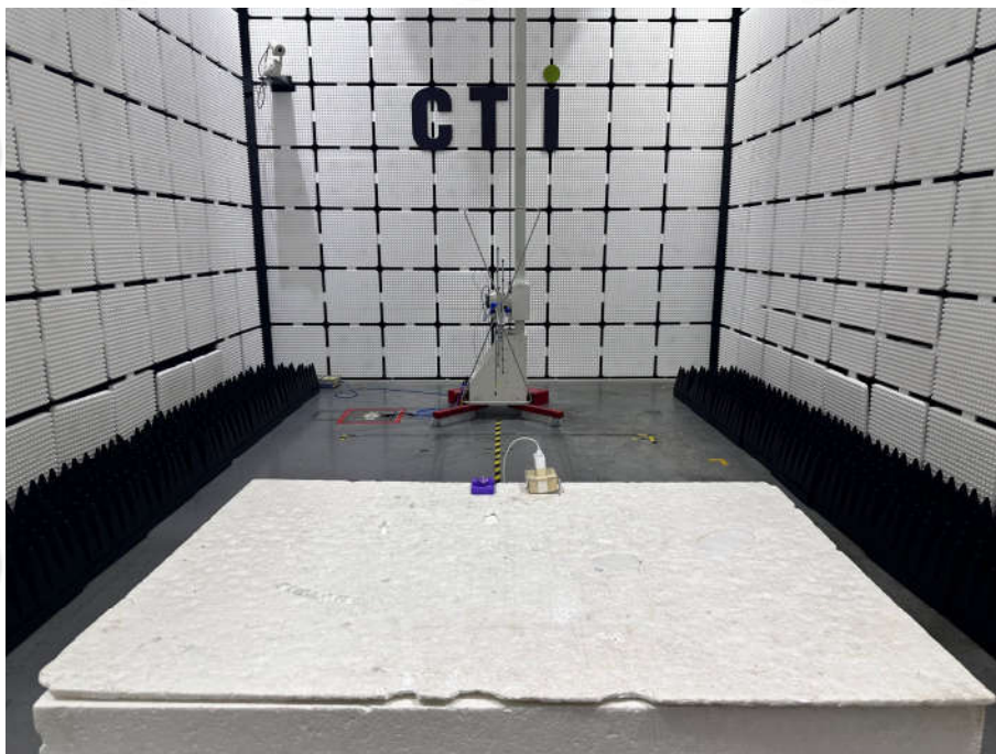
Radiated Emissions Test Setup (30MHz-1GHz)Mode a
