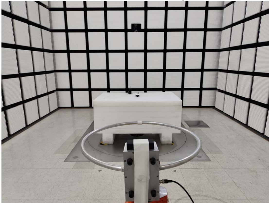
Radiated Emission 9 kHz-30 MHz Ground-parallel View
