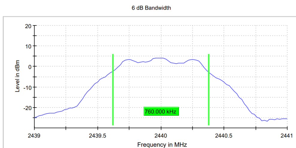
BLE_1M_Ant1_2440
