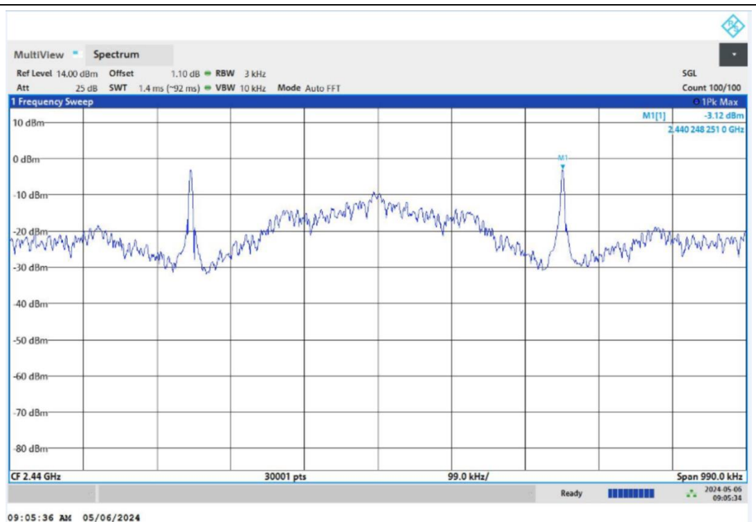
BLE_S8_Ant1_2440
