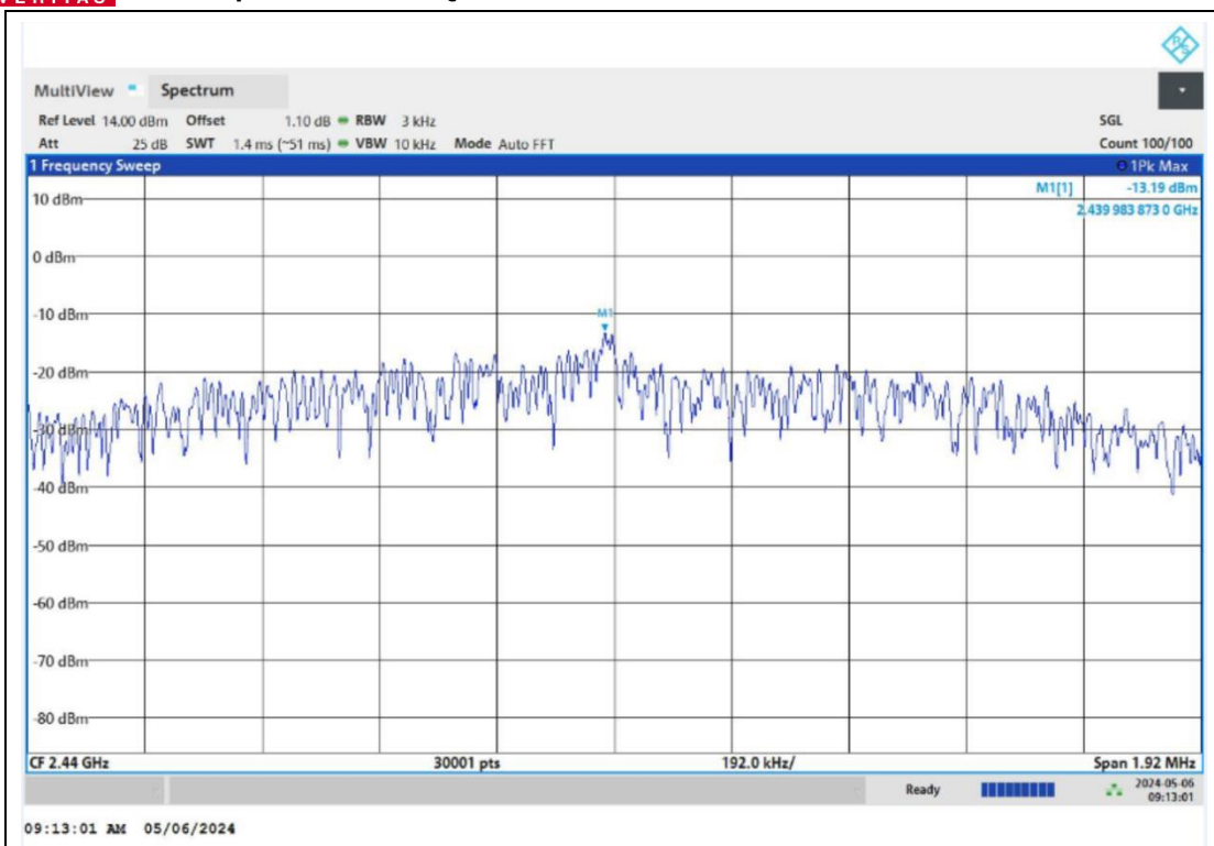
BLE_2M_Ant1_2440
