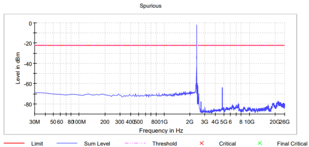
BLE_1M_Ant1_2480_30~26000
