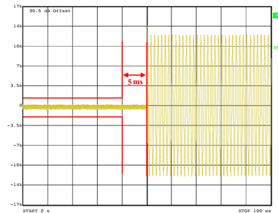
Transmitter Frequency Behavior @ 25 KHz Channel Separation-----On – Off
