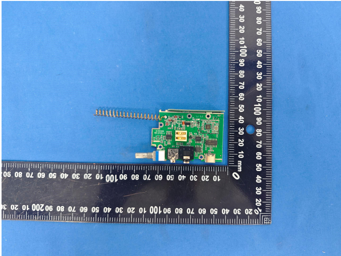
Spring Antenna
