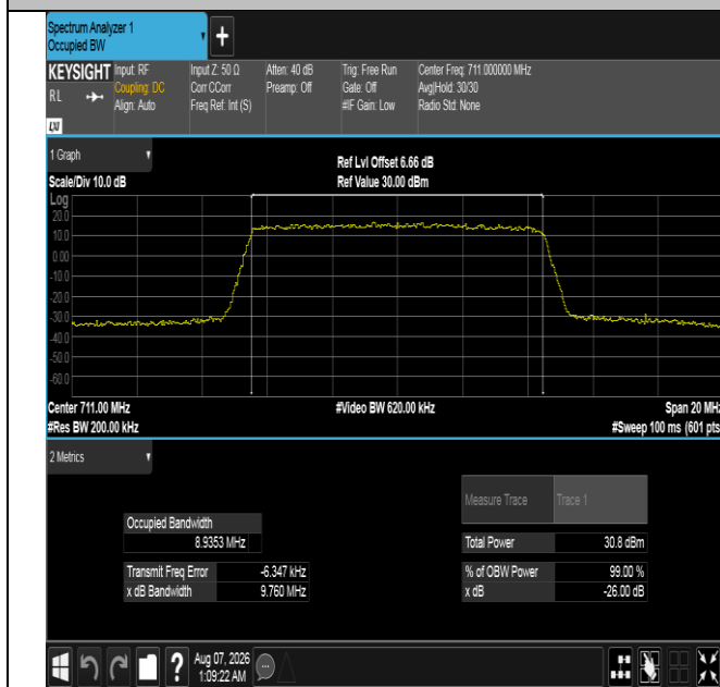
Band12-10MHz-QPSK-23130-50RB#0-PASS
