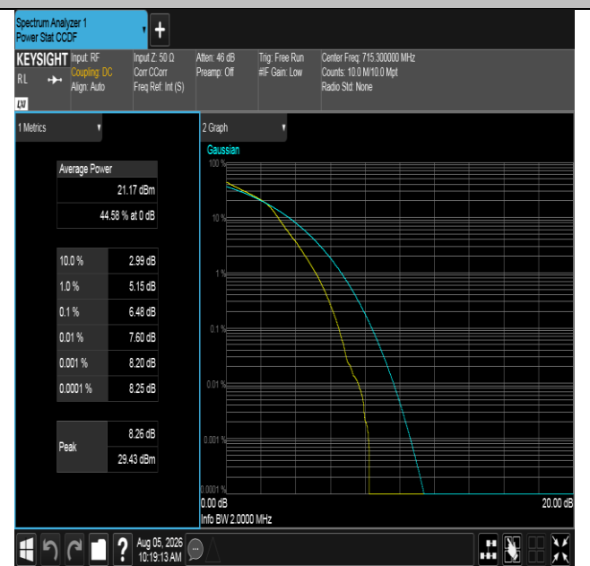
Band12-1.4MHz-16QAM-23173-6RB#0-PASS
