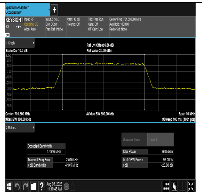
Band12-5MHz-16QAM-23035-25RB#0-PASS
