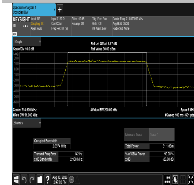
Band12-3MHz-QPSK-23165-15RB#0-PASS
