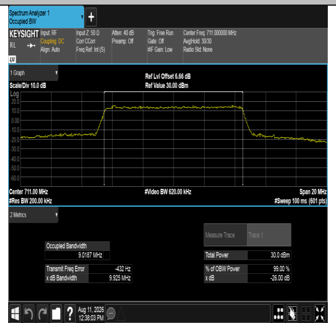
Band12-10MHz-16QAM-23130-50RB#0-PASS
