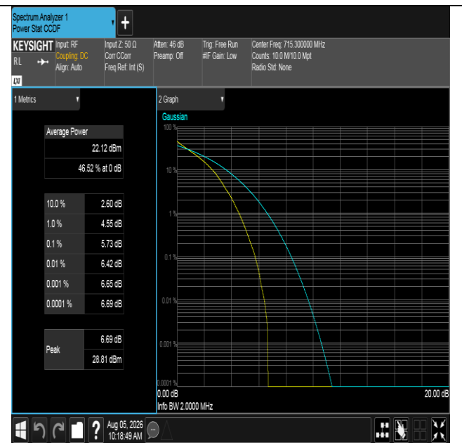
Band12-1.4MHz-QPSK-23173-6RB#0-PASS
