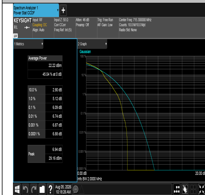
Band12-1.4MHz-16QAM-23173-1RB#0-PASS
