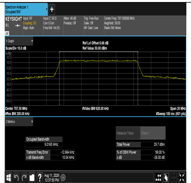
Band12-10MHz-16QAM-23095-50RB#0-PASS
