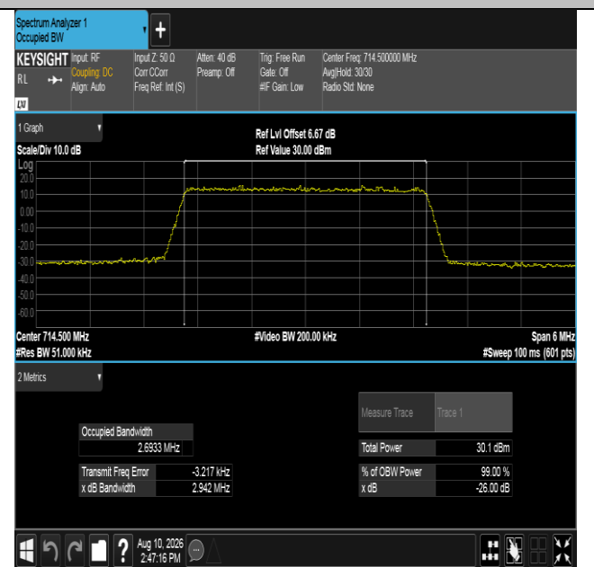
Band12-3MHz-16QAM-23165-15RB#0-PASS
