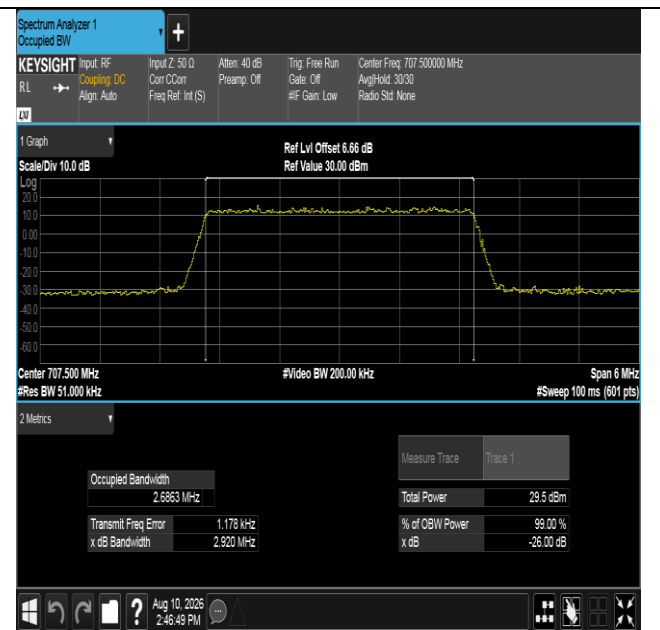
Band12-3MHz-16QAM-23095-15RB#0-PASS
