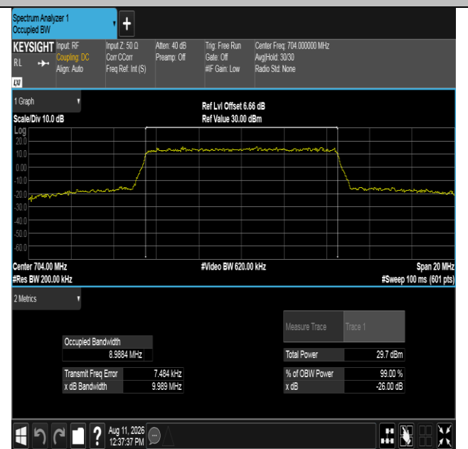
Band12-10MHz-16QAM-23060-50RB#0-PASS
