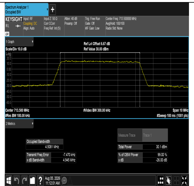
Band12-5MHz-16QAM-23155-25RB#0-PASS
