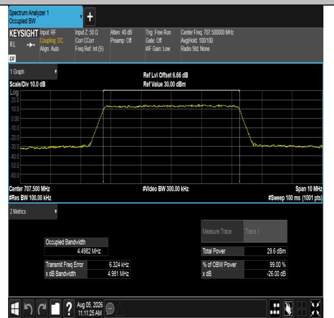
Band12-5MHz-16QAM-23095-25RB#0-PASS
