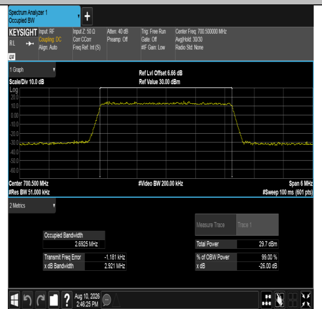
Band12-3MHz-16QAM-23025-15RB#0-PASS
