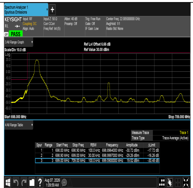
Band12-10MHz-16QAM-23060-1RB#0-PASS
