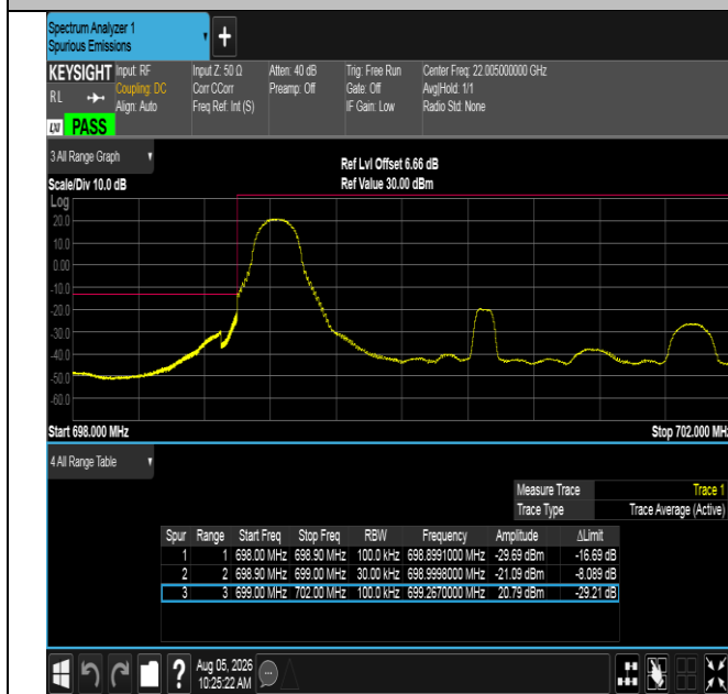
Band12-3MHz-QPSK-23025-1RB#0-PASS
