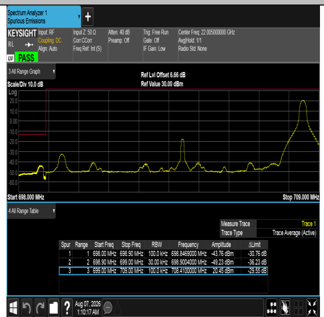
Band12-10MHz-QPSK-23060-1RB#49-PASS
