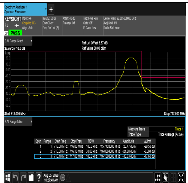
Band12-3MHz-QPSK-23165-1RB#14-PASS
