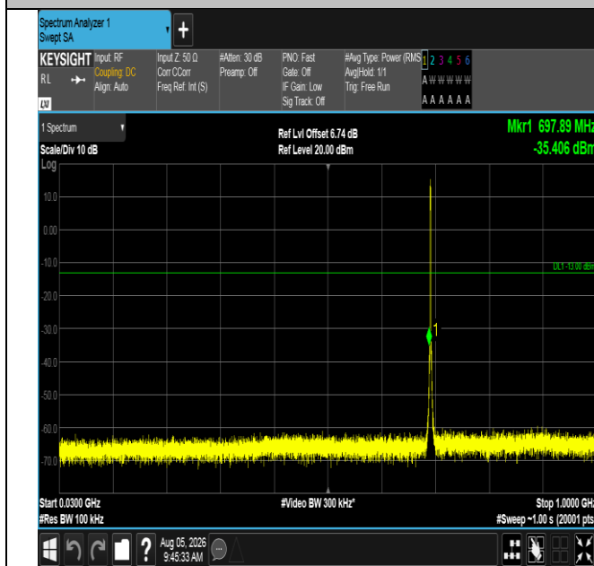
Band12-1.4MHz-QPSK-23017-6RB#0-30~1000-PASS
