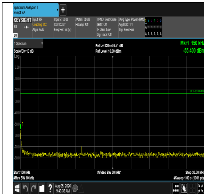
Band12-1.4MHz-QPSK-23017-1RB#5-0.15~30-PASS
