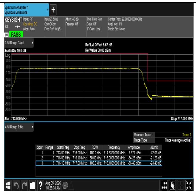
Band12-3MHz-16QAM-23165-15RB#0-PASS
