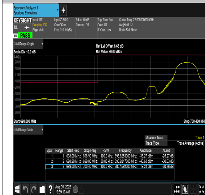
Band12-1.4MHz-16QAM-23017-1RB#5-PASS
