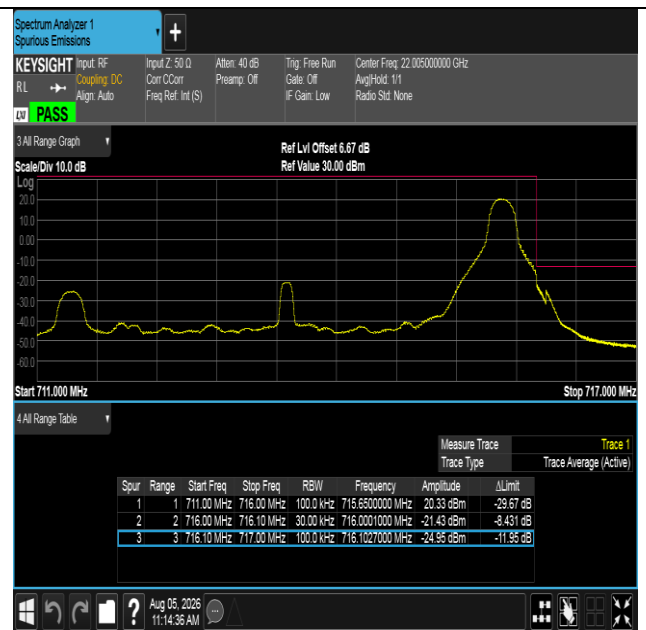
Band12-5MHz-QPSK-23155-1RB#24-PASS
