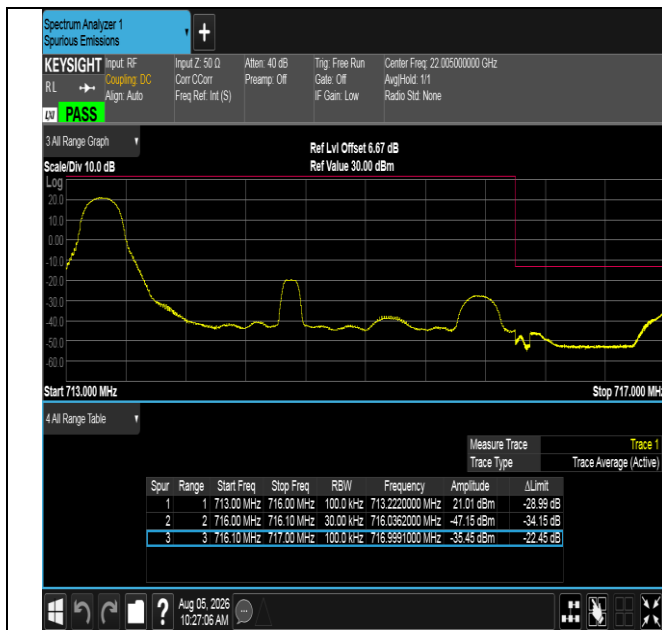
Band12-3MHz-QPSK-23165-1RB#0-PASS
