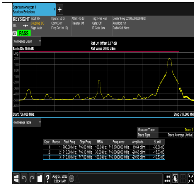
Band12-10MHz-16QAM-23130-1RB#49-PASS
