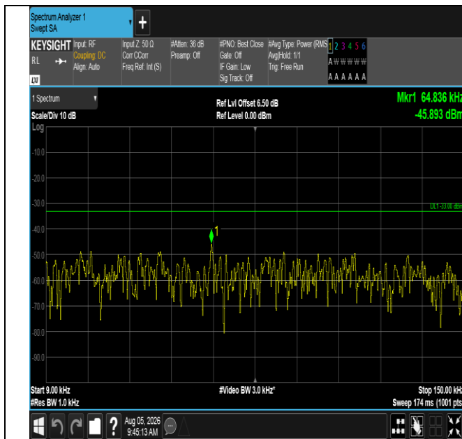
Band12-1.4MHz-QPSK-23017-6RB#0-0.009~0.15-PASS
