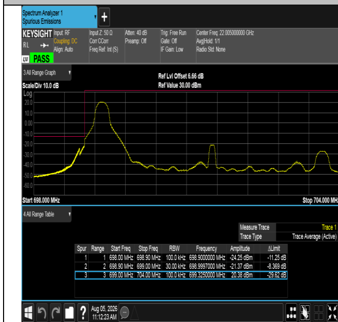
Band12-5MHz-QPSK-23035-1RB#0-PASS
