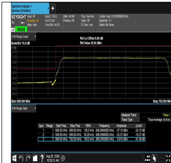
Band12-3MHz-QPSK-23025-15RB#0-PASS
