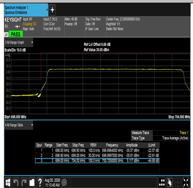
Band12-5MHz-16QAM-23035-25RB#0-PASS
