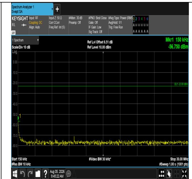
Band12-1.4MHz-QPSK-23017-6RB#0-0.15~30-PASS
