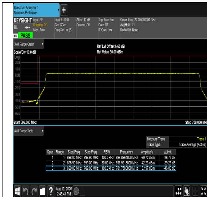
Band12-10MHz-QPSK-23060-50RB#0-PASS
