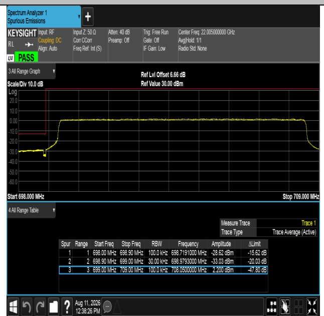
Band12-10MHz-16QAM-23060-50RB#0-PASS
