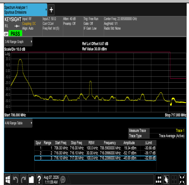
Band12-10MHz-16QAM-23130-1RB#0-PASS
