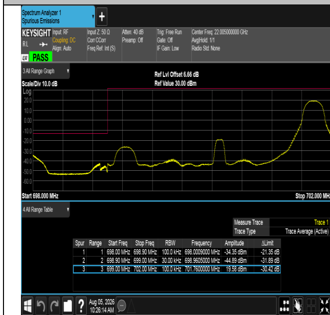
Band12-3MHz-16QAM-23025-1RB#14-PASS
