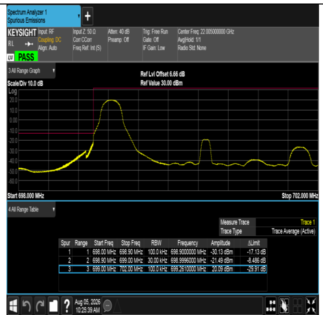
Band12-3MHz-16QAM-23025-1RB#0-PASS
