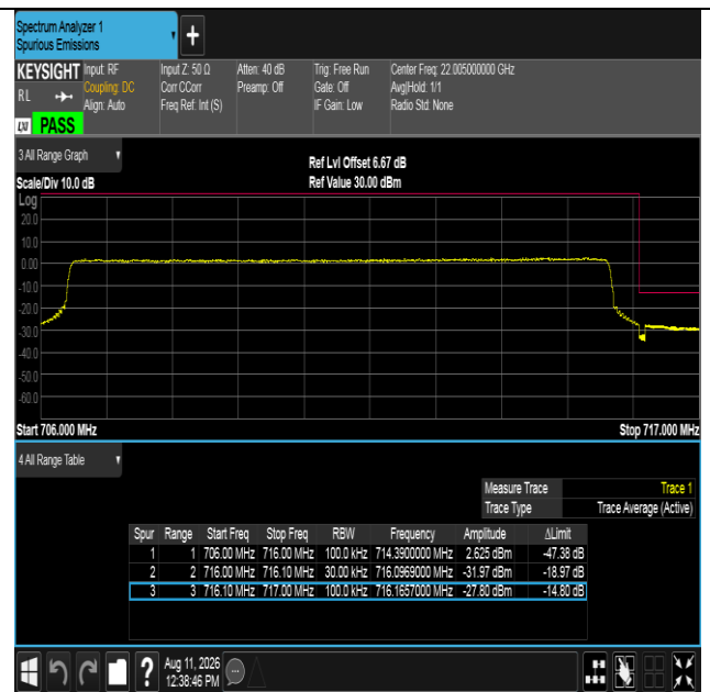
Band12-10MHz-16QAM-23130-50RB#0-PASS
