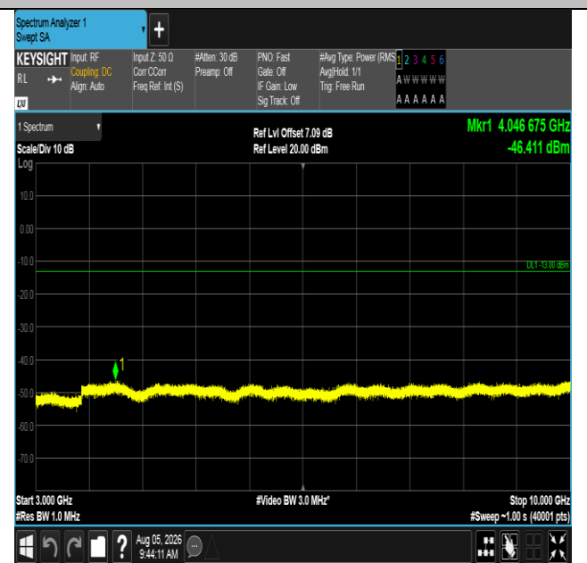
Band12-1.4MHz-QPSK-23017-1RB#5-3000~10000-PASS
