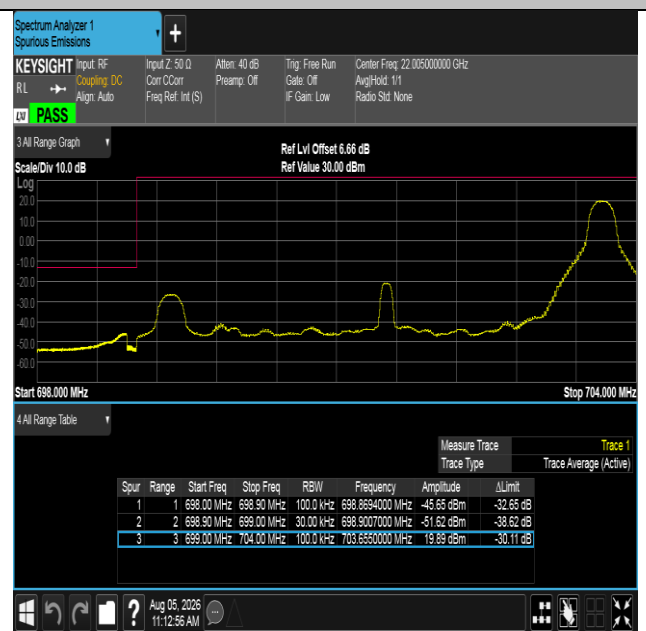
Band12-5MHz-QPSK-23035-1RB#24-PASS
