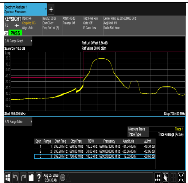
Band12-1.4MHz-16QAM-23017-1RB#0-PASS
