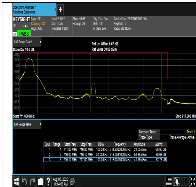
Band12-5MHz-QPSK-23155-1RB#0-PASS
