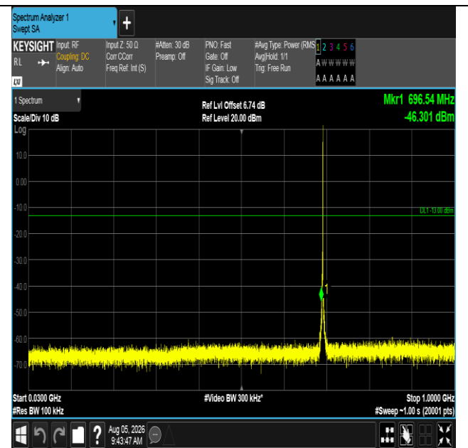
Band12-1.4MHz-QPSK-23017-1RB#5-30~1000-PASS
