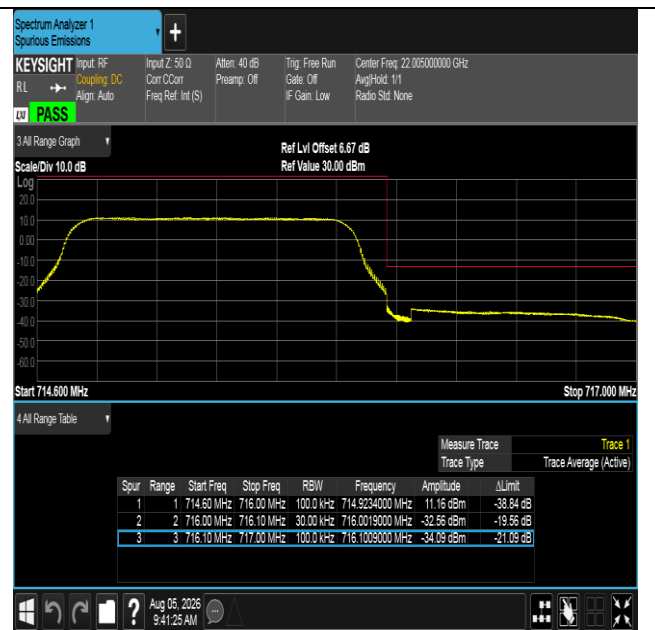
Band12-1.4MHz-16QAM-23173-6RB#0-PASS
