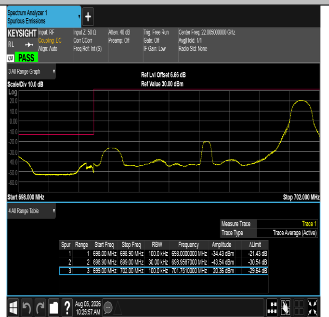
Band12-3MHz-QPSK-23025-1RB#14-PASS
