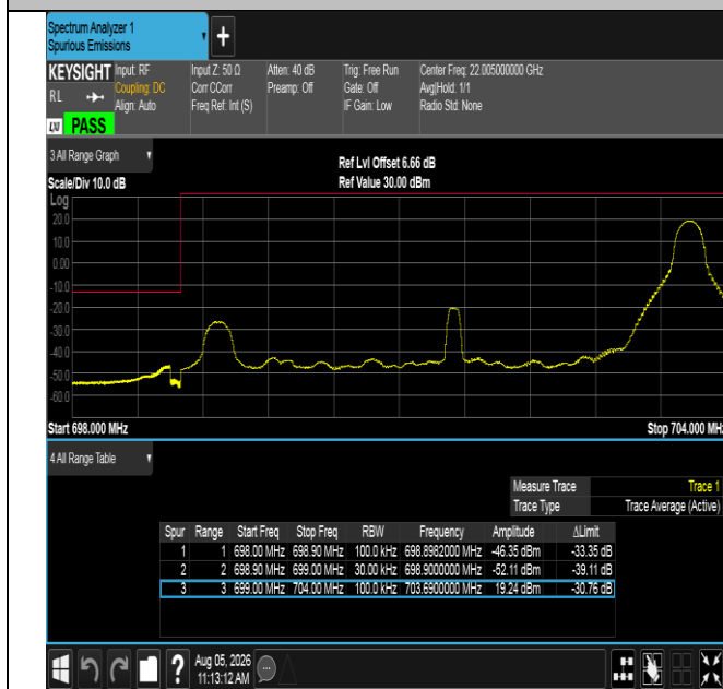
Band12-5MHz-16QAM-23035-1RB#24-PASS
