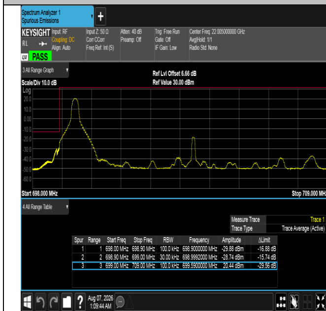
Band12-10MHz-QPSK-23060-1RB#0-PASS
