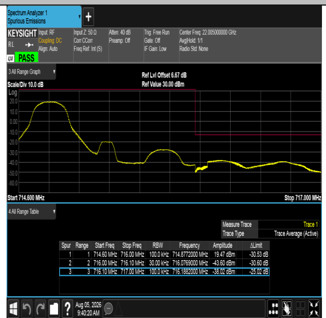
Band12-1.4MHz-16QAM-23173-1RB#0-PASS
