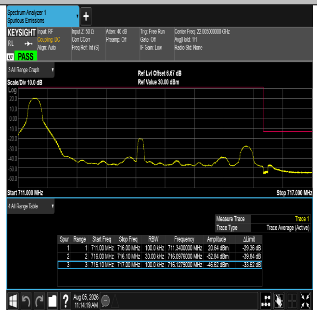
Band12-5MHz-16QAM-23155-1RB#0-PASS
