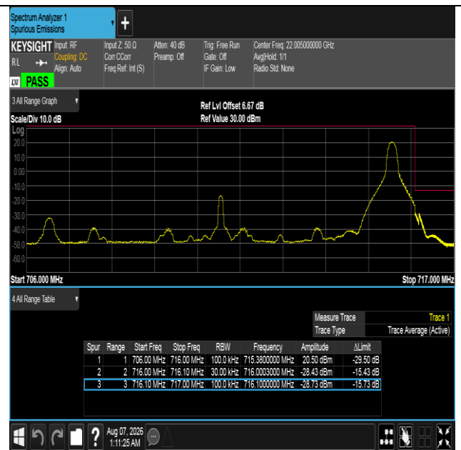
Band12-10MHz-QPSK-23130-1RB#49-PASS
