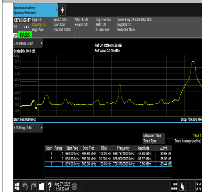
Band12-10MHz-16QAM-23060-1RB#49-PASS
