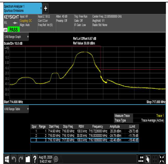
Band12-1.4MHz-QPSK-23173-1RB#5-PASS
