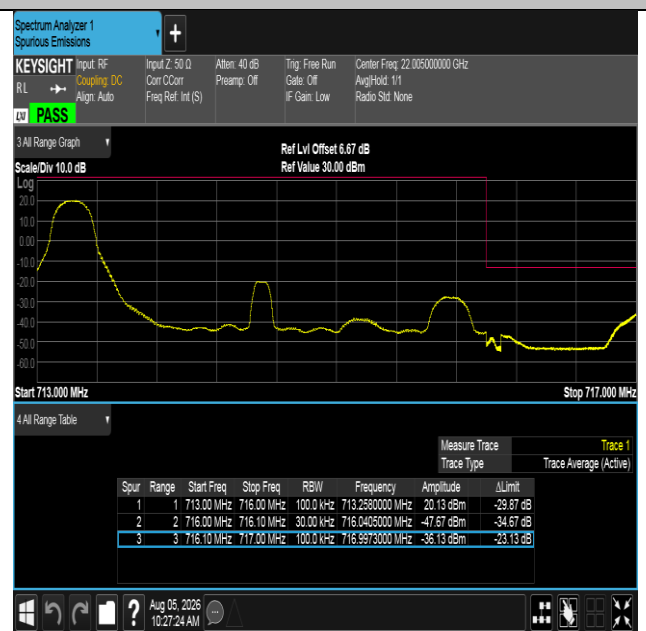
Band12-3MHz-16QAM-23165-1RB#0-PASS
