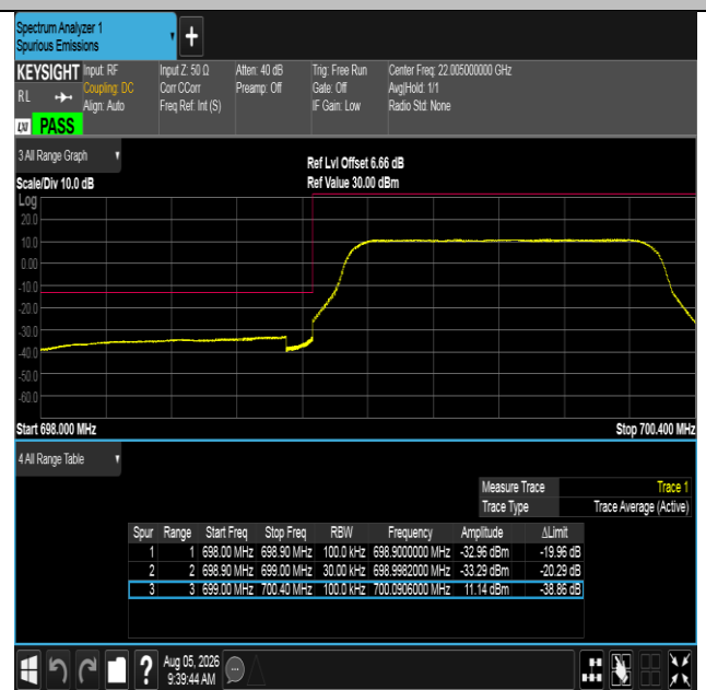
Band12-1.4MHz-16QAM-23017-6RB#0-PASS
