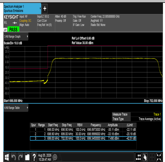
Band12-3MHz-16QAM-23025-15RB#0-PASS
