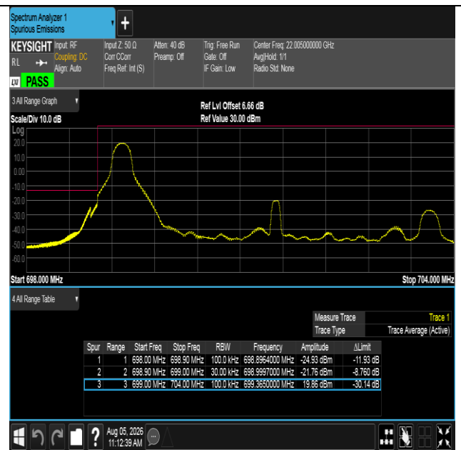
Band12-5MHz-16QAM-23035-1RB#0-PASS
