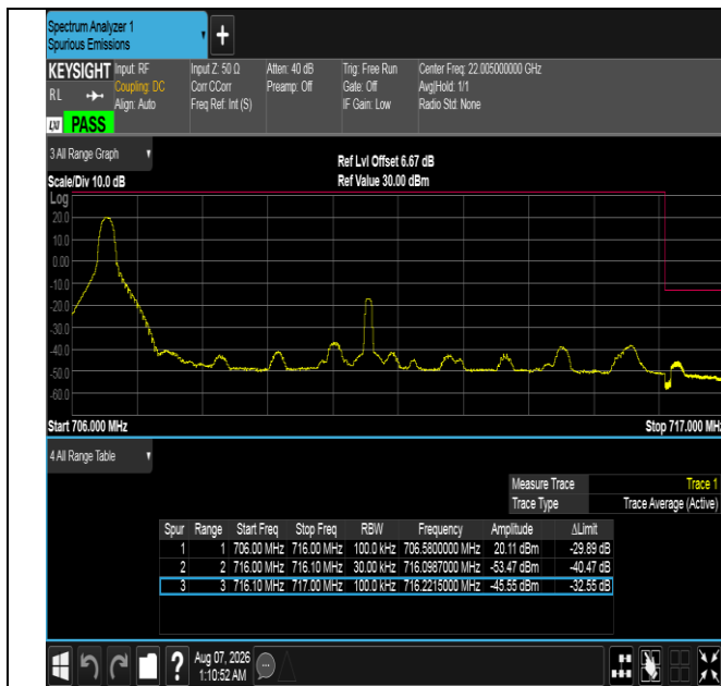
Band12-10MHz-QPSK-23130-1RB#0-PASS
