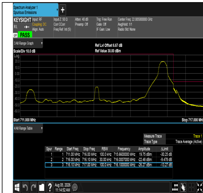
Band12-5MHz-16QAM-23155-1RB#24-PASS
