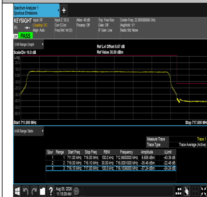
Band12-5MHz-QPSK-23155-25RB#0-PASS
