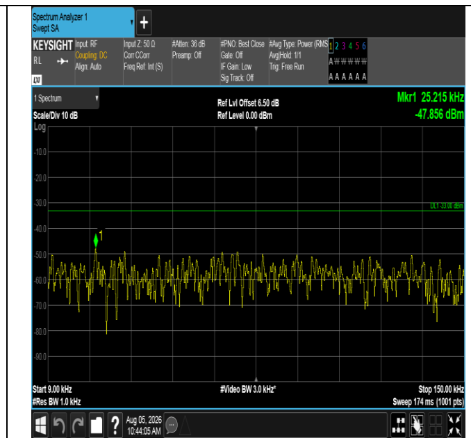
Band12-3MHz-16QAM-23165-15RB#0-0.009~0.15-PASS
