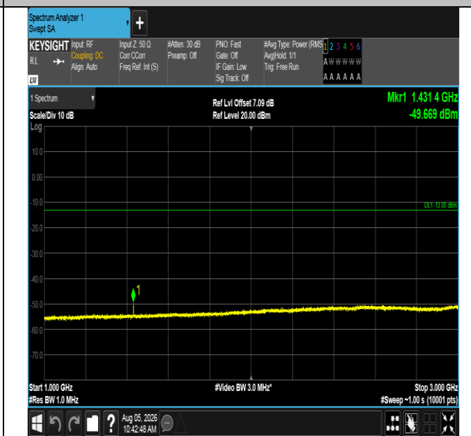
Band12-3MHz-16QAM-23165-1RB#14-1000~3000-PASS
