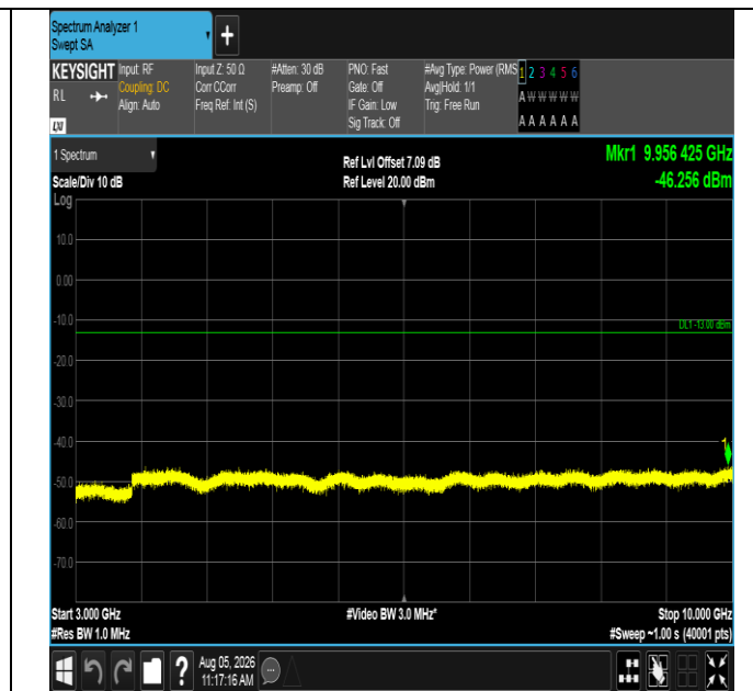
Band12-5MHz-16QAM-23035-1RB#0-3000~10000-PASS
