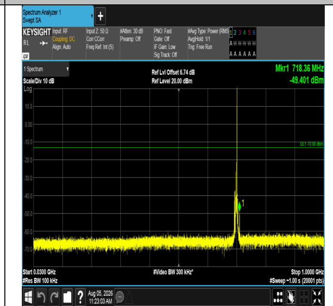
Band12-5MHz-QPSK-23095-1RB#24-30~1000-PASS
