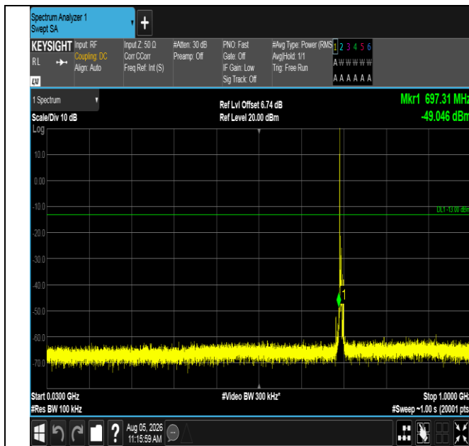
Band12-5MHz-QPSK-23035-1RB#0-30~1000-PASS
