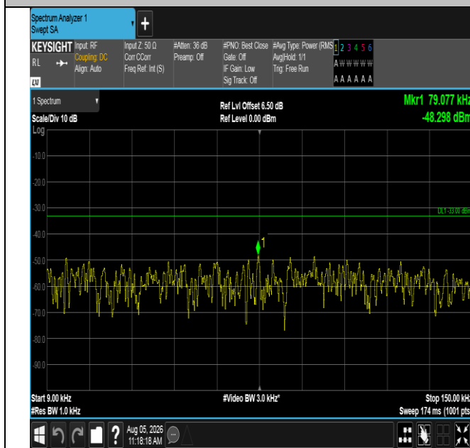
Band12-5MHz-16QAM-23035-1RB#24-0.009~0.15-PASS
