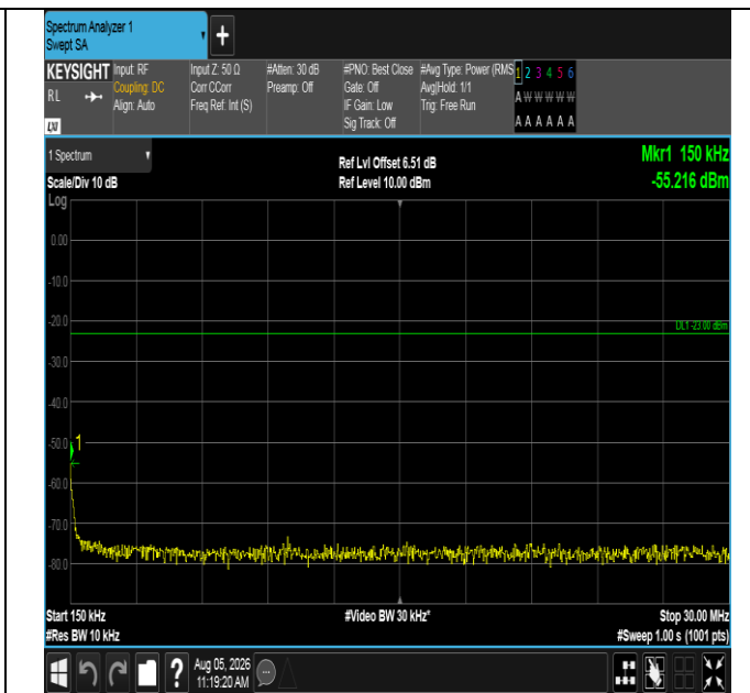
Band12-5MHz-QPSK-23035-25RB#0-0.15~30-PASS
