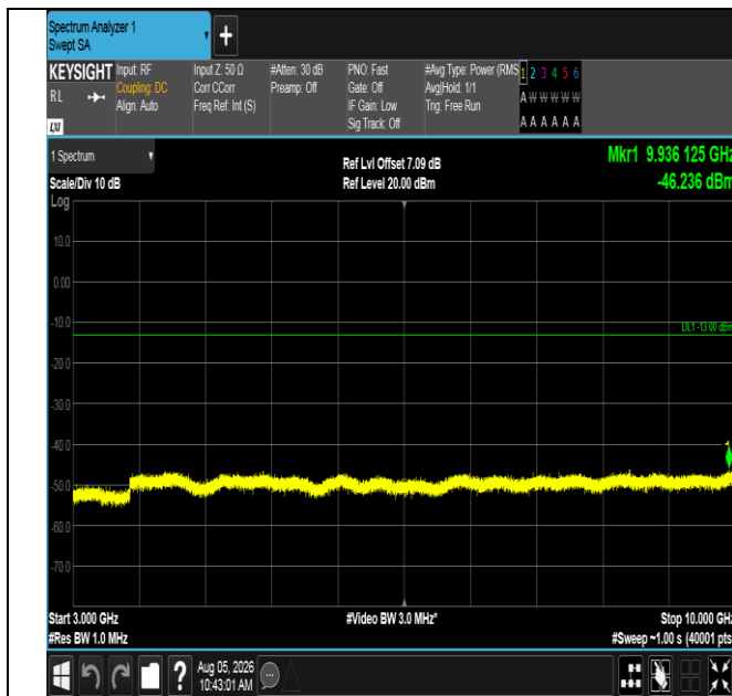
Band12-3MHz-16QAM-23165-1RB#14-3000~10000-PASS
