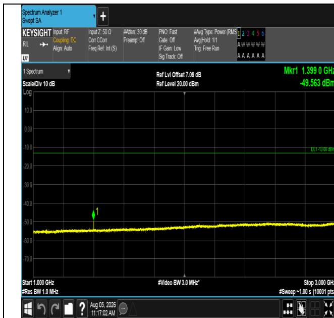
Band12-5MHz-16QAM-23035-1RB#0-1000~3000-PASS
