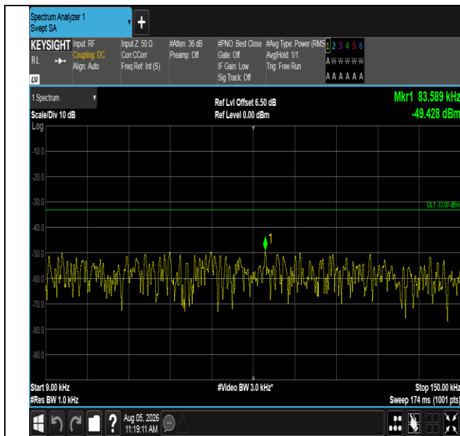
Band12-5MHz-QPSK-23035-25RB#0-0.009~0.15-PASS
