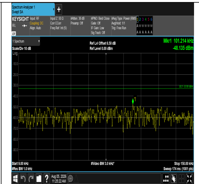
Band12-5MHz-16QAM-23095-25RB#0-0.009~0.15-PASS
