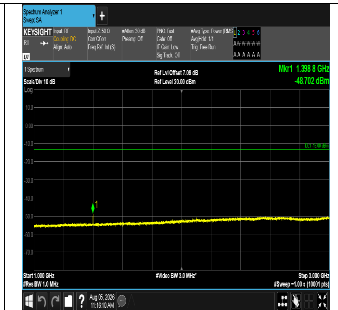
Band12-5MHz-QPSK-23035-1RB#0-1000~3000-PASS
