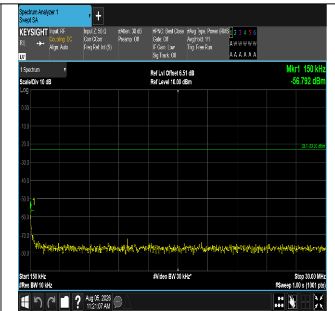
Band12-5MHz-QPSK-23095-1RB#0-0.15~30-PASS
