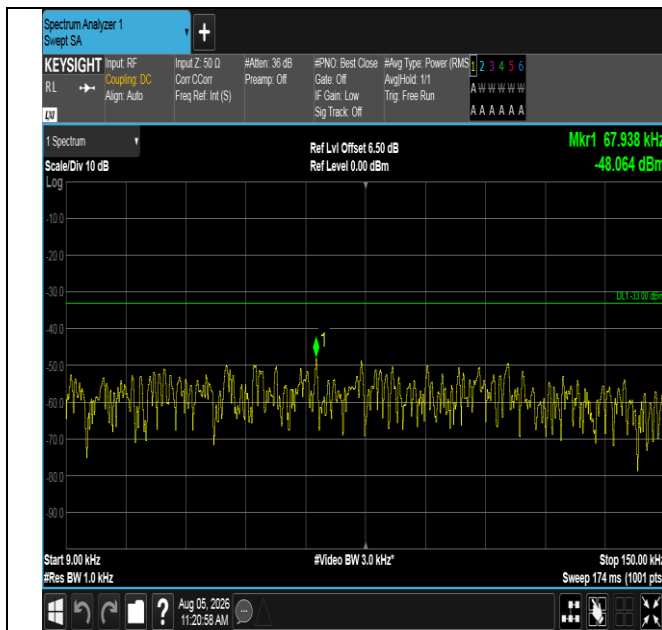
Band12-5MHz-QPSK-23095-1RB#0-0.009~0.15-PASS
