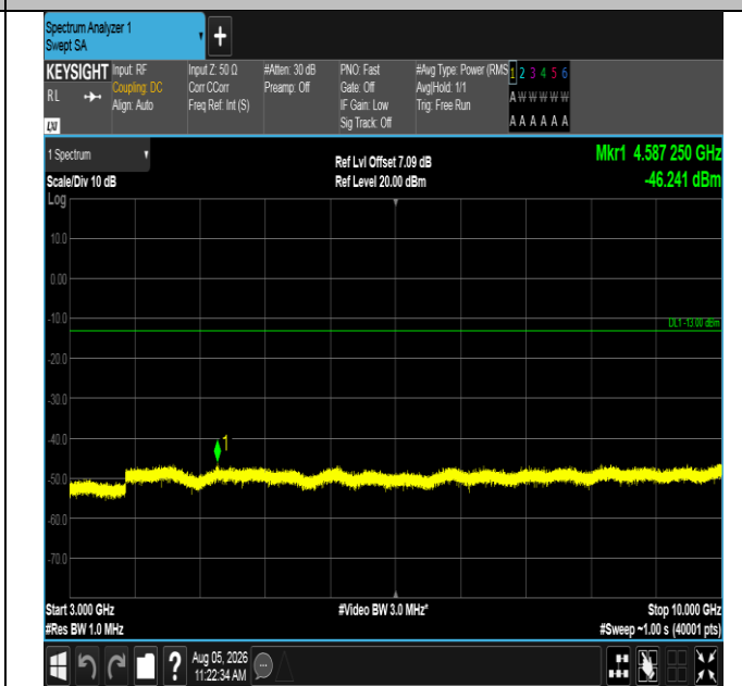
Band12-5MHz-16QAM-23095-1RB#0-3000~10000-PASS
