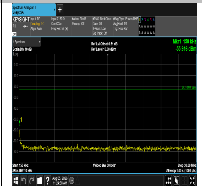
Band12-5MHz-QPSK-23095-25RB#0-0.15~30-PASS
