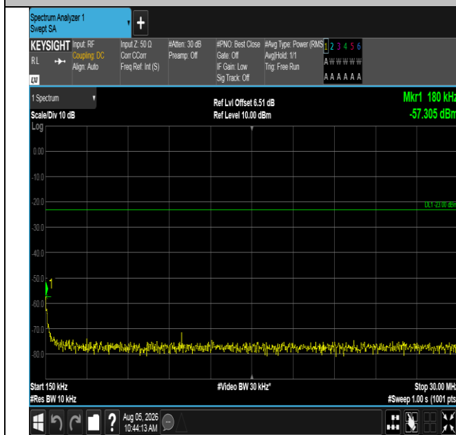
Band12-3MHz-16QAM-23165-15RB#0-0.15~30-PASS
