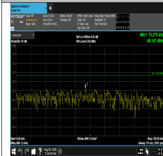
Band12-5MHz-QPSK-23095-25RB#0-0.009~0.15-PASS
