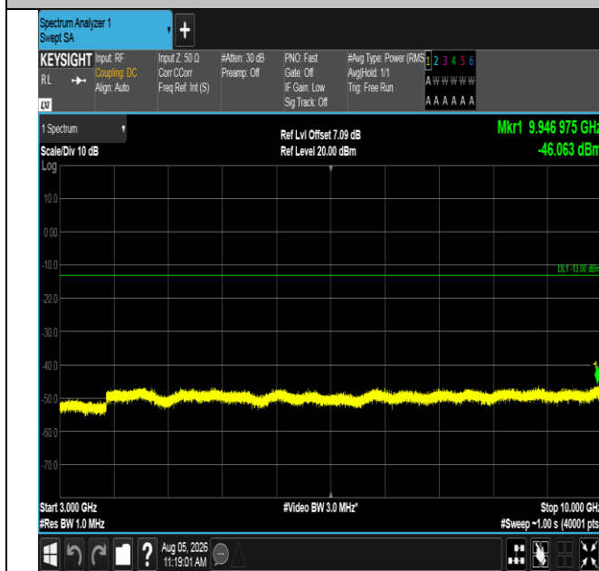
Band12-5MHz-16QAM-23035-1RB#24-3000~10000-PASS
