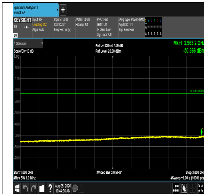
Band12-3MHz-16QAM-23165-15RB#0-1000~3000-PASS
