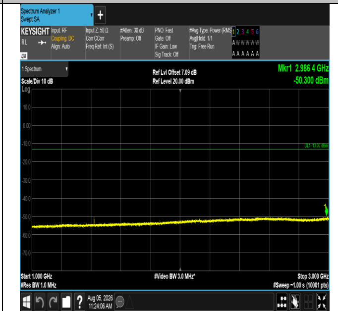
Band12-5MHz-16QAM-23095-1RB#24-1000~3000-PASS
