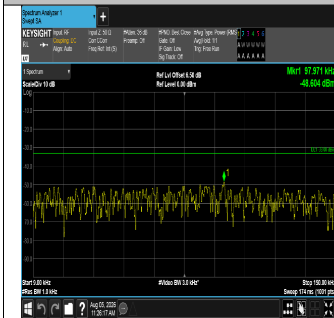
Band12-5MHz-QPSK-23155-1RB#0-0.009~0.15-PASS
