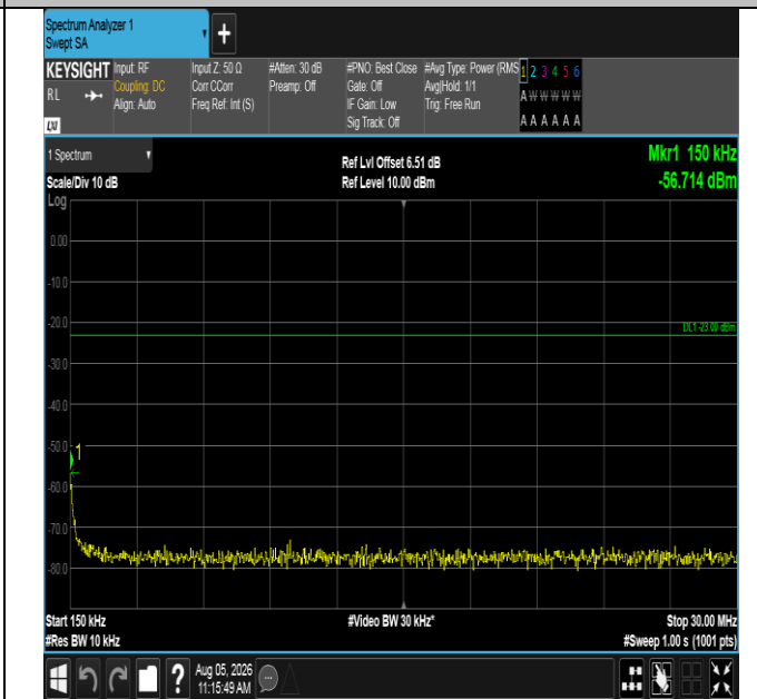
Band12-5MHz-QPSK-23035-1RB#0-0.15~30-PASS
