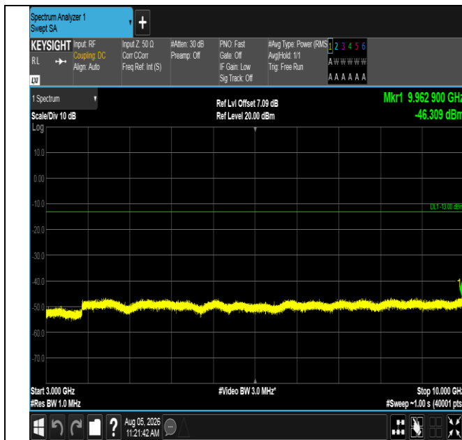
Band12-5MHz-QPSK-23095-1RB#0-3000~10000-PASS
