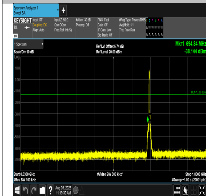
Band12-5MHz-QPSK-23035-25RB#0-30~1000-PASS
