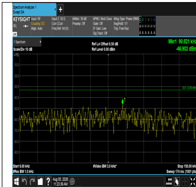
Band12-5MHz-16QAM-23095-1RB#24-0.009~0.15-PASS
