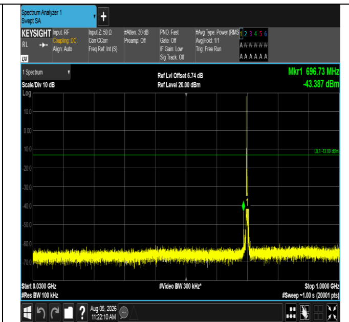
Band12-5MHz-16QAM-23095-1RB#0-30~1000-PASS
