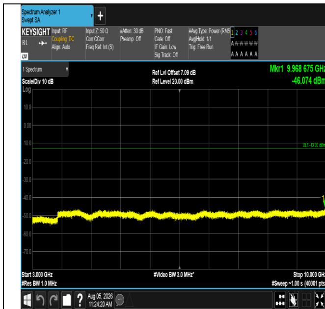
Band12-5MHz-16QAM-23095-1RB#24-3000~10000-PASS
