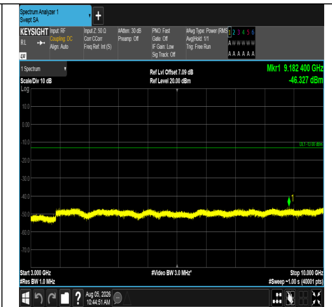
Band12-3MHz-16QAM-23165-15RB#0-3000~10000-PASS
