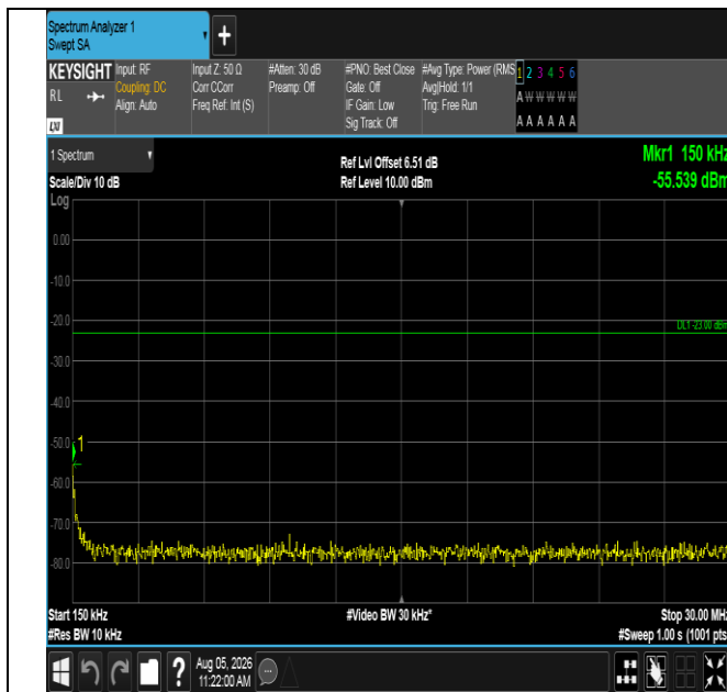
Band12-5MHz-16QAM-23095-1RB#0-0.15~30-PASS
