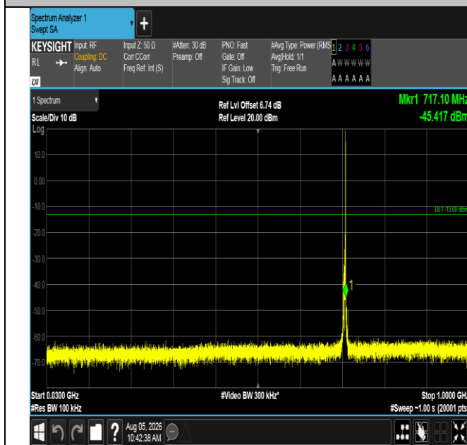
Band12-3MHz-16QAM-23165-1RB#14-30~1000-PASS
