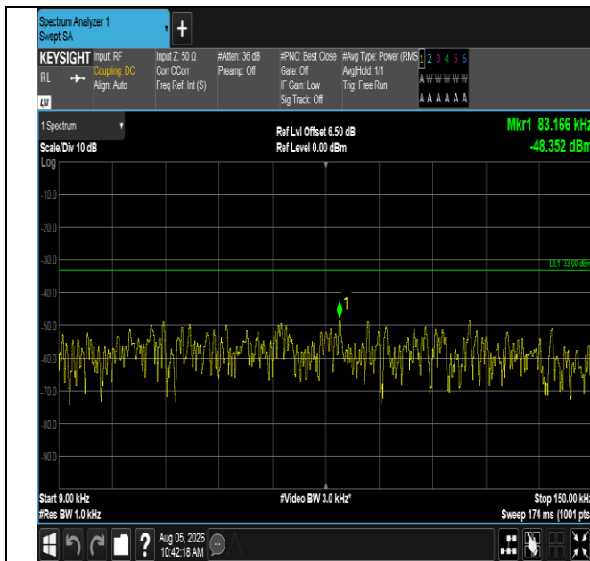
Band12-3MHz-16QAM-23165-1RB#14-0.009~0.15-PASS
