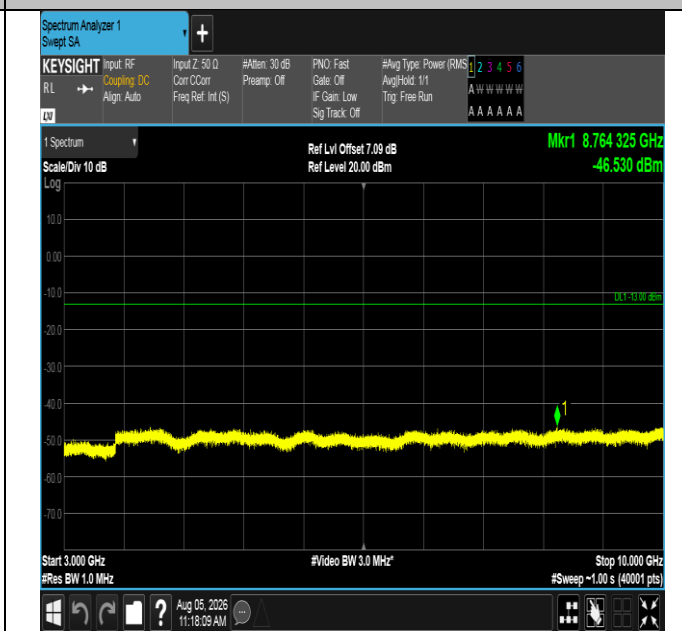
Band12-5MHz-QPSK-23035-1RB#24-3000~10000-PASS
