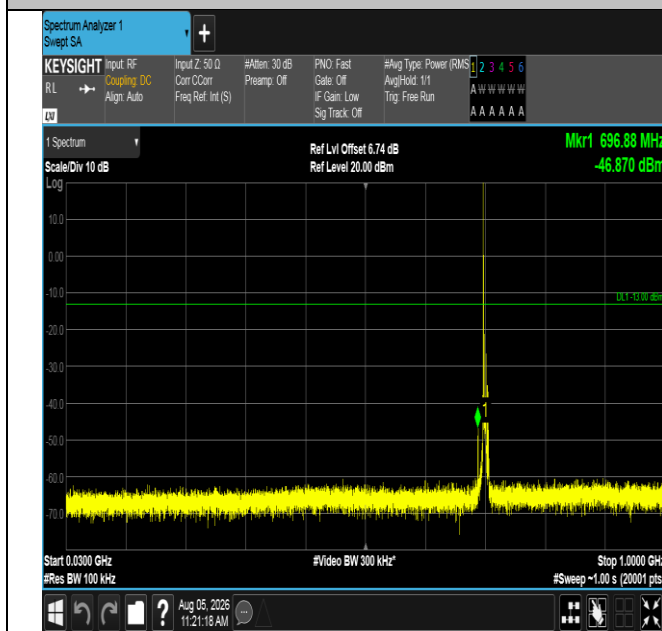
Band12-5MHz-QPSK-23095-1RB#0-30~1000-PASS
