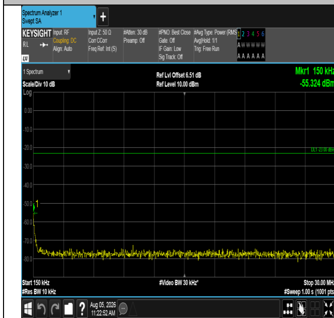
Band12-5MHz-QPSK-23095-1RB#24-0.15~30-PASS
