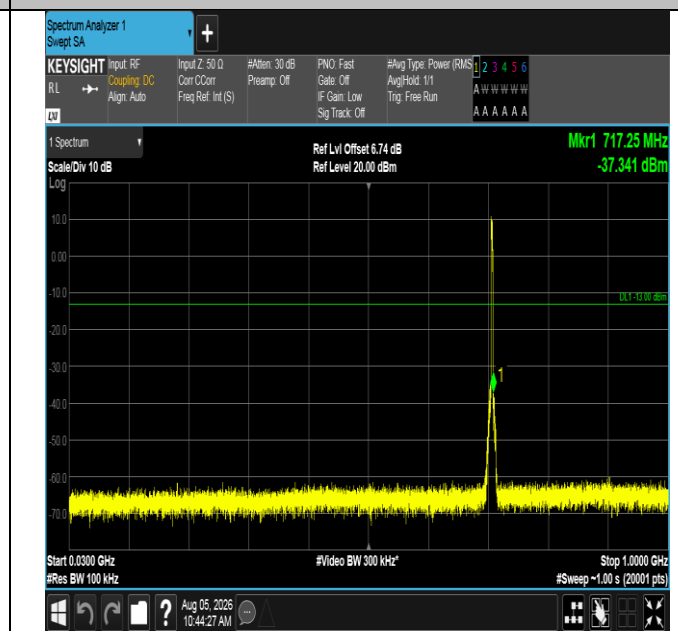
Band12-3MHz-16QAM-23165-15RB#0-30~1000-PASS
