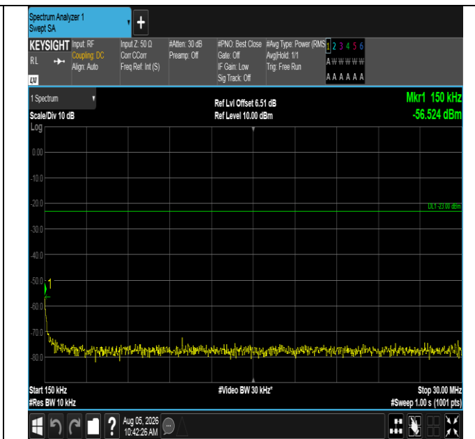
Band12-3MHz-16QAM-23165-1RB#14-0.15~30-PASS
