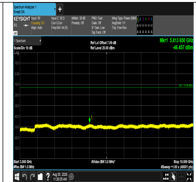
Band12-5MHz-16QAM-23095-25RB#0-3000~10000-PASS
