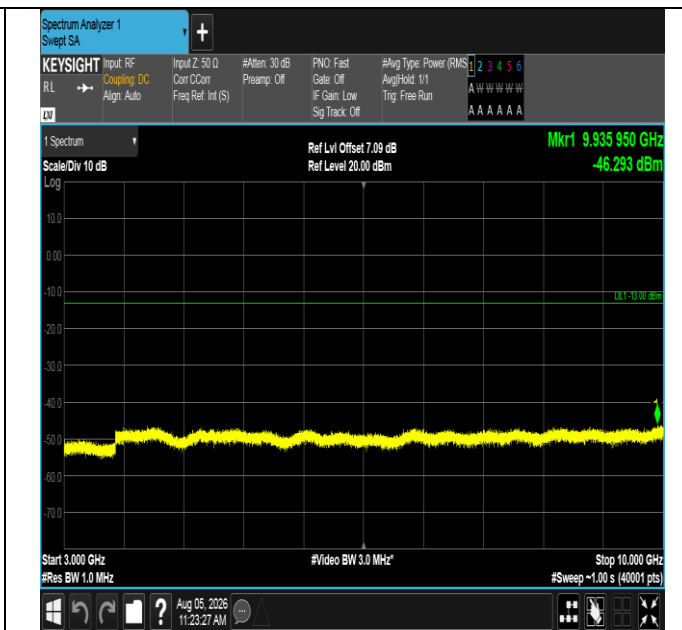
Band12-5MHz-QPSK-23095-1RB#24-3000~10000-PASS
