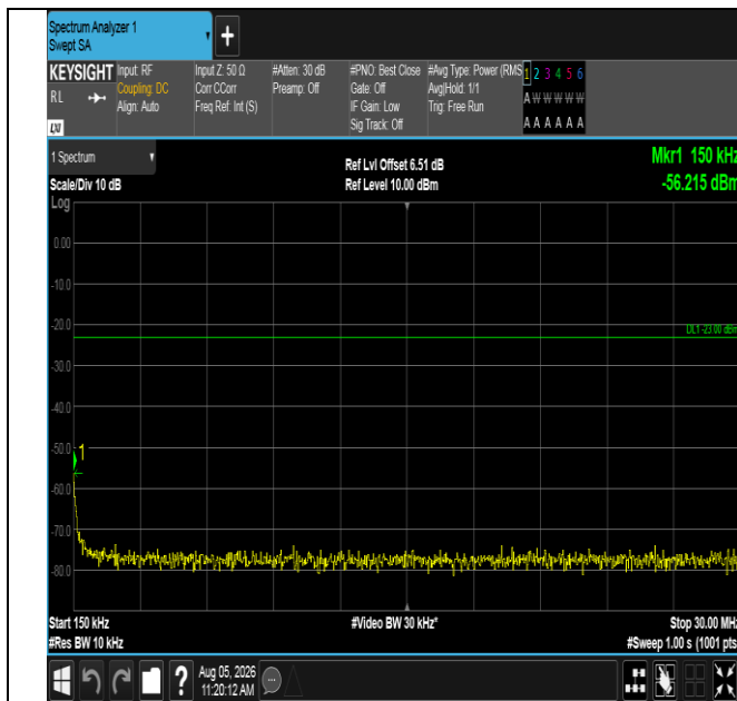
Band12-5MHz-16QAM-23035-25RB#0-0.15~30-PASS
