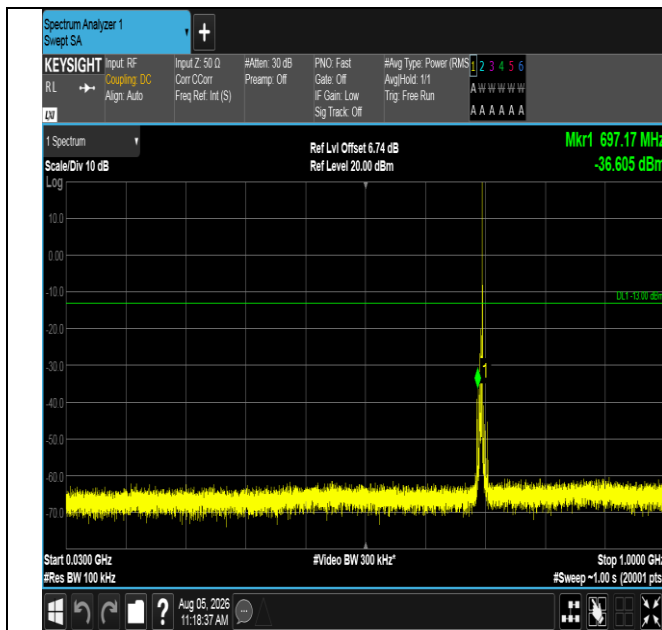
Band12-5MHz-16QAM-23035-1RB#24-30~1000-PASS
