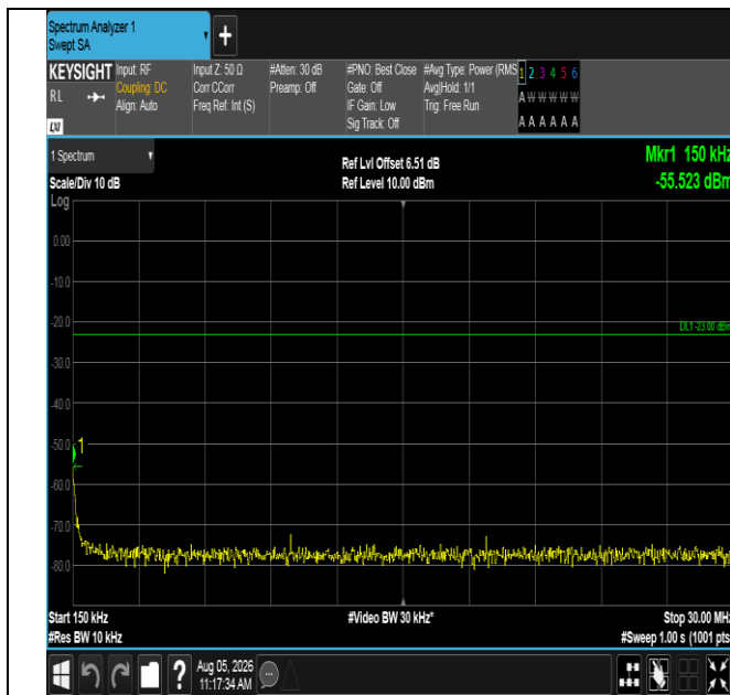
Band12-5MHz-QPSK-23035-1RB#24-0.15~30-PASS
