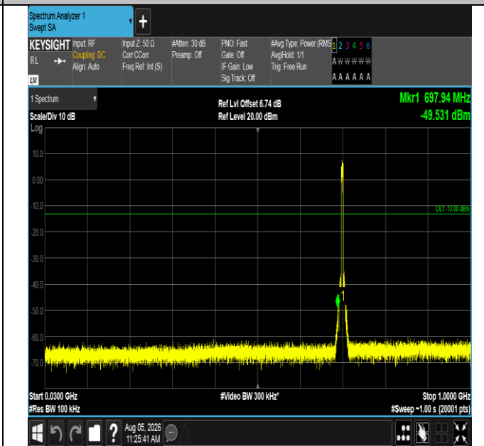
Band12-5MHz-16QAM-23095-25RB#0-30~1000-PASS
