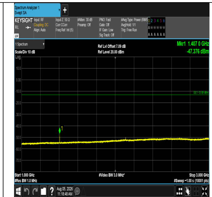
Band12-5MHz-16QAM-23035-1RB#24-1000~3000-PASS
