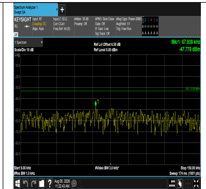
Band12-5MHz-QPSK-23095-1RB#24-0.009~0.15-PASS
