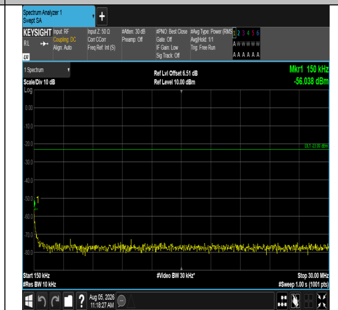
Band12-5MHz-16QAM-23035-1RB#24-0.15~30-PASS
