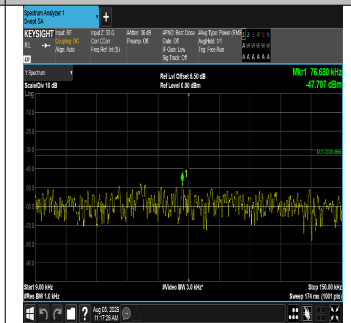
Band12-5MHz-QPSK-23035-1RB#24-0.009~0.15-PASS
