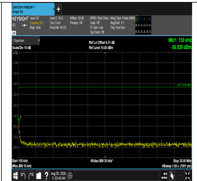
Band12-5MHz-16QAM-23095-1RB#24-0.15~30-PASS
