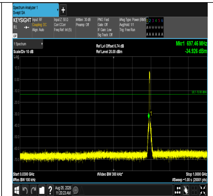
Band12-5MHz-16QAM-23035-25RB#0-30~1000-PASS
