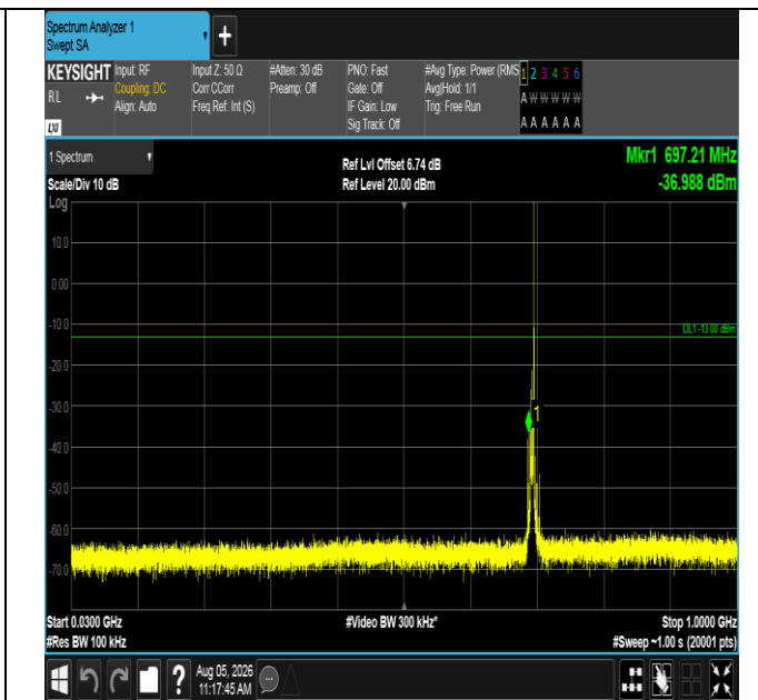
Band12-5MHz-QPSK-23035-1RB#24-30~1000-PASS
