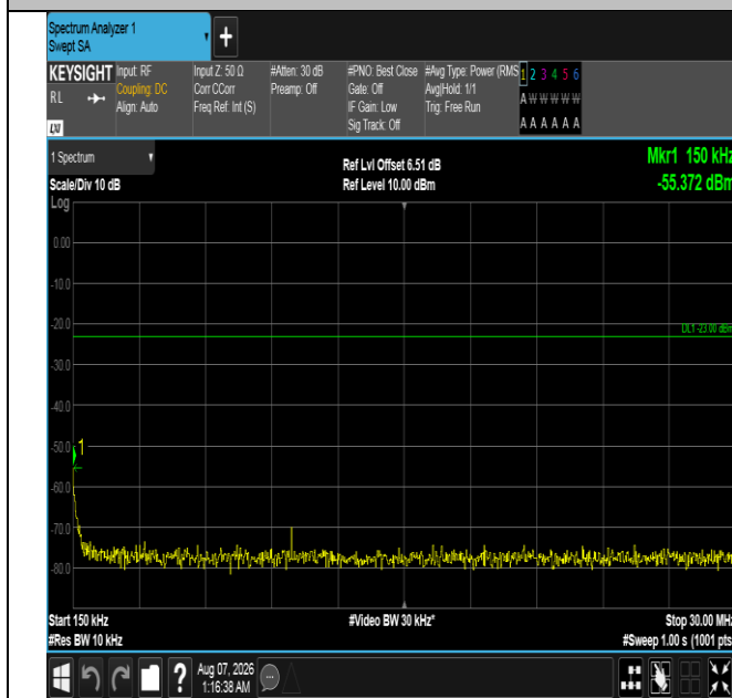
Band12-10MHz-16QAM-23095-1RB#0-0.15~30-PASS
