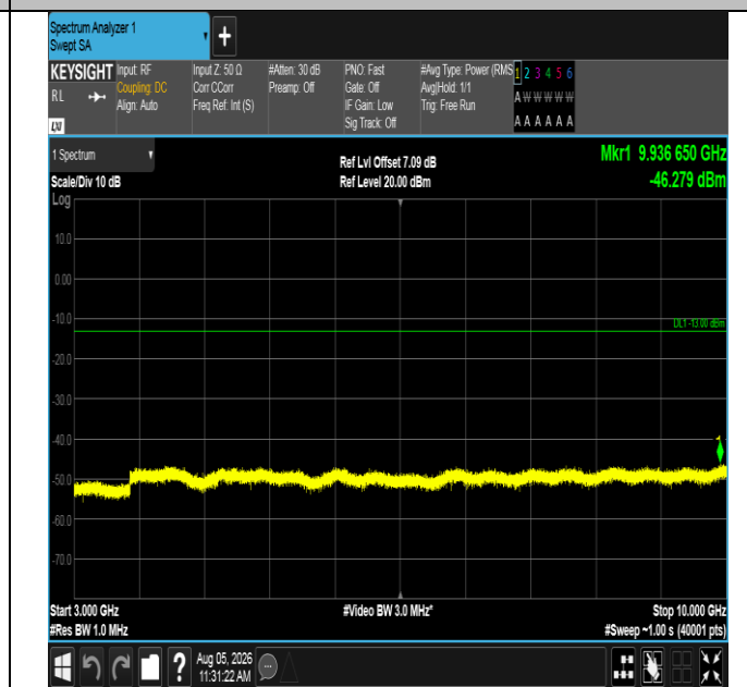
Band12-5MHz-16QAM-23155-25RB#0-3000~10000-PASS
