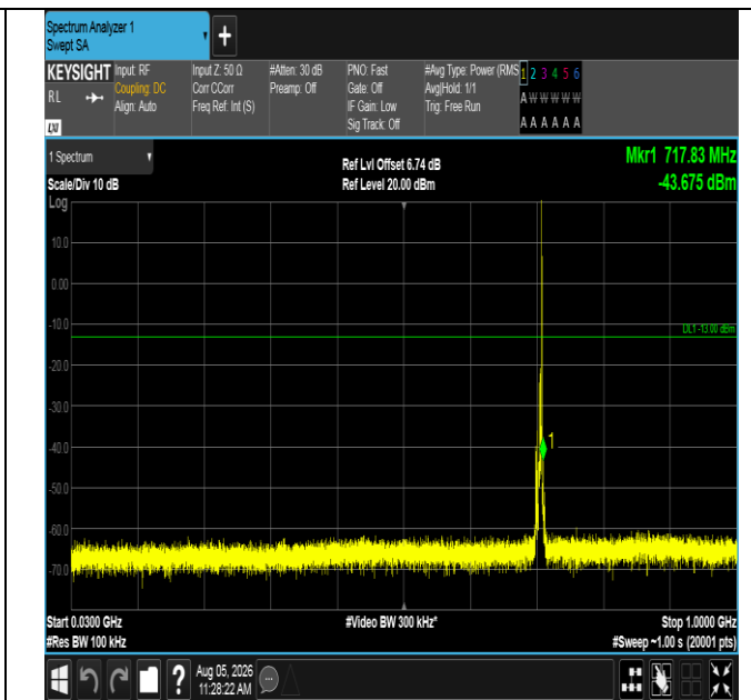
Band12-5MHz-QPSK-23155-1RB#24-30~1000-PASS
