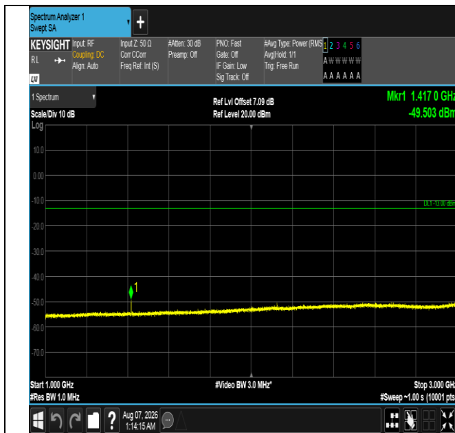
Band12-10MHz-QPSK-23060-1RB#49-1000~3000-PASS
