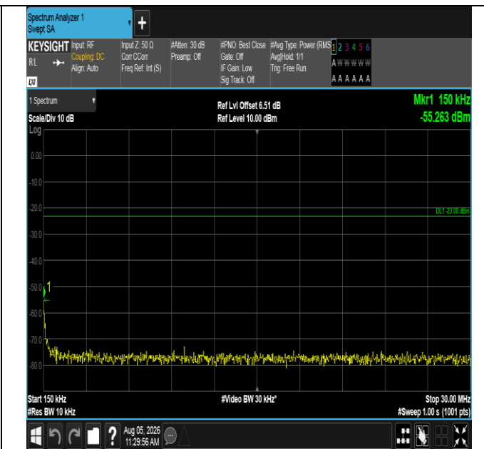
Band12-5MHz-QPSK-23155-25RB#0-0.15~30-PASS
