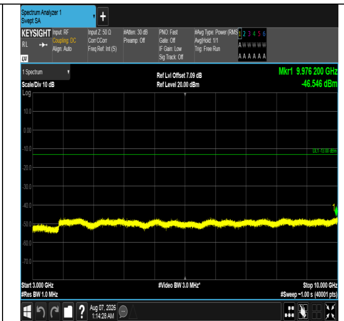
Band12-10MHz-QPSK-23060-1RB#49-3000~10000-PASS
