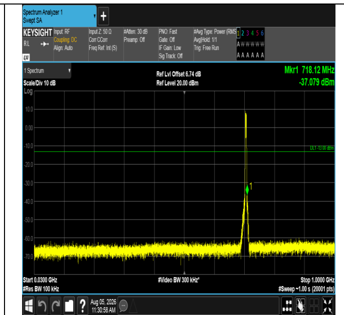
Band12-5MHz-16QAM-23155-25RB#0-30~1000-PASS
