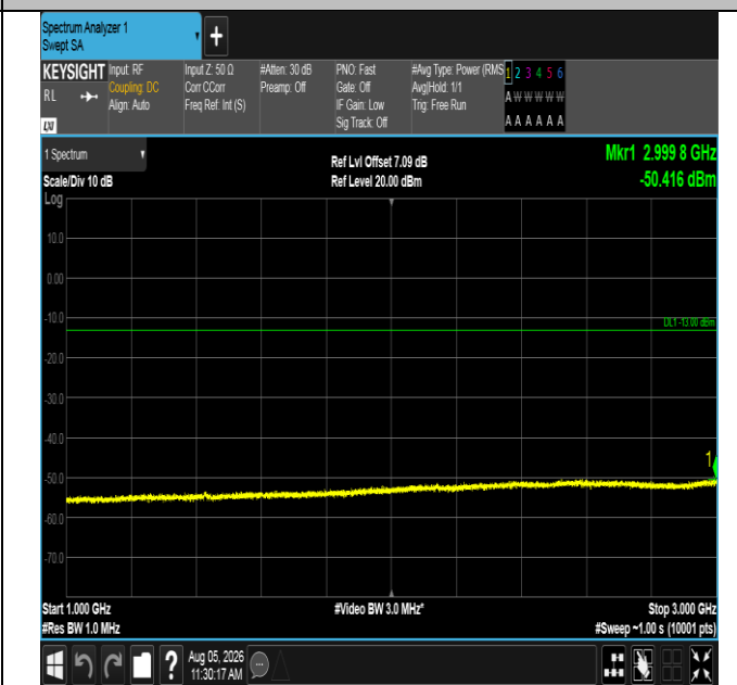
Band12-5MHz-QPSK-23155-25RB#0-1000~3000-PASS
