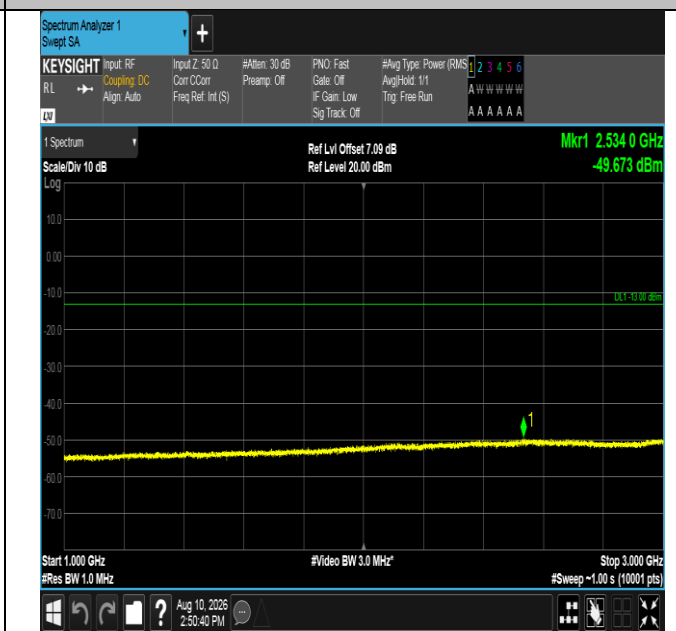
Band12-10MHz-QPSK-23095-50RB#0-1000~3000-PASS
