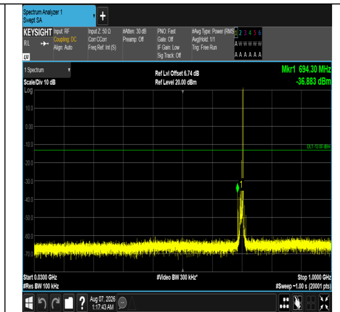
Band12-10MHz-QPSK-23095-1RB#49-30~1000-PASS
