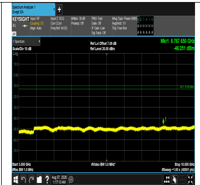
Band12-10MHz-16QAM-23095-1RB#0-3000~10000-PASS
