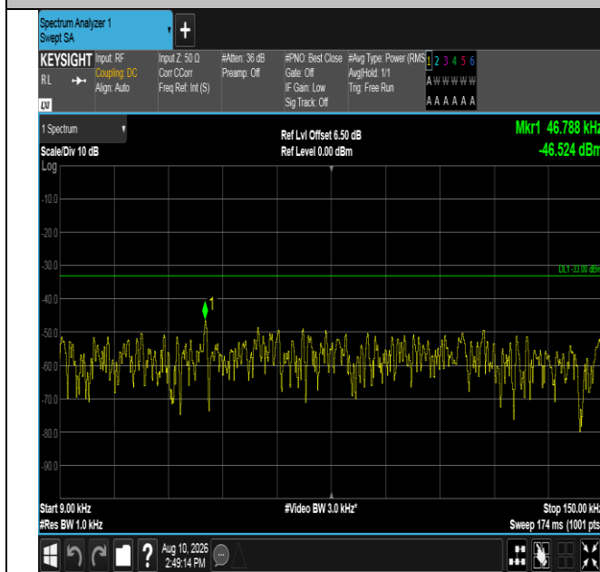
Band12-10MHz-QPSK-23060-50RB#0-0.009~0.15-PASS
