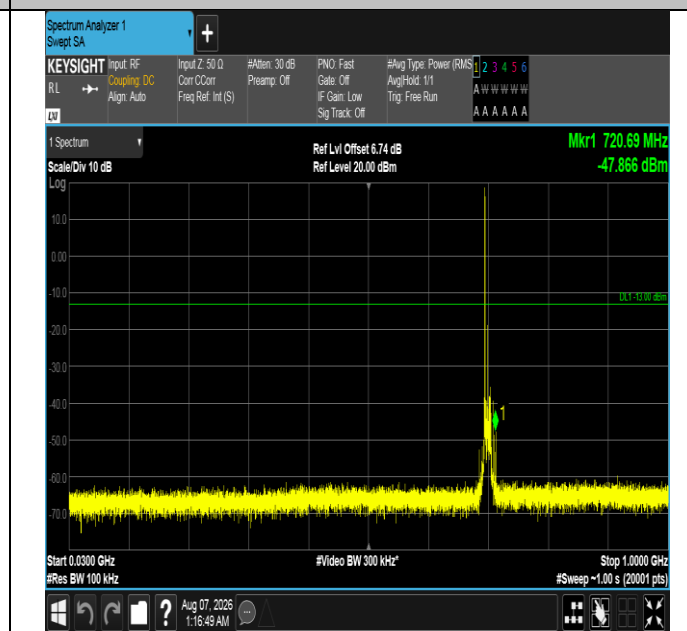
Band12-10MHz-16QAM-23095-1RB#0-30~1000-PASS
