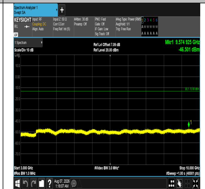
Band12-10MHz-QPSK-23095-1RB#49-3000~10000-PASS
