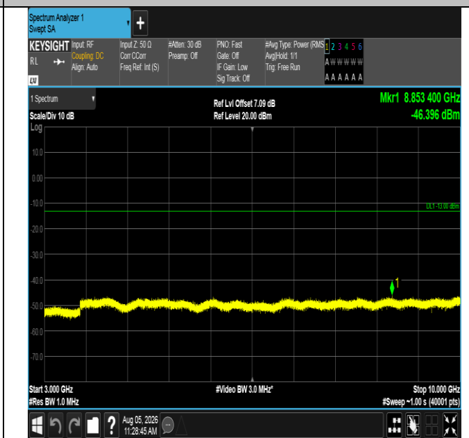
Band12-5MHz-QPSK-23155-1RB#24-3000~10000-PASS
