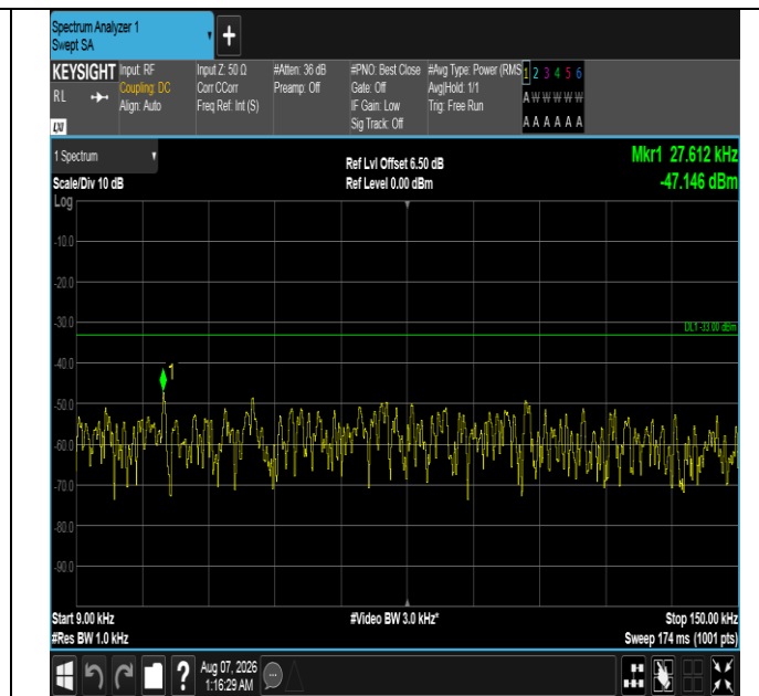
Band12-10MHz-16QAM-23095-1RB#0-0.009~0.15-PASS
