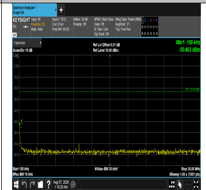
Band12-10MHz-16QAM-23095-1RB#49-0.15~30-PASS
