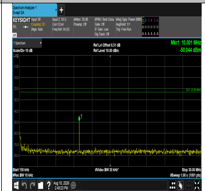
Band12-10MHz-QPSK-23060-50RB#0-0.15~30-PASS
