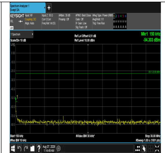
Band12-10MHz-16QAM-23060-1RB#49-0.15~30-PASS
