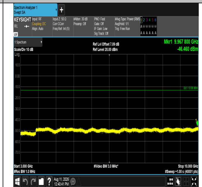
Band12-10MHz-16QAM-23095-50RB#0-3000~10000-PASS
