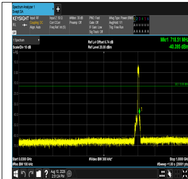
Band12-10MHz-QPSK-23130-50RB#0-30~1000-PASS
