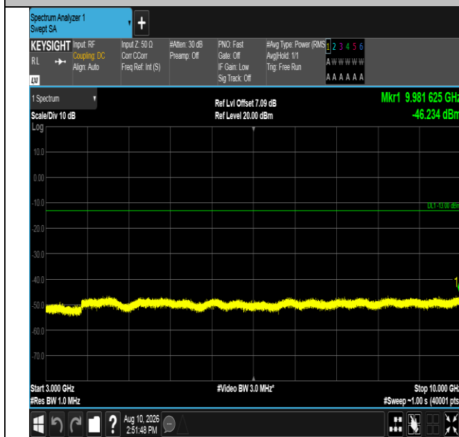
Band12-10MHz-QPSK-23130-50RB#0-3000~10000-PASS
