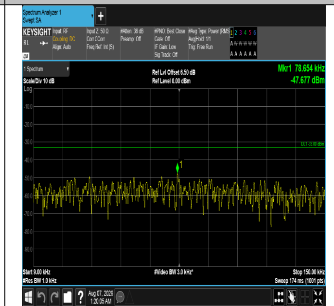
Band12-10MHz-16QAM-23130-1RB#0-0.009~0.15-PASS
