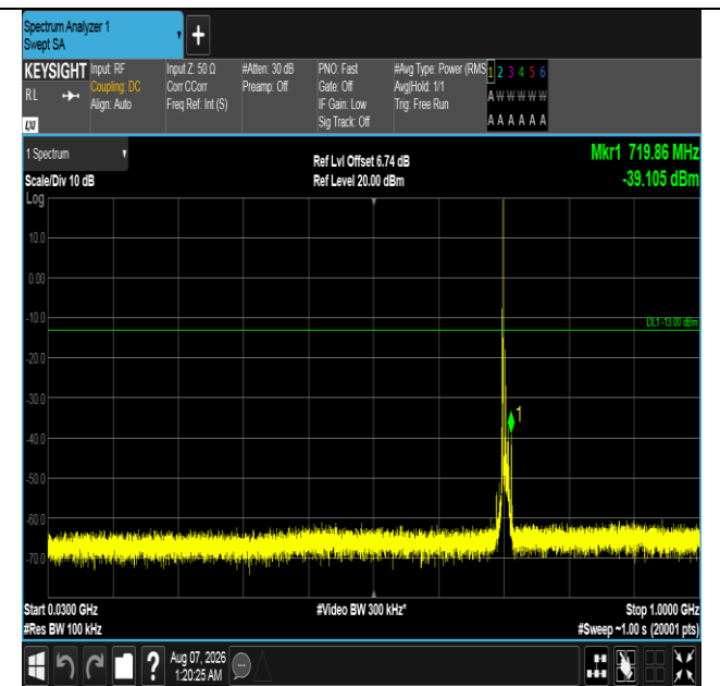
Band12-10MHz-16QAM-23130-1RB#0-30~1000-PASS
