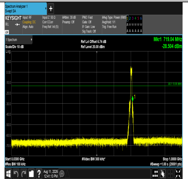
Band12-10MHz-16QAM-23130-50RB#0-30~1000-PASS
