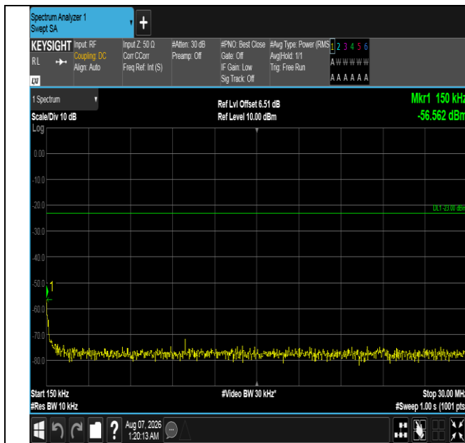
Band12-10MHz-16QAM-23130-1RB#0-0.15~30-PASS
