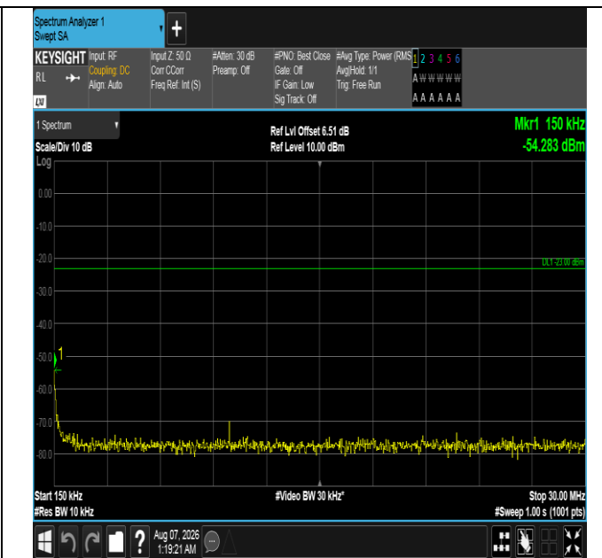
Band12-10MHz-QPSK-23130-1RB#0-0.15~30-PASS
