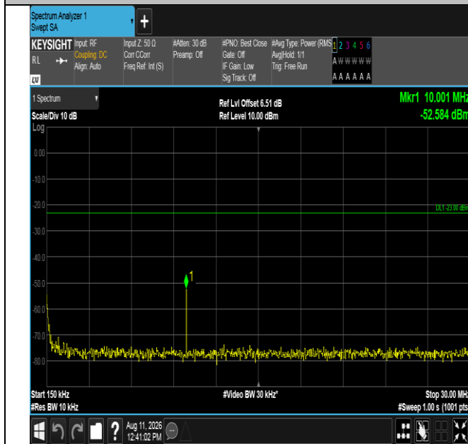
Band12-10MHz-16QAM-23130-50RB#0-0.15~30-PASS
