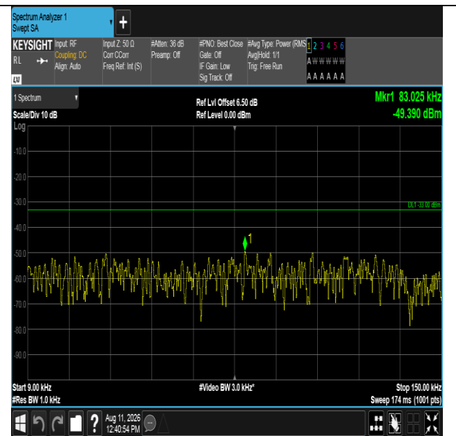
Band12-10MHz-16QAM-23130-50RB#0-0.009~0.15-PASS
