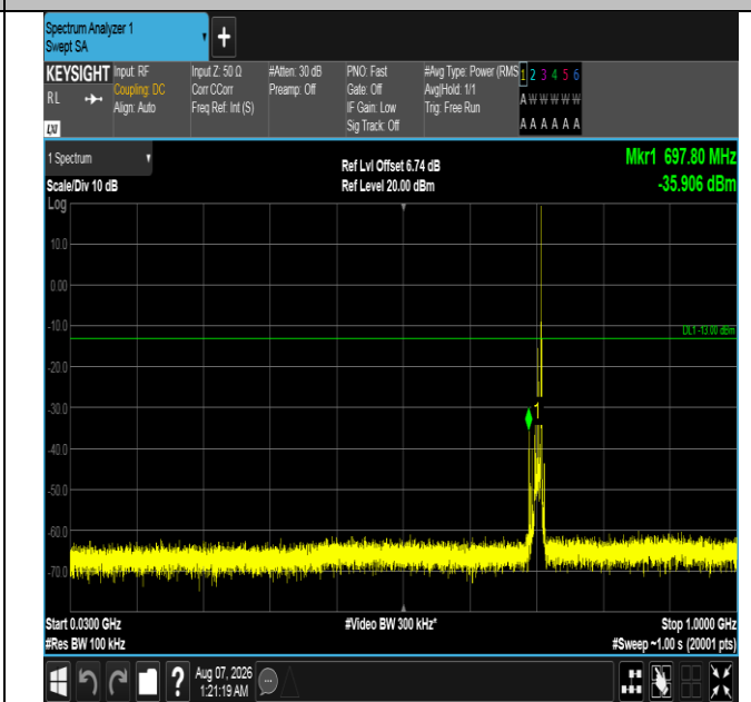
Band12-10MHz-QPSK-23130-1RB#49-30~1000-PASS
