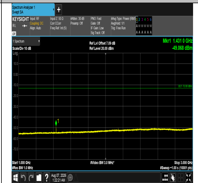
Band12-10MHz-16QAM-23130-1RB#49-1000~3000-PASS
