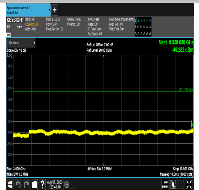
Band12-10MHz-16QAM-23130-1RB#0-3000~10000-PASS
