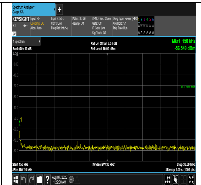
Band12-10MHz-16QAM-23130-1RB#49-0.15~30-PASS
