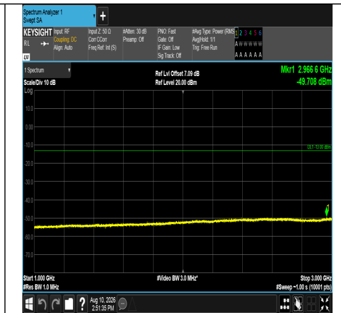
Band12-10MHz-QPSK-23130-50RB#0-1000~3000-PASS
