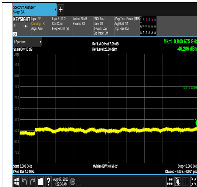
Band12-10MHz-16QAM-23130-1RB#49-3000~10000-PASS
