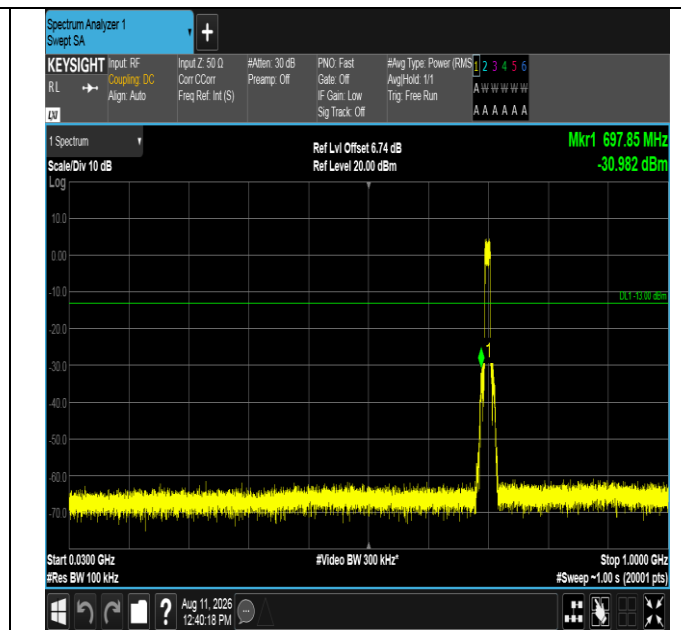
Band12-10MHz-16QAM-23095-50RB#0-30~1000-PASS
