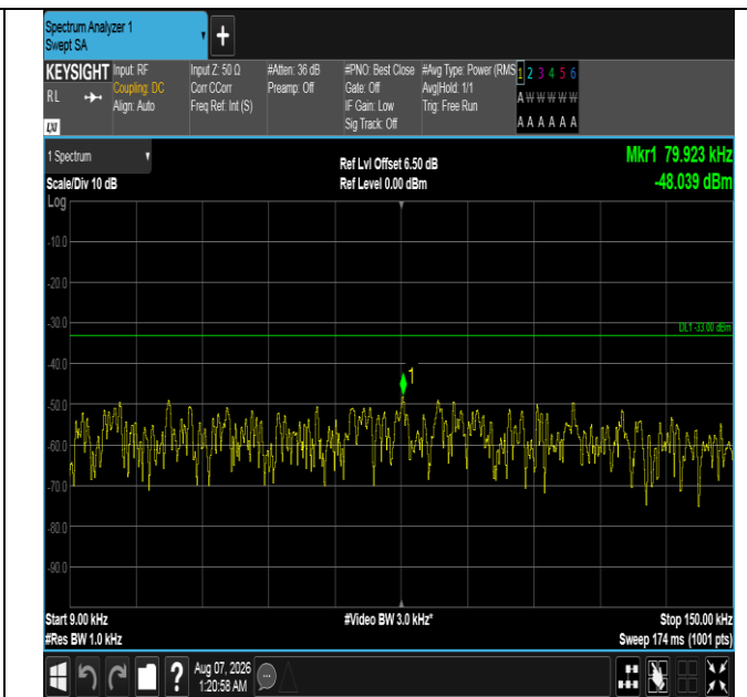
Band12-10MHz-QPSK-23130-1RB#49-0.009~0.15-PASS
