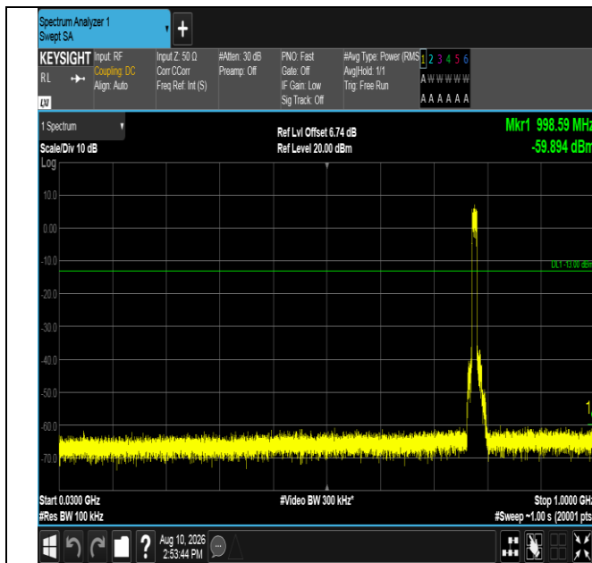
Band13-10MHz-QPSK-23230-50RB#0-30~1000-PASS
