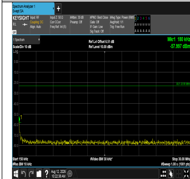
Band13-10MHz-16QAM-23230-50RB#0-0.15~30-PASS
