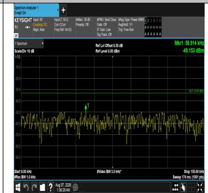
Band13-10MHz-16QAM-23230-1RB#0-0.009~0.15-PASS
