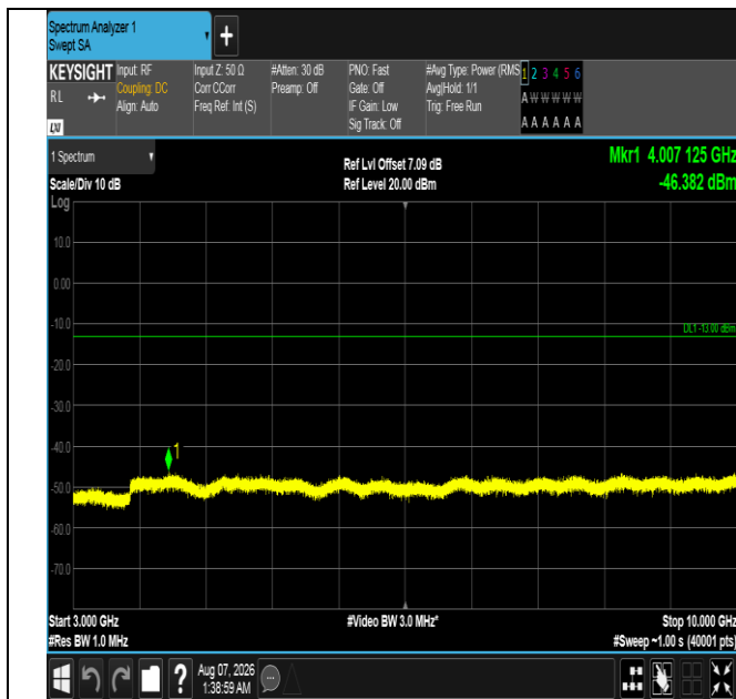
Band13-10MHz-16QAM-23230-1RB#49-3000~10000-PASS
