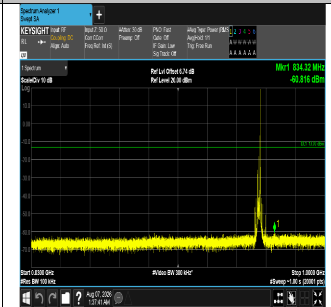
Band13-10MHz-QPSK-23230-1RB#49-30~1000-PASS
