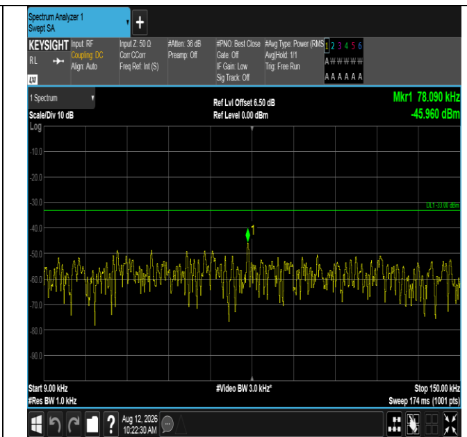
Band13-10MHz-16QAM-23230-50RB#0-0.009~0.15-PASS
