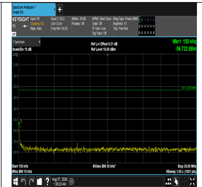
Band13-10MHz-16QAM-23230-1RB#49-0.15~30-PASS
