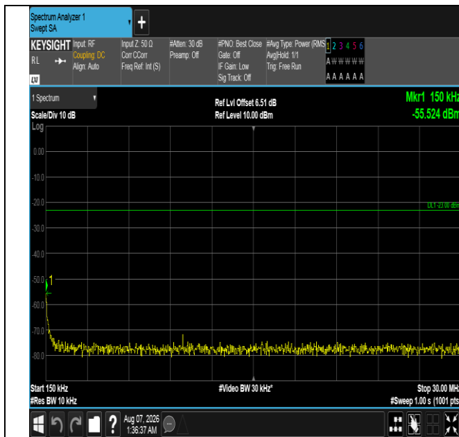
Band13-10MHz-16QAM-23230-1RB#0-0.15~30-PASS
