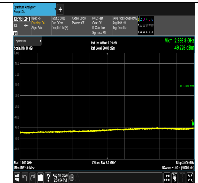
Band13-10MHz-QPSK-23230-50RB#0-1000~3000-PASS
