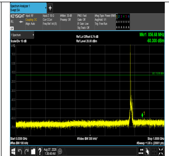
Band13-10MHz-16QAM-23230-1RB#0-30~1000-PASS
