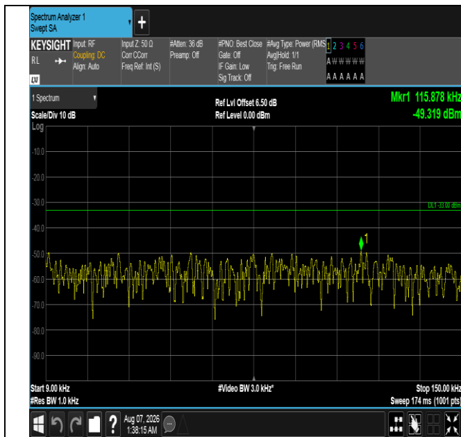
Band13-10MHz-16QAM-23230-1RB#49-0.009~0.15-PASS
