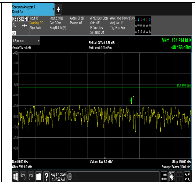
Band13-10MHz-QPSK-23230-1RB#49-0.009~0.15-PASS
