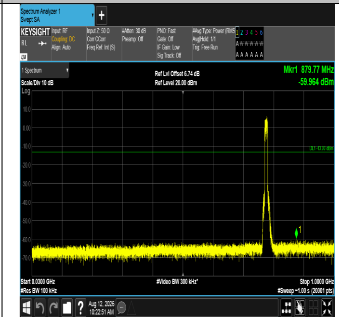
Band13-10MHz-16QAM-23230-50RB#0-30~1000-PASS
