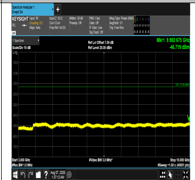
Band13-10MHz-16QAM-23230-1RB#0-3000~10000-PASS
