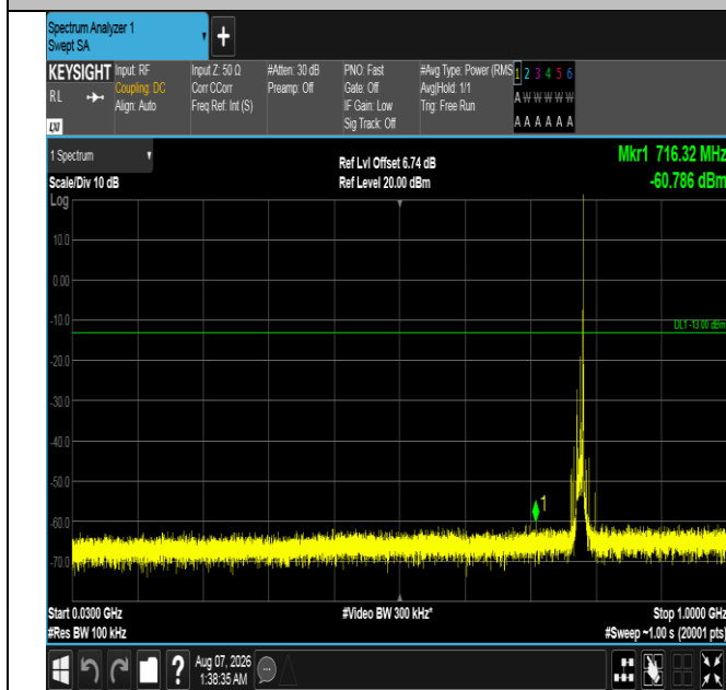
Band13-10MHz-16QAM-23230-1RB#49-30~1000-PASS
