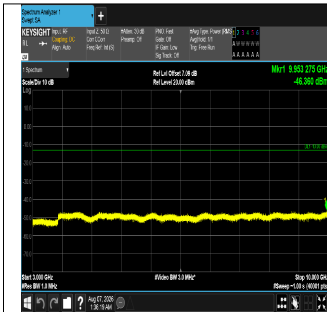
Band13-10MHz-QPSK-23230-1RB#0-3000~10000-PASS
