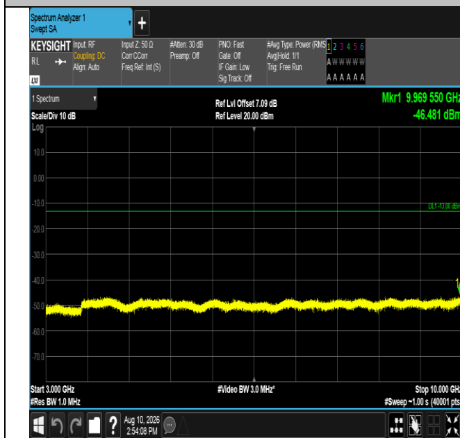
Band13-10MHz-QPSK-23230-50RB#0-3000~10000-PASS
