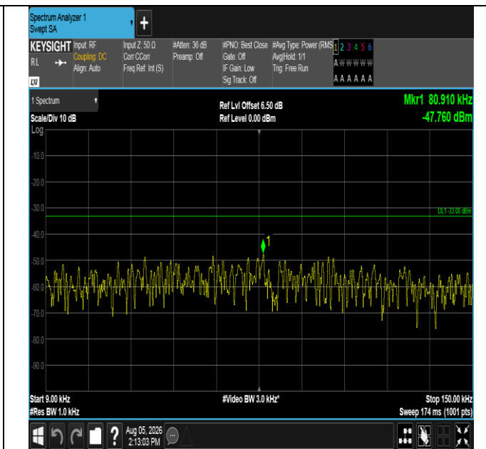
Band17-5MHz-16QAM-23825-25RB#0-0.009~0.15-PASS
