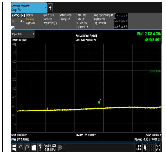
Band17-5MHz-16QAM-23790-1RB#24-1000~3000-PASS
