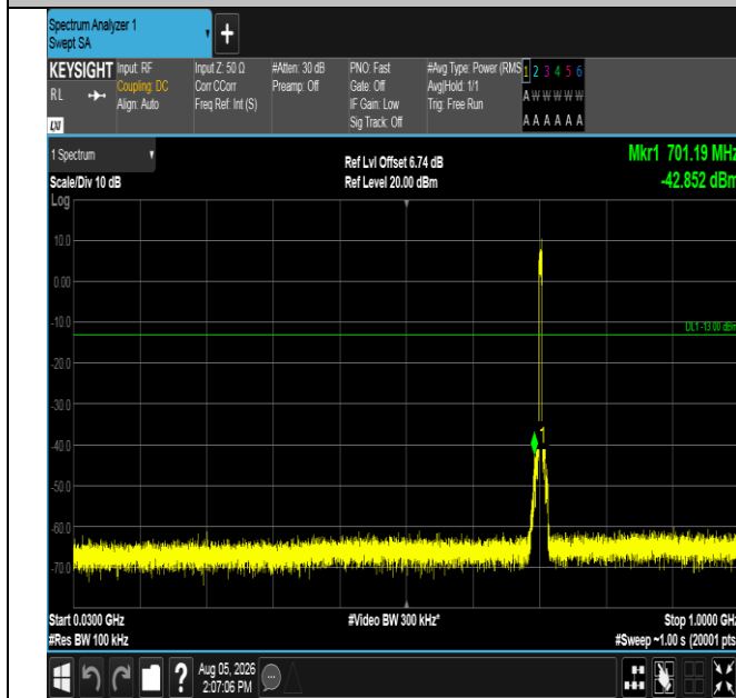
Band17-5MHz-QPSK-23790-25RB#0-30~1000-PASS
