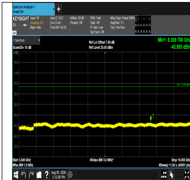
Band17-5MHz-16QAM-23825-1RB#24-3000~10000-PASS
