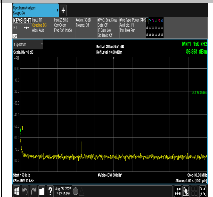
Band17-5MHz-QPSK-23825-25RB#0-0.15~30-PASS
