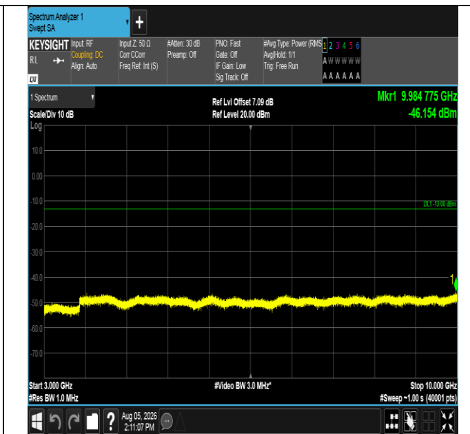
Band17-5MHz-QPSK-23825-1RB#24-3000~10000-PASS
