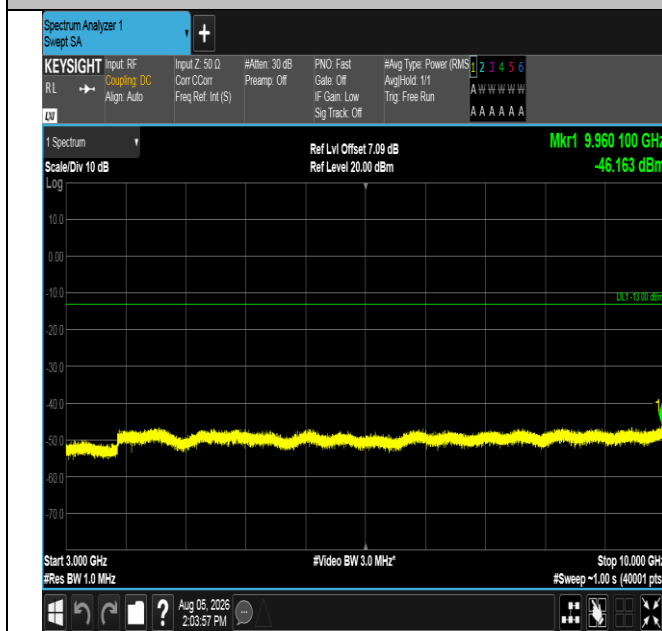
Band17-5MHz-QPSK-23790-1RB#0-3000~10000-PASS
