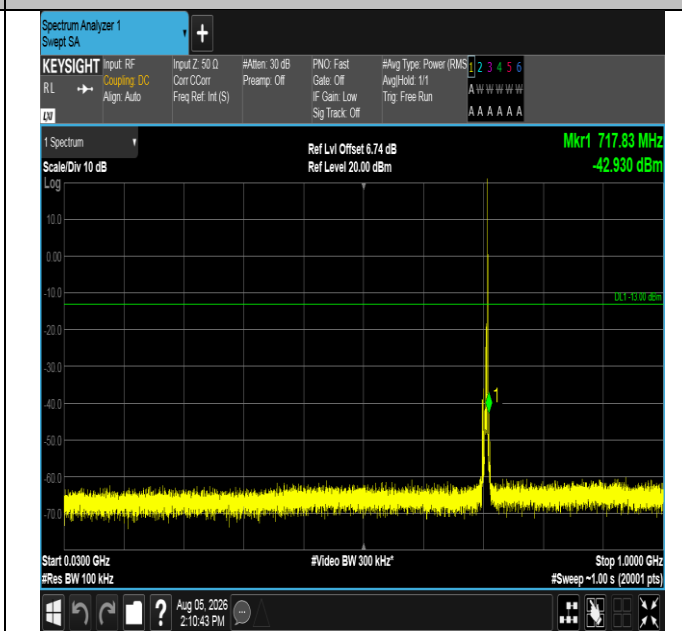
Band17-5MHz-QPSK-23825-1RB#24-30~1000-PASS
