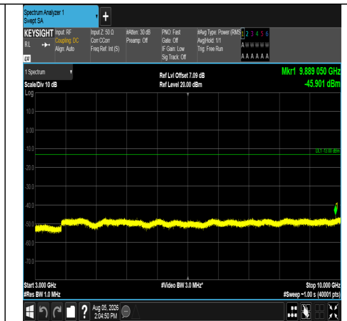
Band17-5MHz-16QAM-23790-1RB#0-3000~10000-PASS
