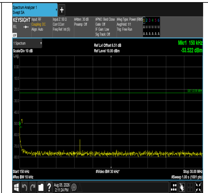
Band17-5MHz-16QAM-23825-1RB#24-0.15~30-PASS
