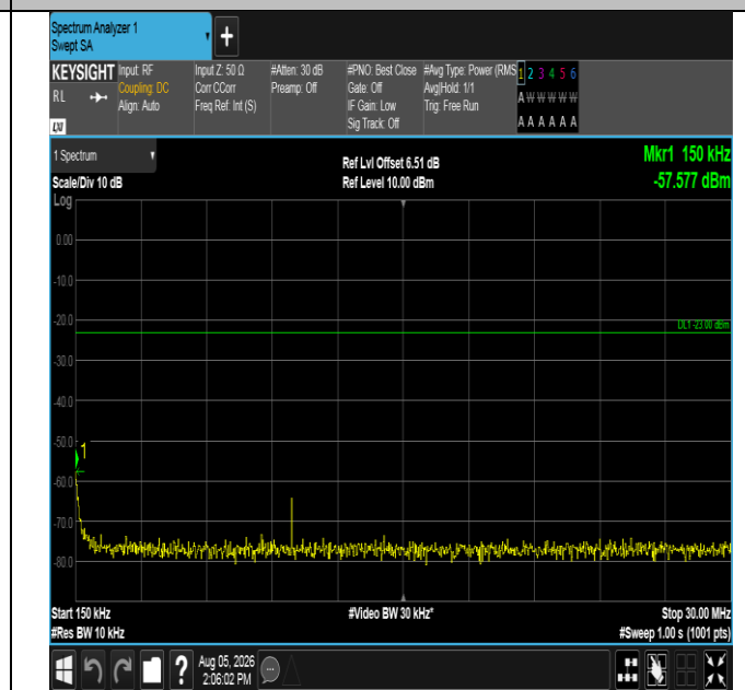
Band17-5MHz-16QAM-23790-1RB#24-0.15~30-PASS
