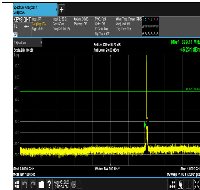
Band17-5MHz-QPSK-23790-1RB#0-30~1000-PASS
