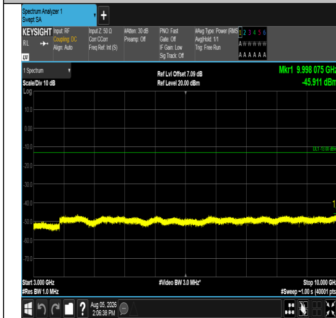
Band17-5MHz-16QAM-23790-1RB#24-3000~10000-PASS
