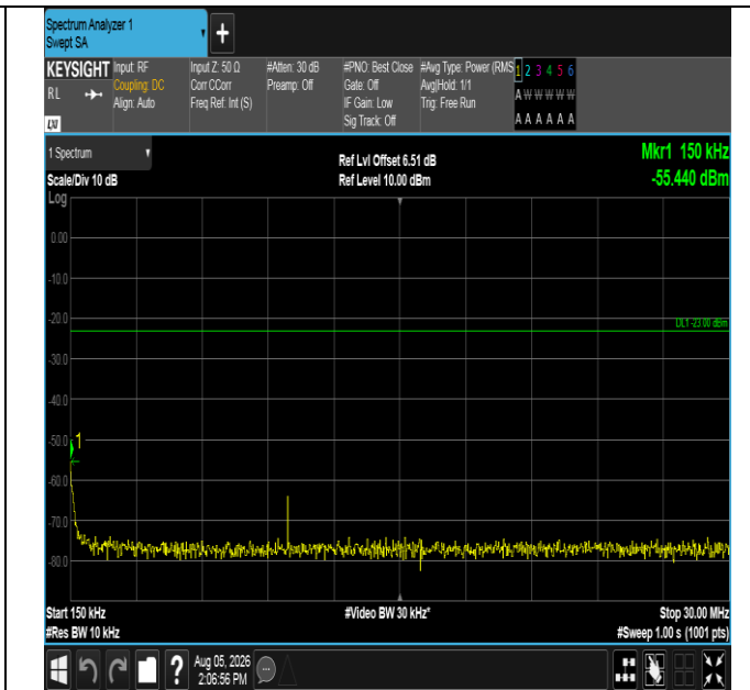
Band17-5MHz-QPSK-23790-25RB#0-0.15~30-PASS
