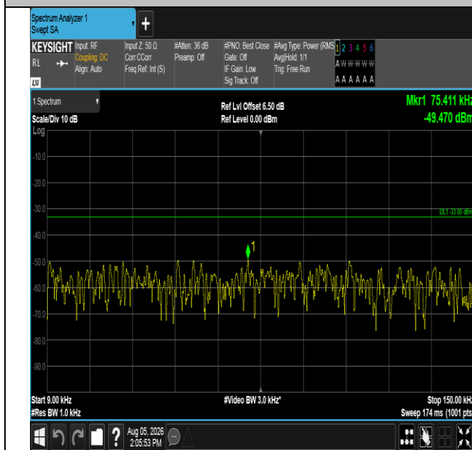
Band17-5MHz-16QAM-23790-1RB#24-0.009~0.15-PASS
