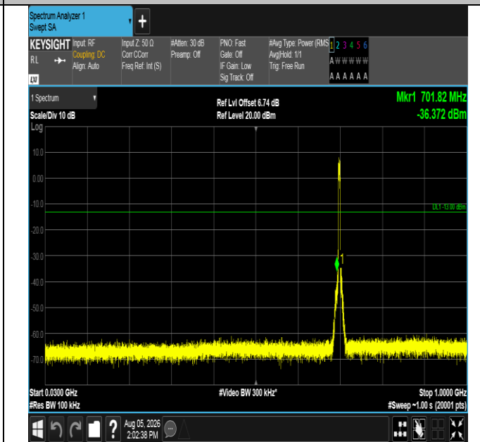
Band17-5MHz-16QAM-23755-25RB#0-30~1000-PASS
