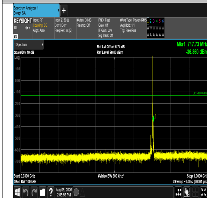
Band17-5MHz-QPSK-23825-1RB#0-30~1000-PASS
