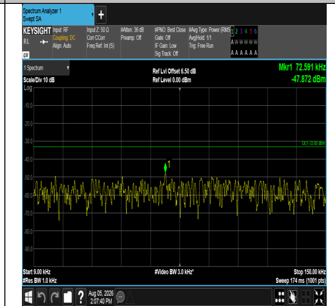
Band17-5MHz-16QAM-23790-25RB#0-0.009~0.15-PASS
