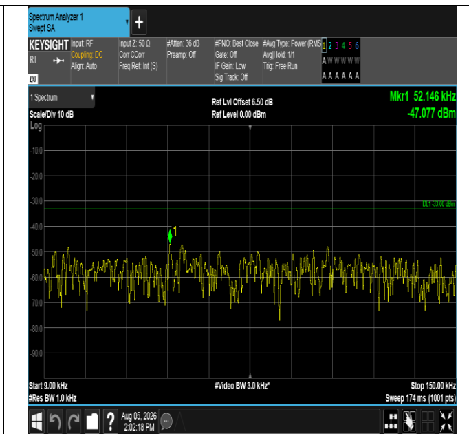
Band17-5MHz-16QAM-23755-25RB#0-0.009~0.15-PASS
