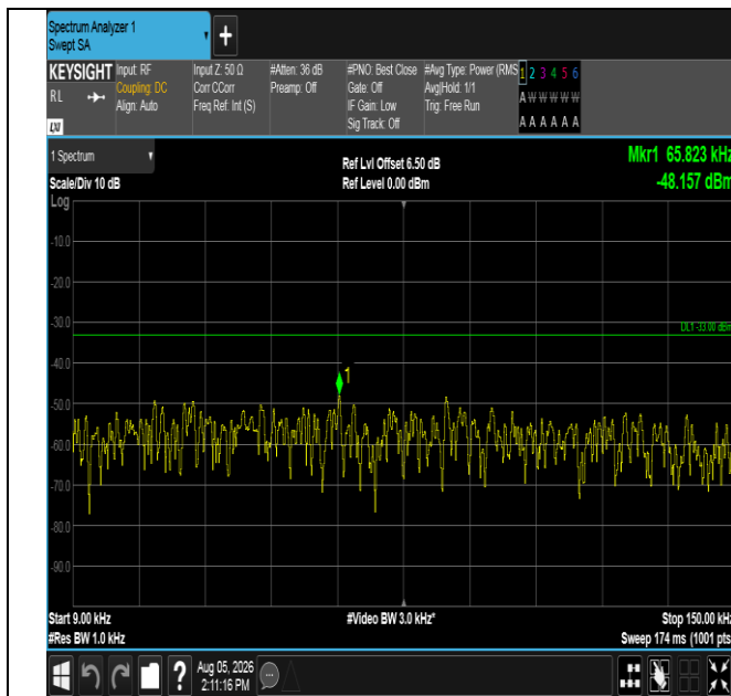
Band17-5MHz-16QAM-23825-1RB#24-0.009~0.15-PASS
