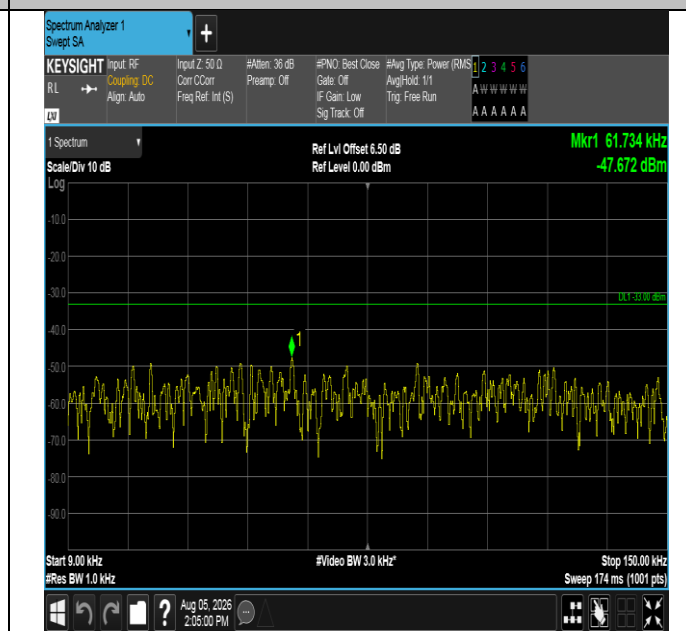
Band17-5MHz-QPSK-23790-1RB#24-0.009~0.15-PASS
