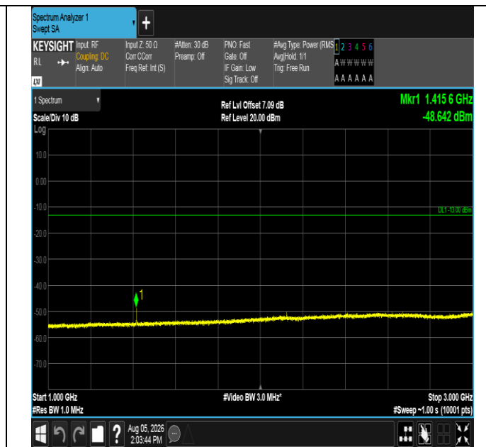
Band17-5MHz-QPSK-23790-1RB#0-1000~3000-PASS
