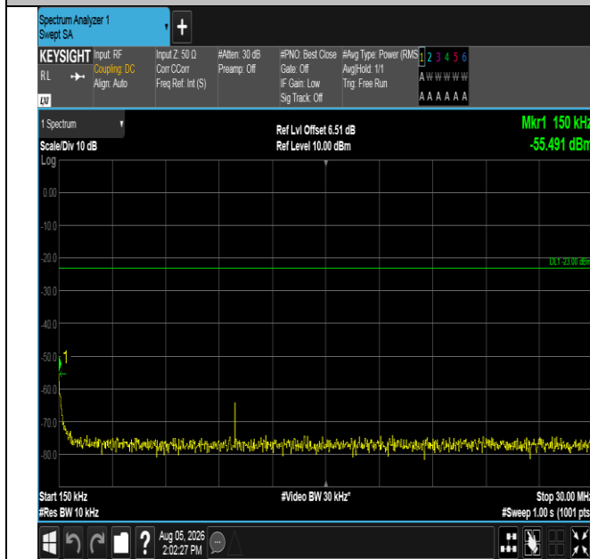
Band17-5MHz-16QAM-23755-25RB#0-0.15~30-PASS
