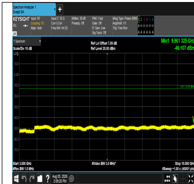
Band17-5MHz-QPSK-23825-1RB#0-3000~10000-PASS
