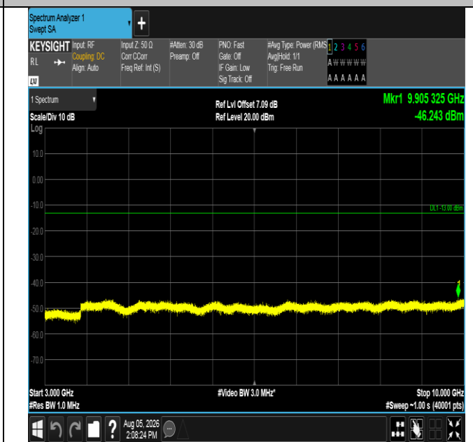
Band17-5MHz-16QAM-23790-25RB#0-3000~10000-PASS
