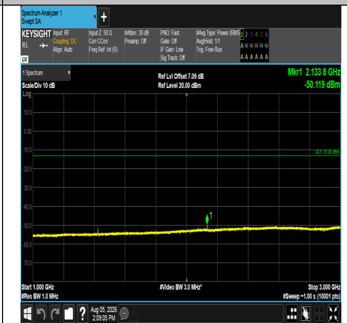
Band17-5MHz-QPSK-23825-1RB#0-1000~3000-PASS
