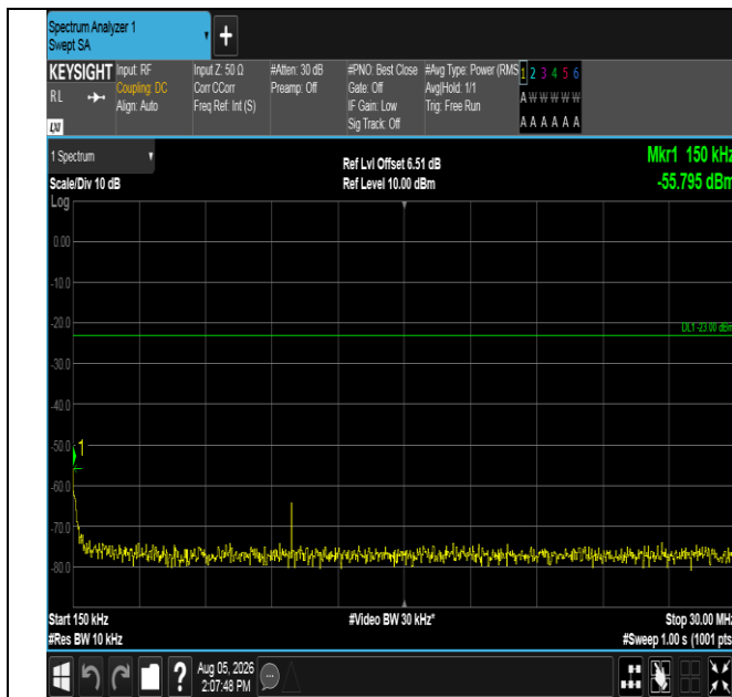
Band17-5MHz-16QAM-23790-25RB#0-0.15~30-PASS
