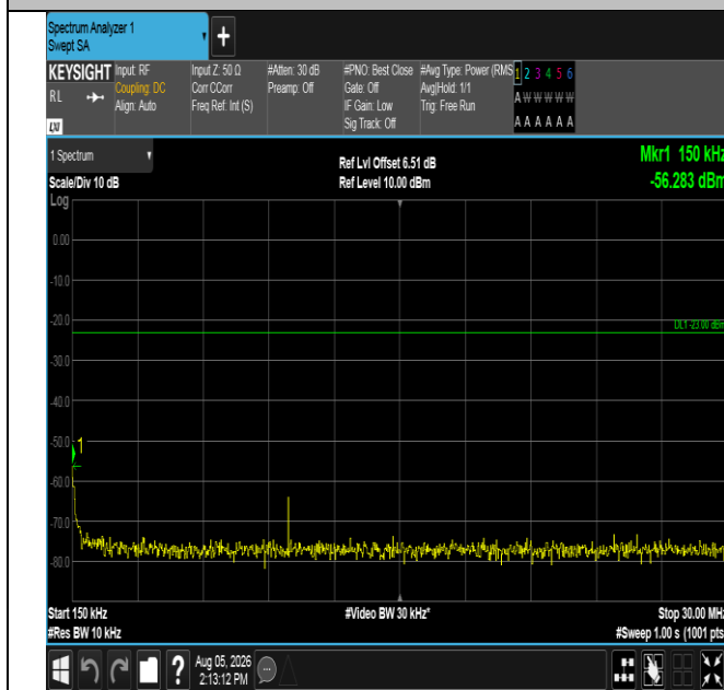
Band17-5MHz-16QAM-23825-25RB#0-0.15~30-PASS
