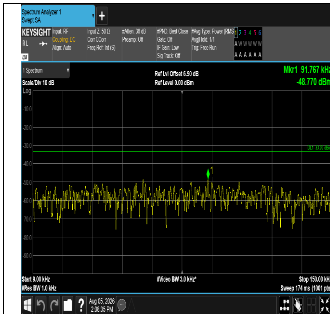
Band17-5MHz-QPSK-23825-1RB#0-0.009~0.15-PASS
