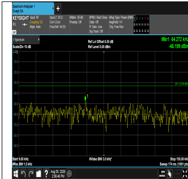
Band17-5MHz-QPSK-23790-25RB#0-0.009~0.15-PASS
