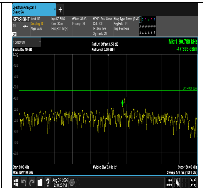
Band17-5MHz-QPSK-23825-1RB#24-0.009~0.15-PASS
