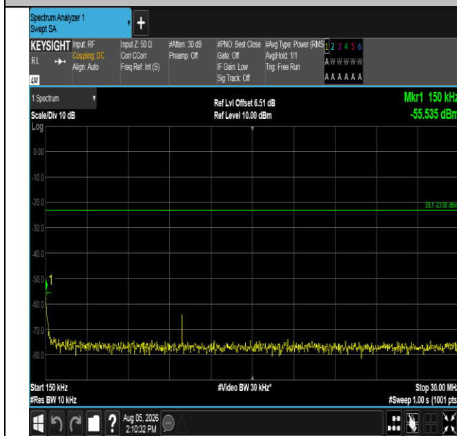
Band17-5MHz-QPSK-23825-1RB#24-0.15~30-PASS
