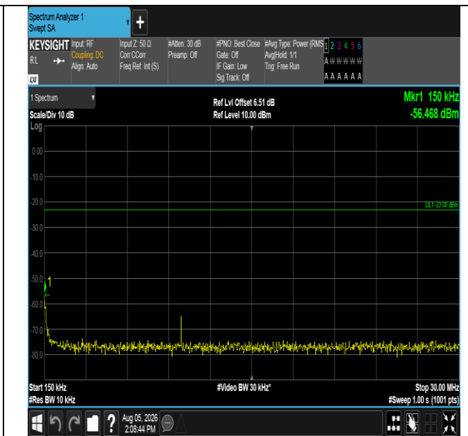
Band17-5MHz-QPSK-23825-1RB#0-0.15~30-PASS
