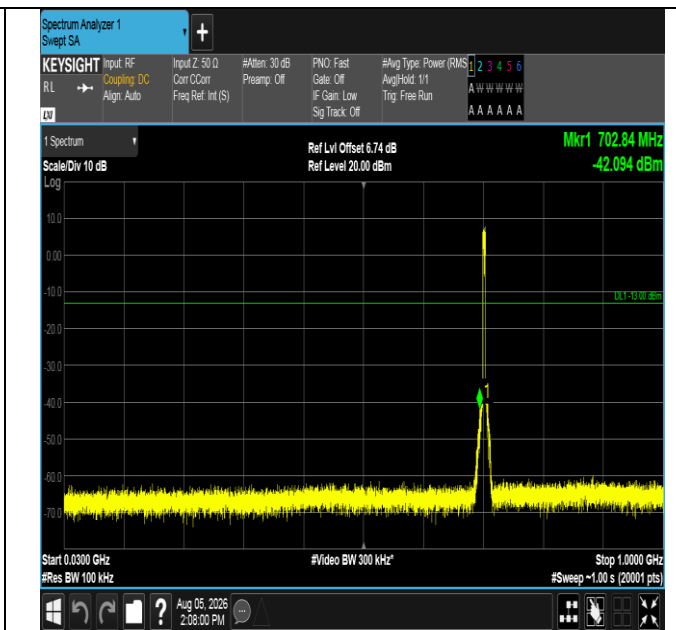
Band17-5MHz-16QAM-23790-25RB#0-30~1000-PASS
