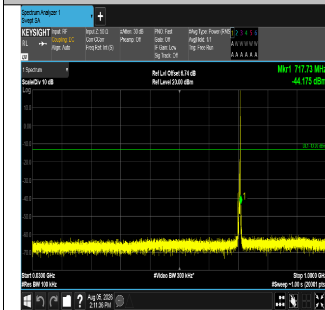
Band17-5MHz-16QAM-23825-1RB#24-30~1000-PASS
