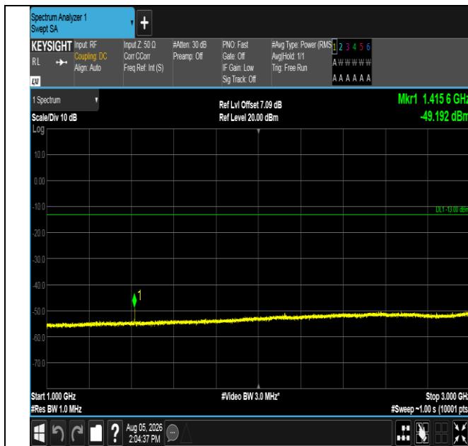
Band17-5MHz-16QAM-23790-1RB#0-1000~3000-PASS
