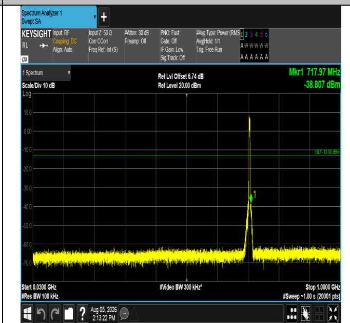
Band17-5MHz-16QAM-23825-25RB#0-30~1000-PASS
