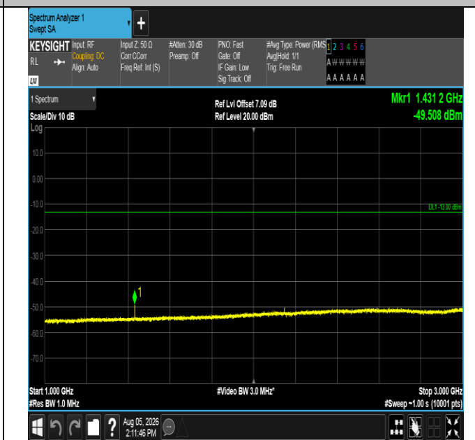
Band17-5MHz-16QAM-23825-1RB#24-1000~3000-PASS
