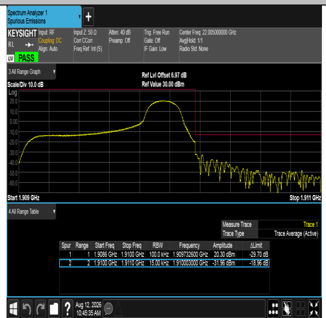
Band2-1.4MHz-QPSK-19193-1RB#5-PASS
