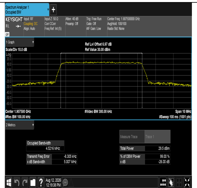
Band2-5MHz-16QAM-19175-25RB#0-PASS
