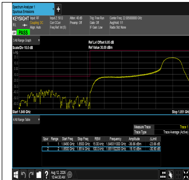
Band2-1.4MHz-16QAM-18607-1RB#5-PASS
