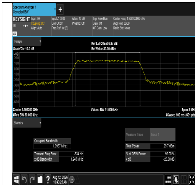
Band2-1.4MHz-QPSK-19193-6RB#0-PASS
