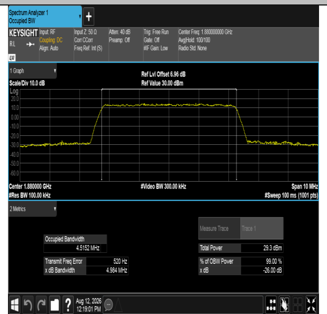
Band2-5MHz-16QAM-18900-25RB#0-PASS
