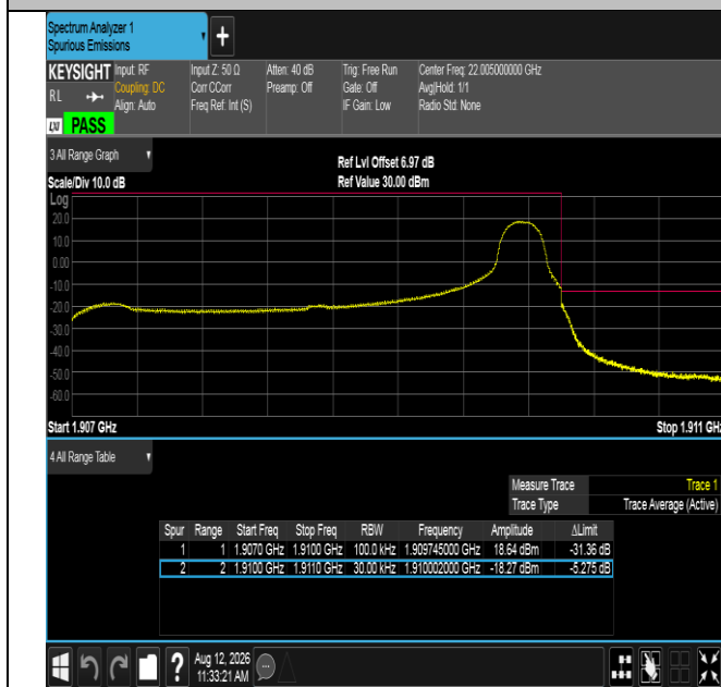
Band2-3MHz-16QAM-19185-1RB#14-PASS
