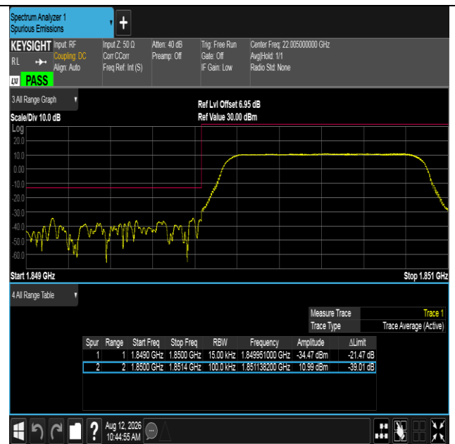
Band2-1.4MHz-16QAM-18607-6RB#0-PASS
