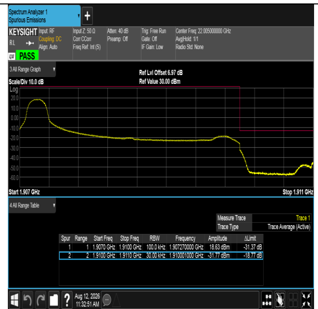
Band2-3MHz-16QAM-19185-1RB#0-PASS
