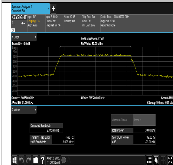
Band2-3MHz-QPSK-19185-15RB#0-PASS
