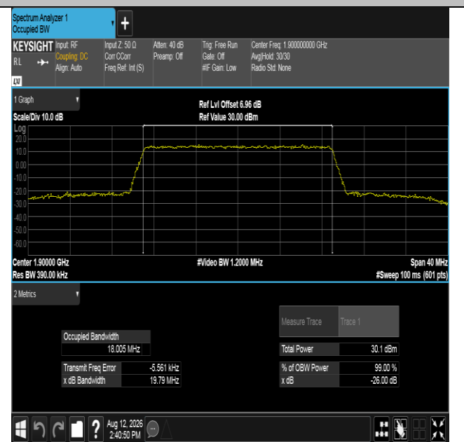
Band2-20MHz-16QAM-19100-100RB#0-PASS
