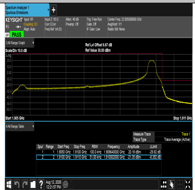
Band2-5MHz-QPSK-19175-1RB#24-PASS
