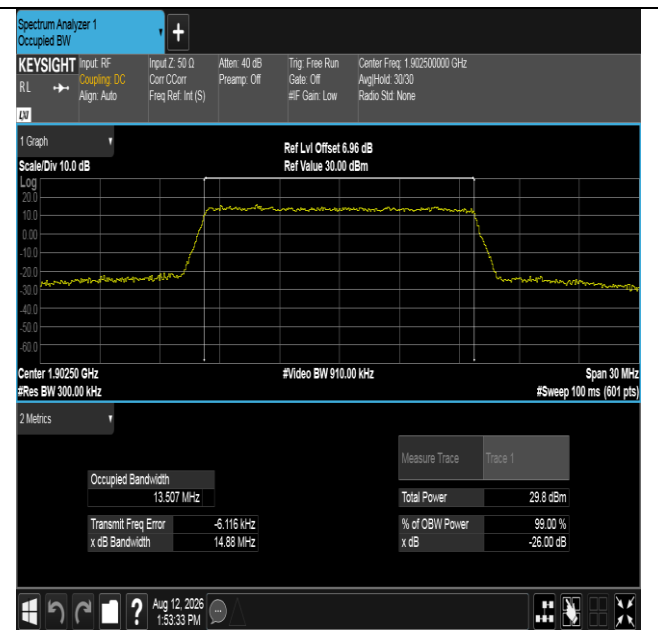
Band2-15MHz-16QAM-19125-75RB#0-PASS
