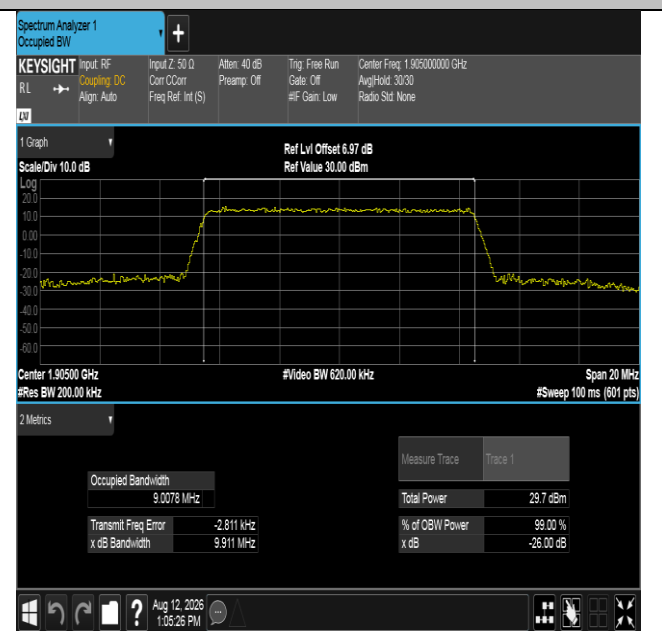
Band2-10MHz-16QAM-19150-50RB#0-PASS
