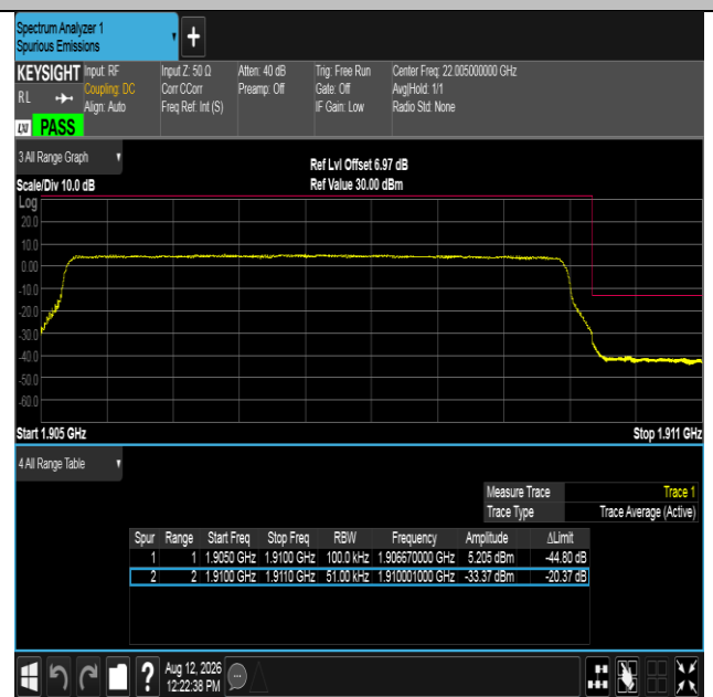
Band2-5MHz-16QAM-19175-25RB#0-PASS
