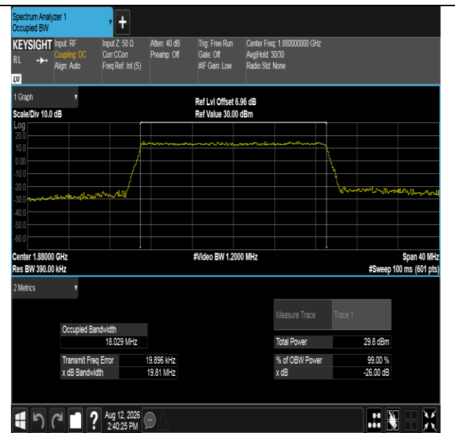
Band2-20MHz-16QAM-18900-100RB#0-PASS
