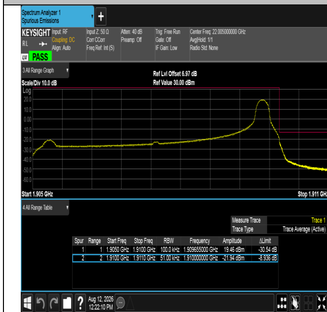
Band2-5MHz-16QAM-19175-1RB#24-PASS
