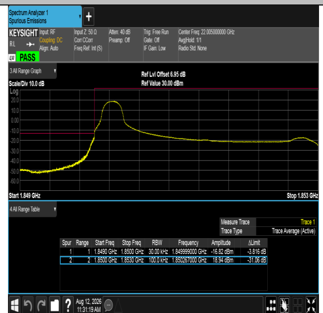
Band2-3MHz-16QAM-18615-1RB#0-PASS
