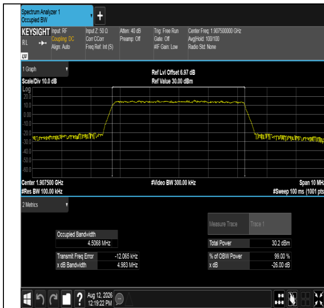
Band2-5MHz-QPSK-19175-25RB#0-PASS
