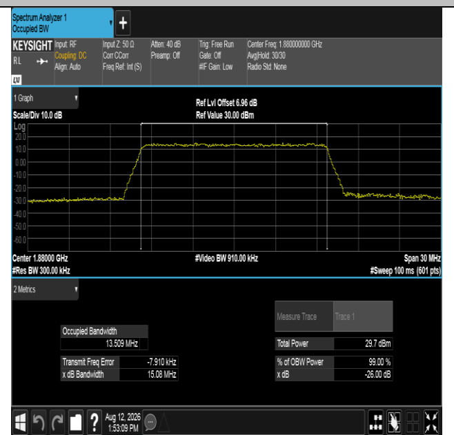
Band2-15MHz-16QAM-18900-75RB#0-PASS
