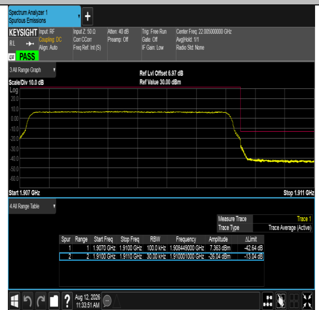
Band2-3MHz-16QAM-19185-15RB#0-PASS
