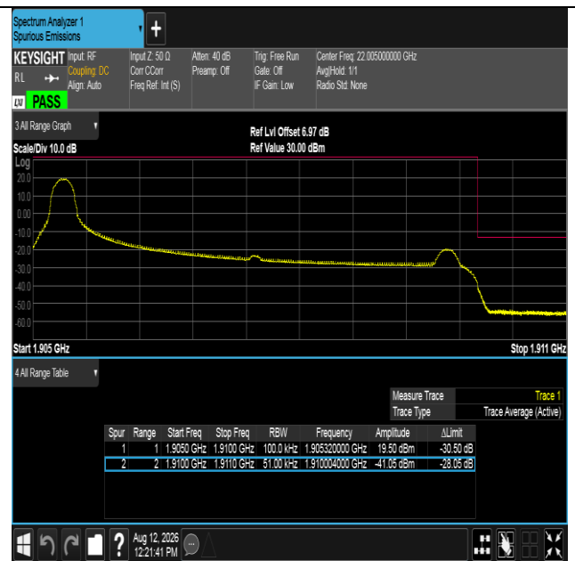
Band2-5MHz-16QAM-19175-1RB#0-PASS
