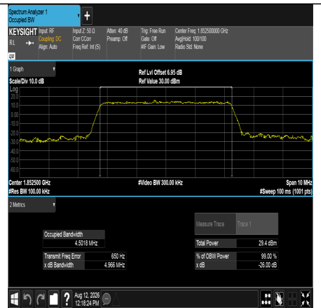
Band2-5MHz-16QAM-18625-25RB#0-PASS
