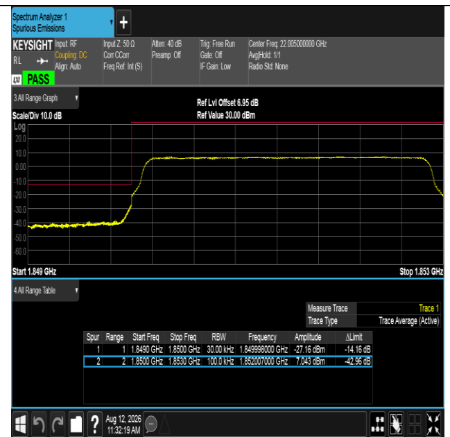
Band2-3MHz-16QAM-18615-15RB#0-PASS
